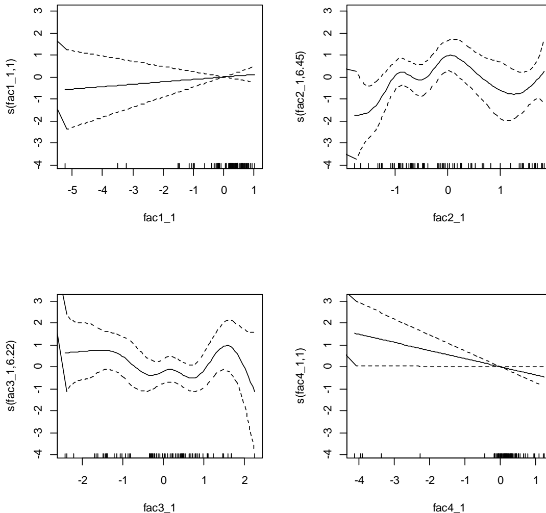
Figure 1: Graph of the non-parametric estimates of each component of the additive model
