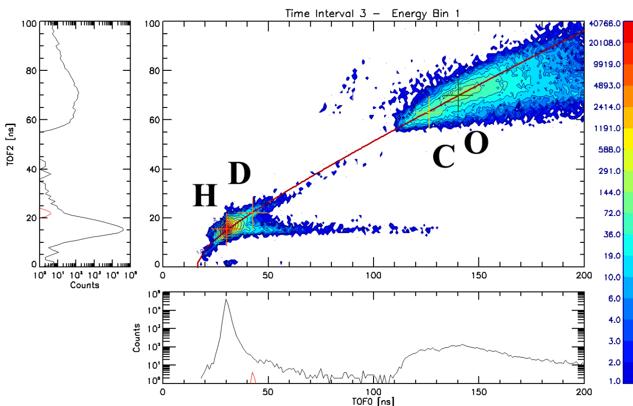
Figure 7. Histogram of triple-coincidence events in the TOF0–TOF2 plane (central panel), with a bin size of 1 ns. The data were collected for energy bin 1 for a time interval near the maximum He flux. The overlaid red line (the mass relation line from the mass equations, see text for details) defines the centre for each species in this plane. It goes through the centres of the peaks of clearly identified species (designated by letters) and the expected position of the D peak. In the leftmost and bottom panels are TOF histograms, which are products of collapse along the TOF2 and TOF0 dimensions, respectively. Red lines in these panels indicate the location and expected amplitude of the D peak to three years of measurements.
