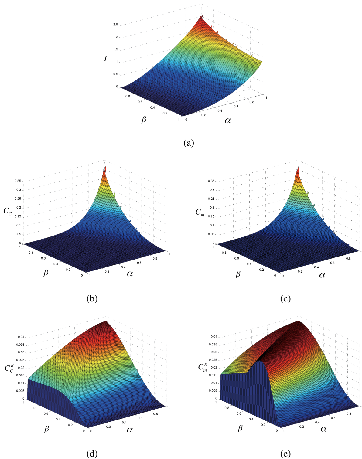
Figure 10. Landscape of complexities I , C_c , C_m , C_c^R , and C_m^R on \alpha - \beta plane. (a): Multi-information I ; (b): Cuboid-bias complexity C_c . (c): Modular complexity C_m ; (d): Regularized cuboid-bias complexity C_c^R ; (e): Regularized modular complexity C_m^R . All complexity measures show the complementarity intersecting with each other, satisfying the boundary conditions vanishing at \alpha = 0 and \beta = 0 except the multi-information I . Note that regularized complexities C_c^R and C_m^R show singularity of convergence at \alpha \rightarrow 0 due to the regularization of infinitesimal value.
