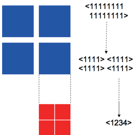
Figure 8. Example of 16-node system \langle 11 \cdots 1 \rangle that has different levels of modularity. The four 4-node subsystems \langle 1111 \rangle (blue blocks) are loosely connected and easy to be decomposed, while inside each component (red blocks) is tightly connected. The degree of connection represents statistical dependency or edge information between subsystems. Such hierarchical structure can be detected by observing the decomposition path of the modular complexity C_m .
