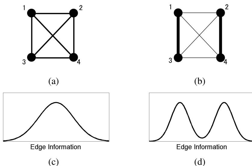
Figure 2. Schematic examples of stochastic systems with identical multi-information I where complexity measures with arithmetic mean fail to distinguish. (a): Example 1 of stochastic system with homogeneous mean of edge information and symmetric fluctuation of its heterogeneity; (b): Example 2 of heterogeneous stochastic system with bimodal edge information distribution and identical multi-information I and complexity based on arithmetic mean as example 1; (c): schematic representation of the distribution of statistical association (edge information) in upper network; (d): schematic representation of the distribution of statistical association (edge information) in upper network.
