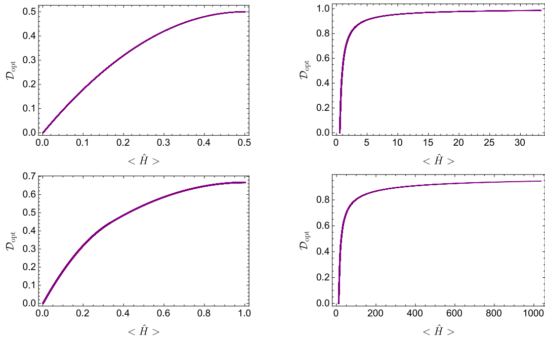
Figure 6. \mathcal{D}_{\text{opt}} as a function of \langle \hat{H} \rangle for different quantum systems: ( Top left ) a single-qubit system with (dimensionless) energy levels 0, 1; ( Top right ) a d -level harmonic oscillator with (dimensionless) energy levels E_n = n + (1/2) ; ( Bottom left ) a two-qubit system with accessible (dimensionless) energies: 0, 1, 2; and ( Bottom right ) a Gaussian wave packet in an infinite square well, with (dimensionless) energy levels E_n = \pi^2 n^2 . All these systems are those studied in Section 3.
