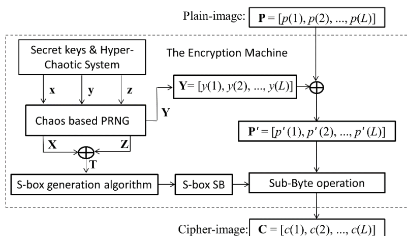
Figure 4. Sketch of the original encryption algorithm.
