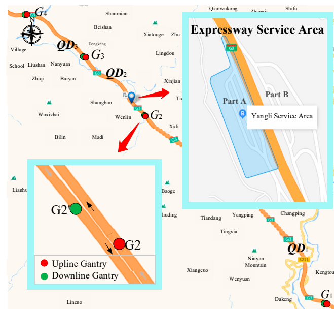
Figure 2. Visualization of ETC gantries and ESA locations.
