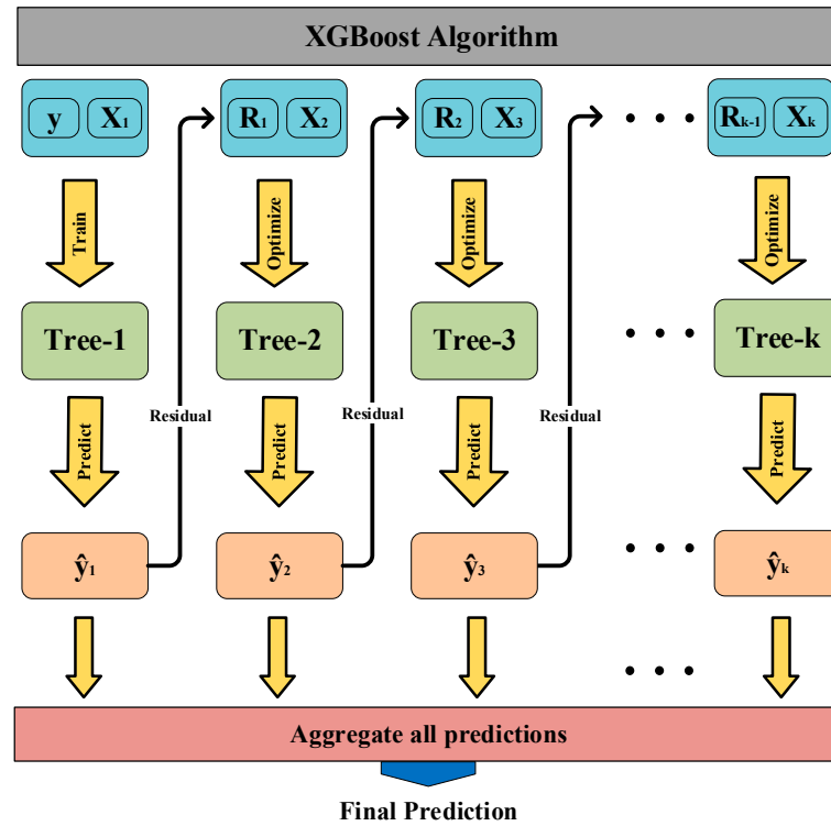
Figure 3. XGBoost Schematic.
