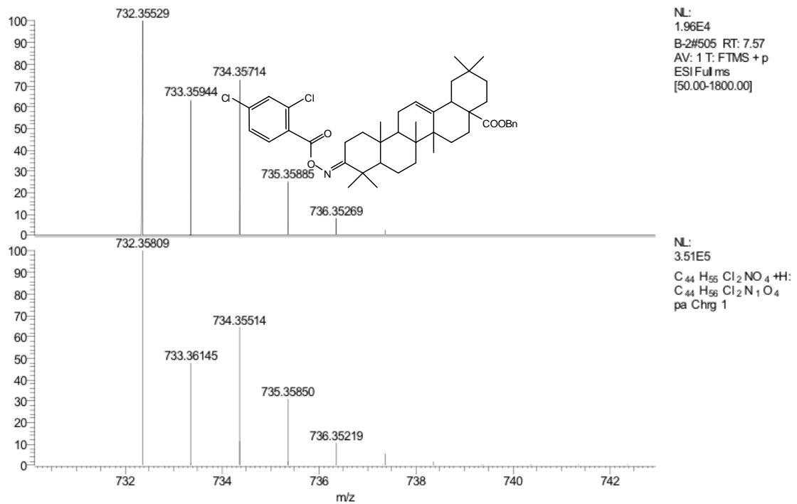
Figure S36. HRMS of compound B-02.
