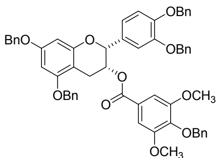
Figure S3. 5,7,3',4',4''-penta- O -benzyl-3- O -(3'',5''-dimethoxybenzoyl)-epicatechin ( 11b ).
