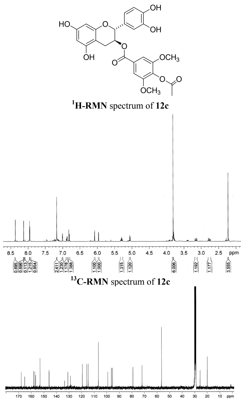
Figure S5. Spectra of 3- O -(4-acetoxy-3,5-dimethoxybenzoyl)-catechin ( 12c ).
