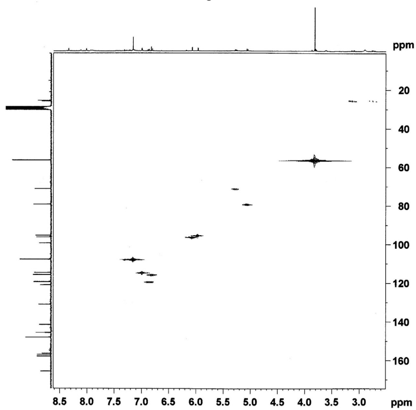
HMQC-RMN spectrum of 12b
