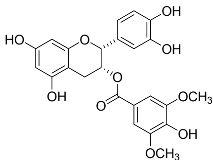
Figure S7. Spectra of 3-O-(4-hydroxy-3,5-dimethoxybenzoyl)-epicatechin (13b).
