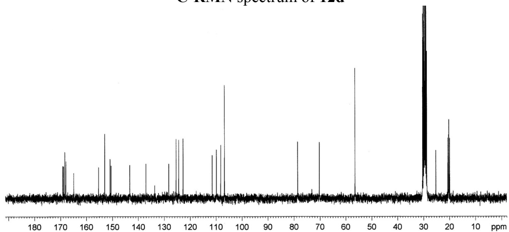
HMQC-RMN spectrum of 12d
