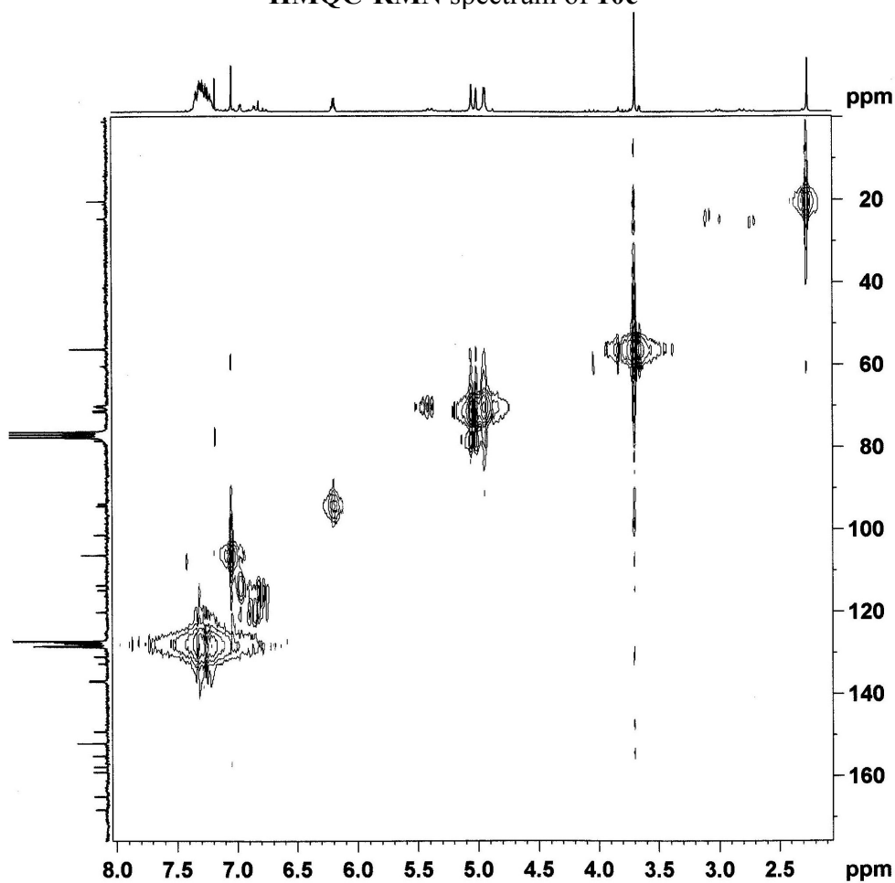
HMQC-RMN spectrum of 10c
