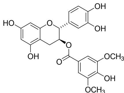
Figure S4. Spectra of 3- O -(4-hydroxy-3,5-dimethoxybenzoyl)-catechin ( 12b ).
