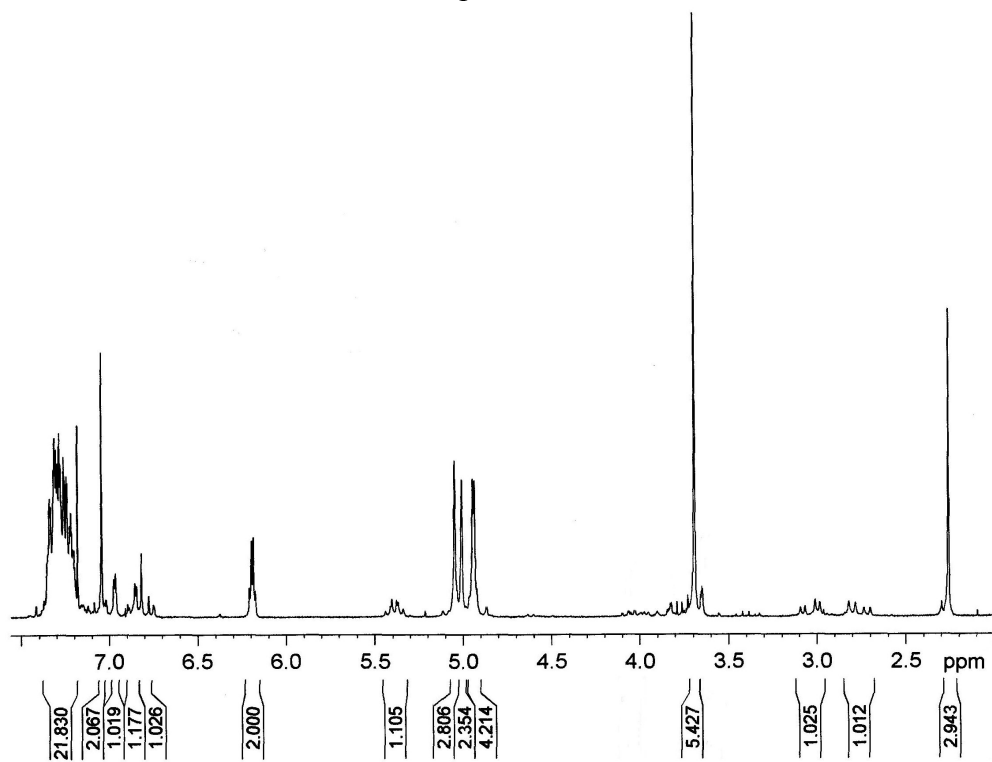
1 H-RMN spectrum of 10c
