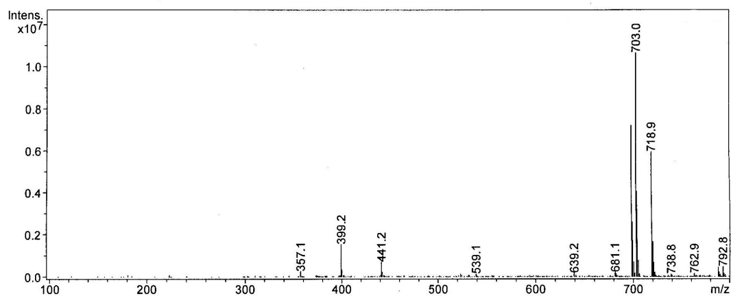
Figure S7. Spectra of 3-O-(4-hydroxy-3,5-dimethoxybenzoyl)-epicatechin (13b).
