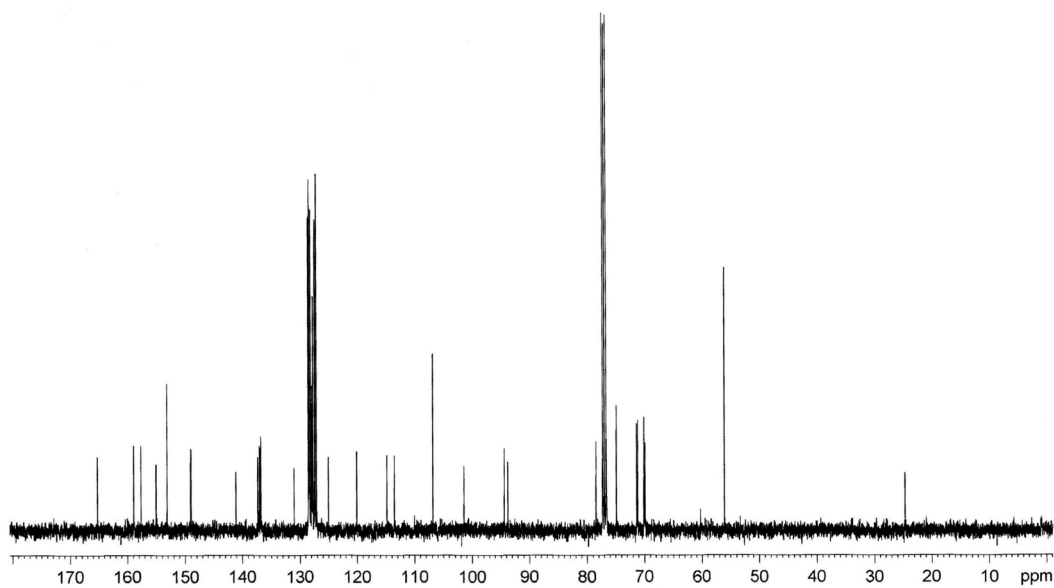
13 C-RMN spectrum of 10b
