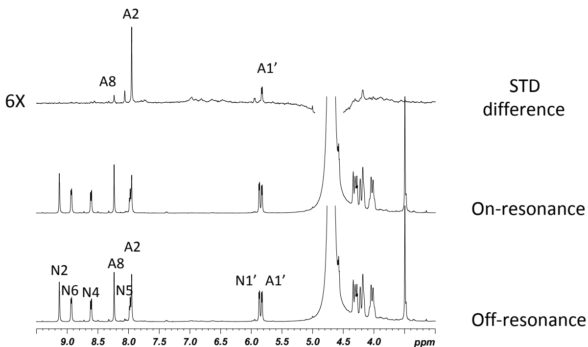
Figure S2. FNR-NADP STD experiment (top), on-resonance (middle) and off-resonance (bottom).
