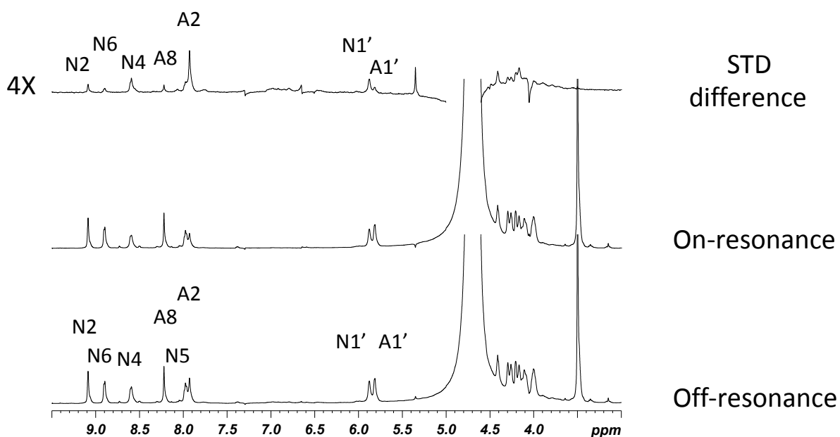
Figure S2. FNR-NADP STD experiment (top), on-resonance (middle) and off-resonance (bottom).
