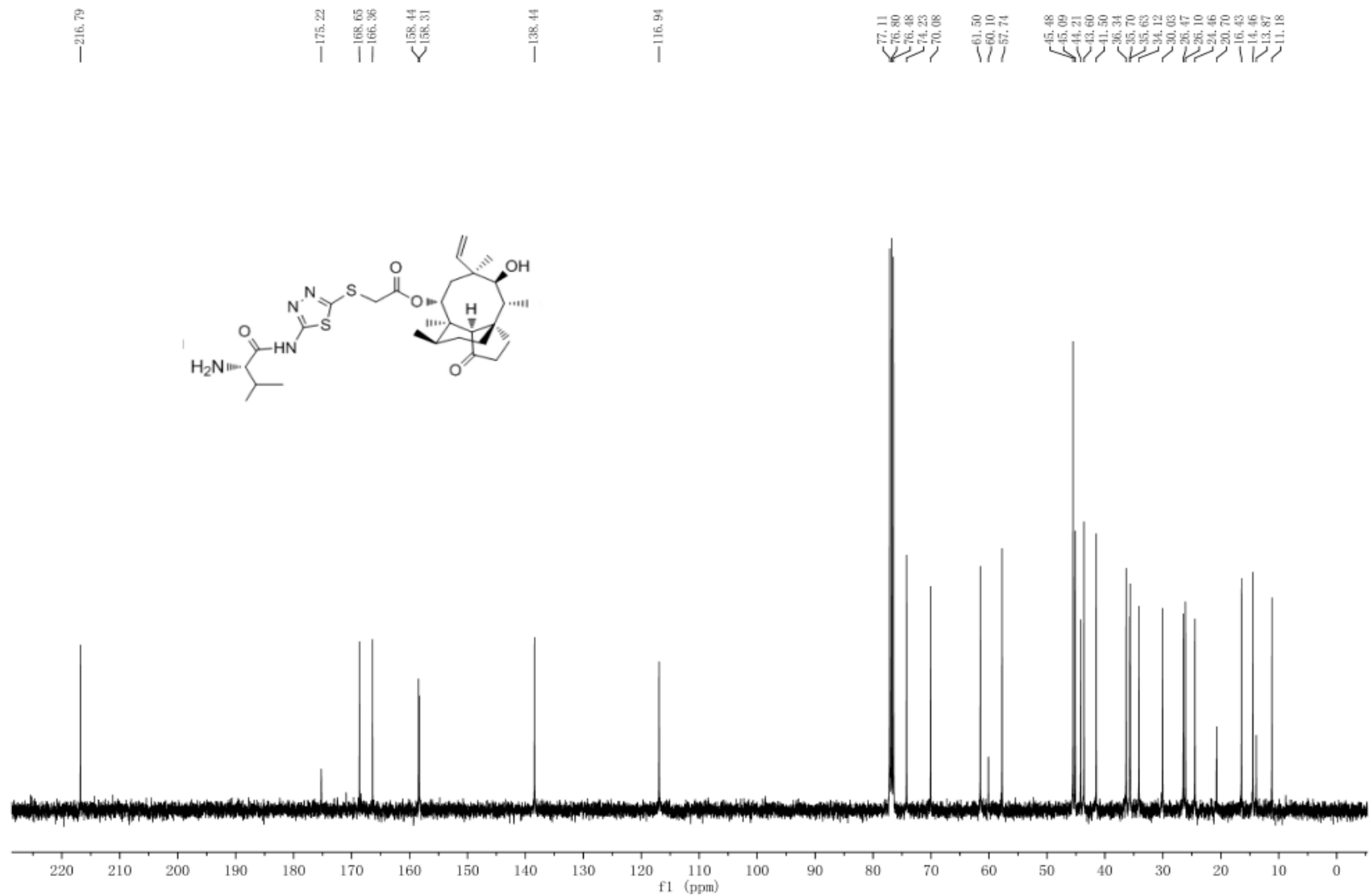
Figure S24. ^{13}\text{C} NMR spectrum of compound 6b.
