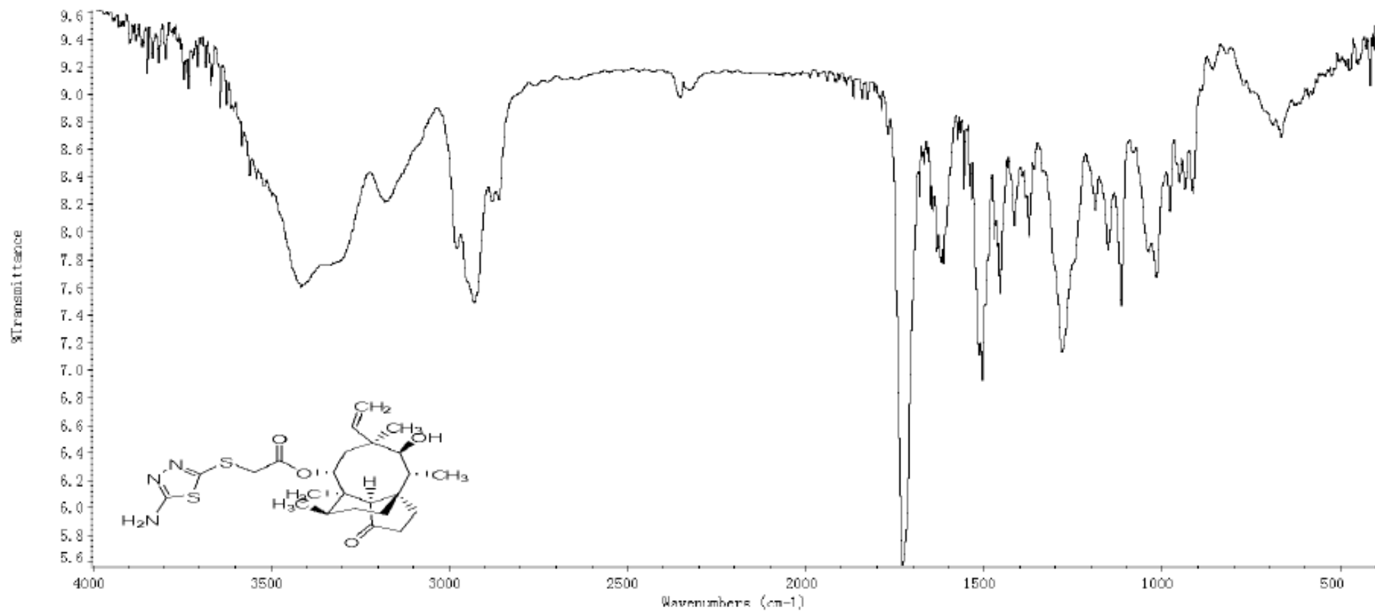
Figure S7. IR spectrum of compound 4.
