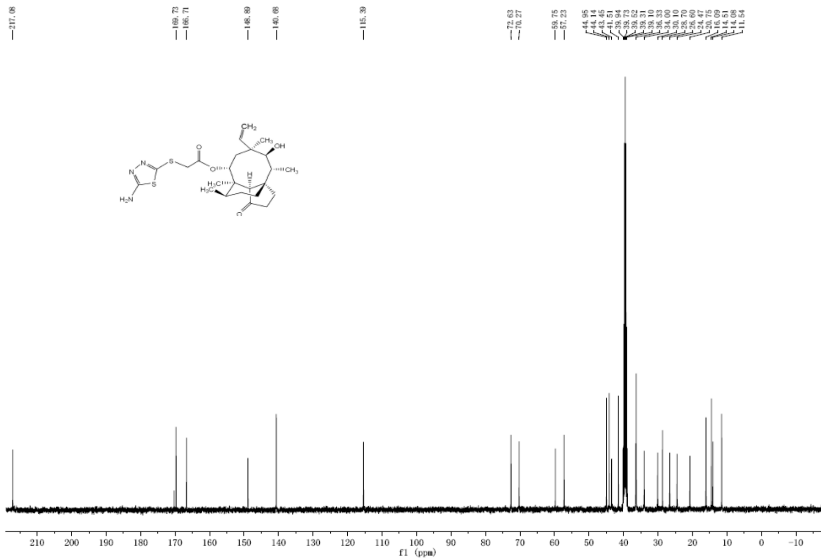
Figure S9. ^{13}\text{C} -NMR spectrum of compound 4.
