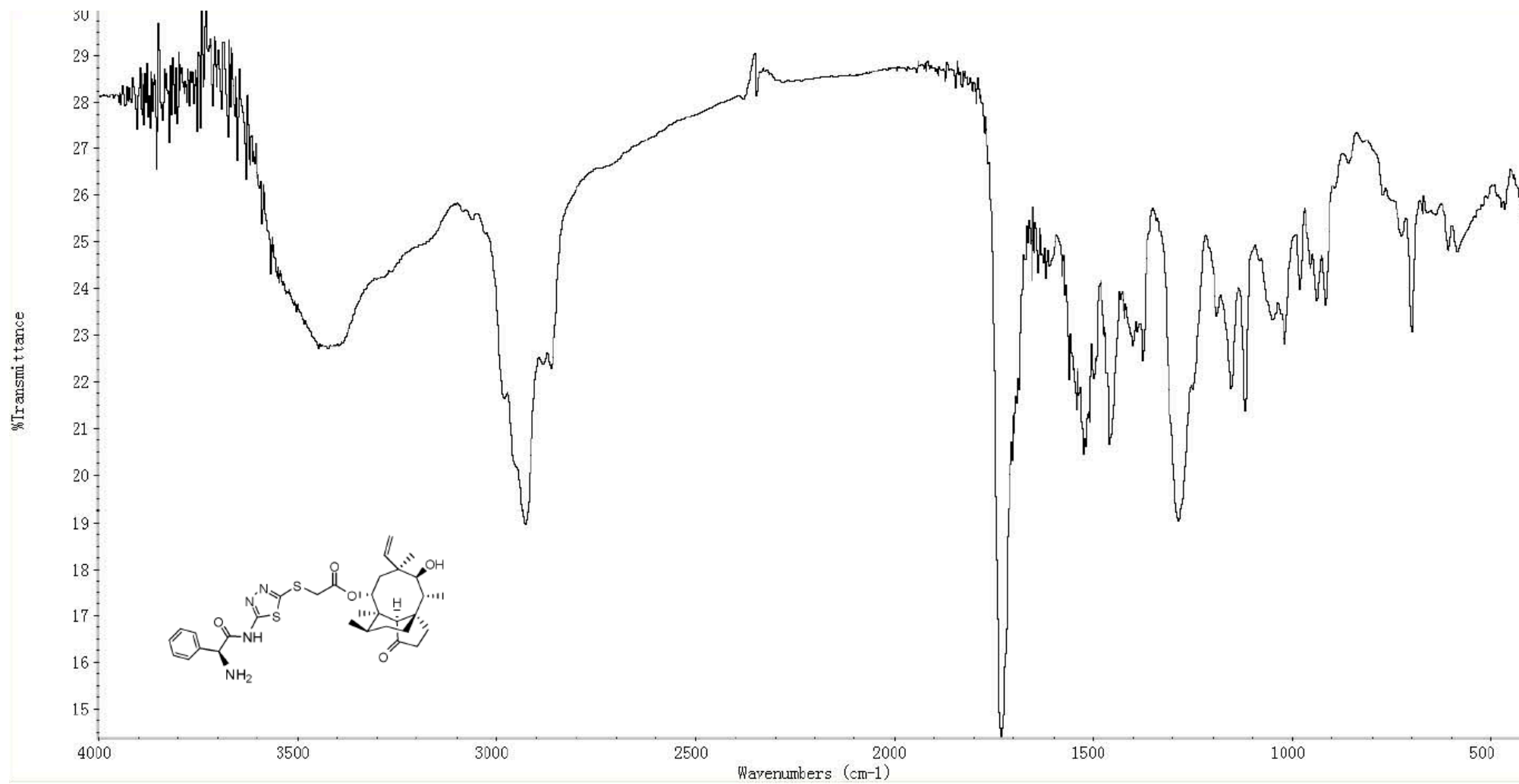
Figure S25. IR spectrum of compound 6c.
