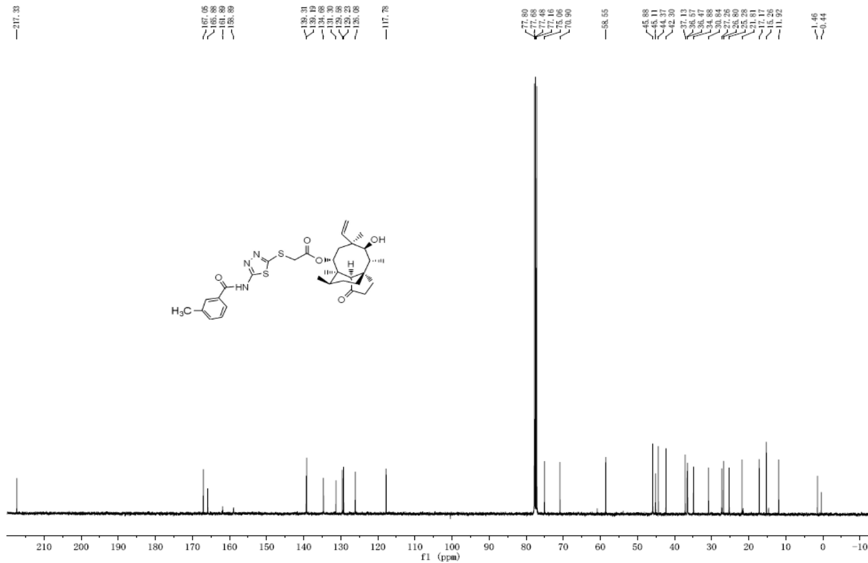
Figure S15. ^{13}\text{C} NMR spectrum of compound 5b.
