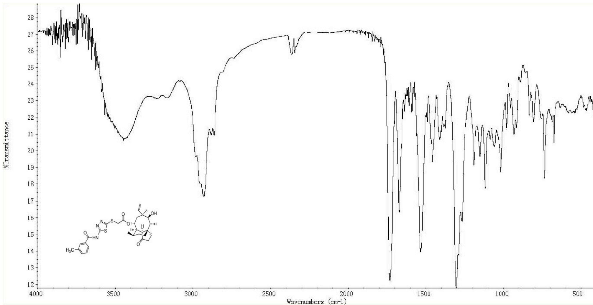
Figure S13. IR spectrum of compound 5b.
