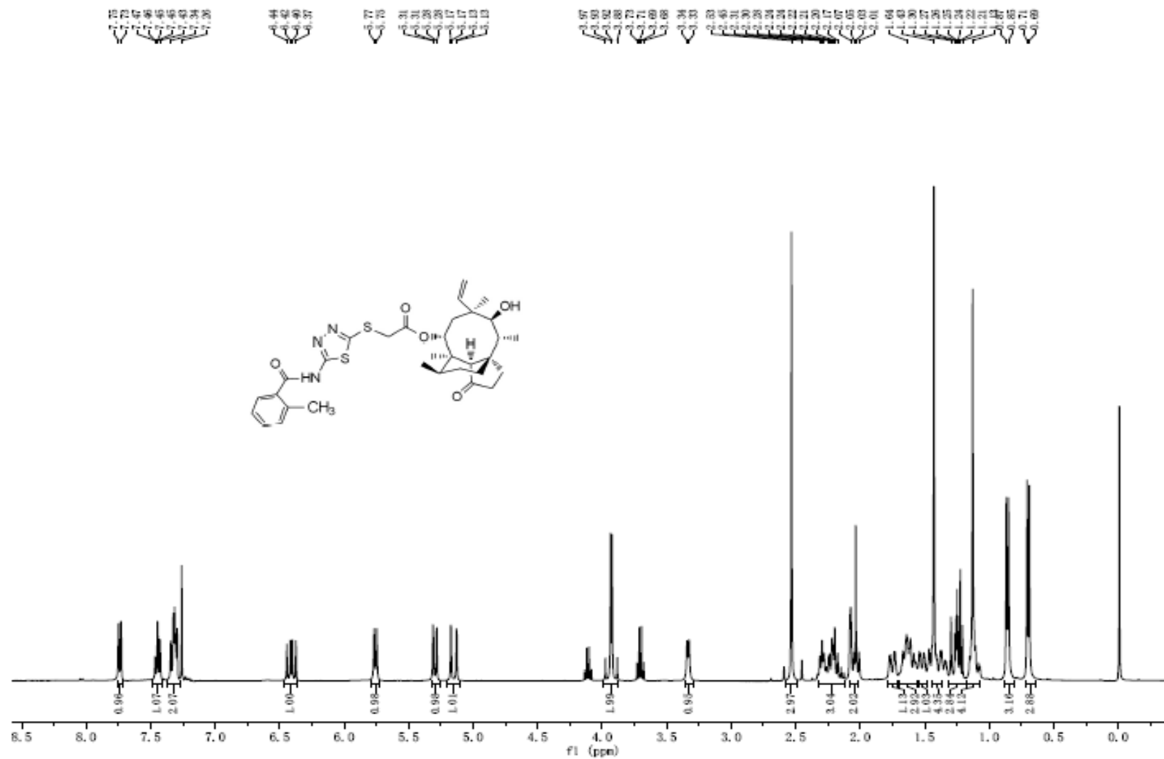
Figure S11. ^1\text{H} NMR spectrum of compound 5a.
