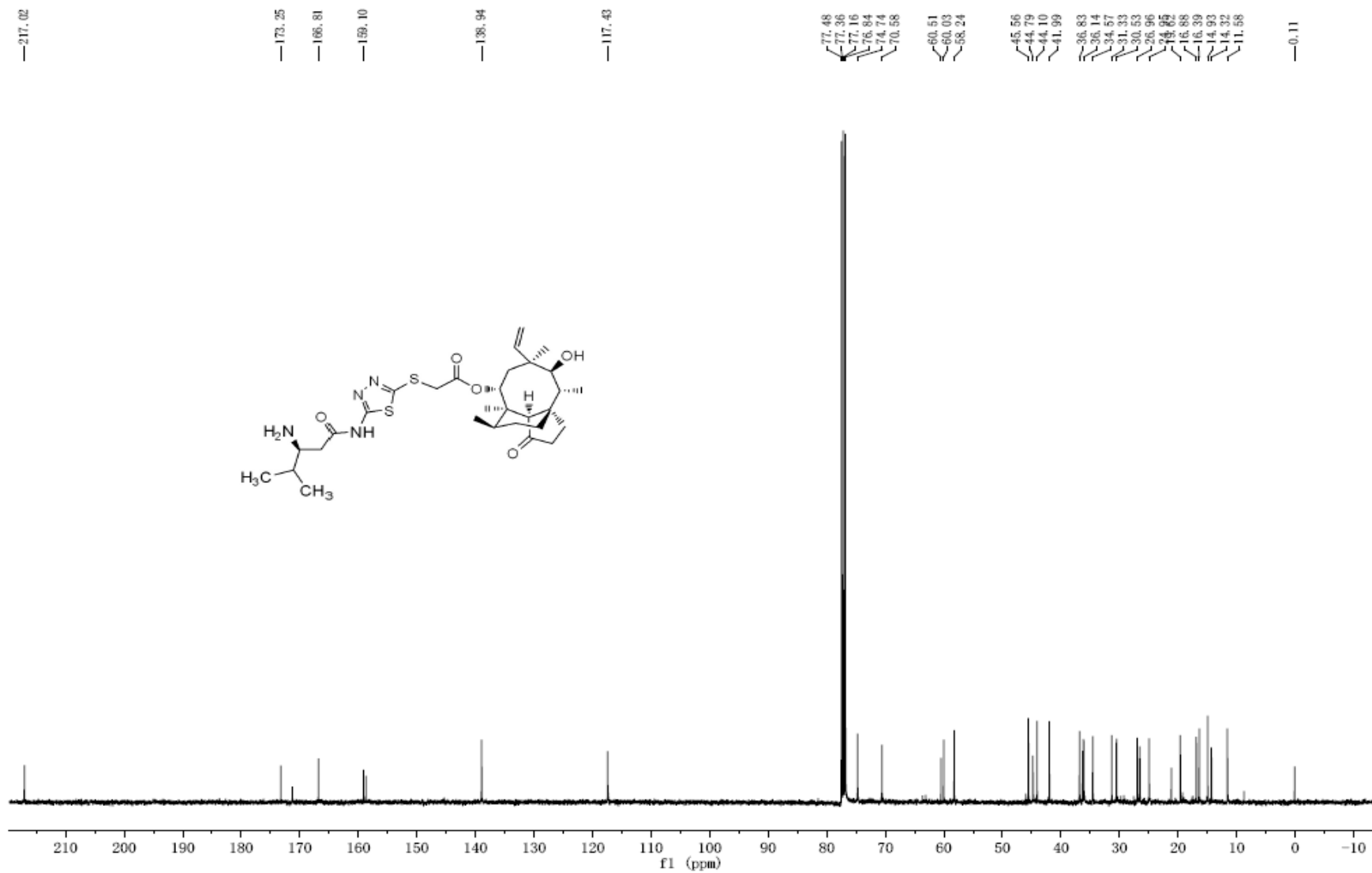
Figure S21. ^{13}\text{C} NMR spectrum of compound 6a.
