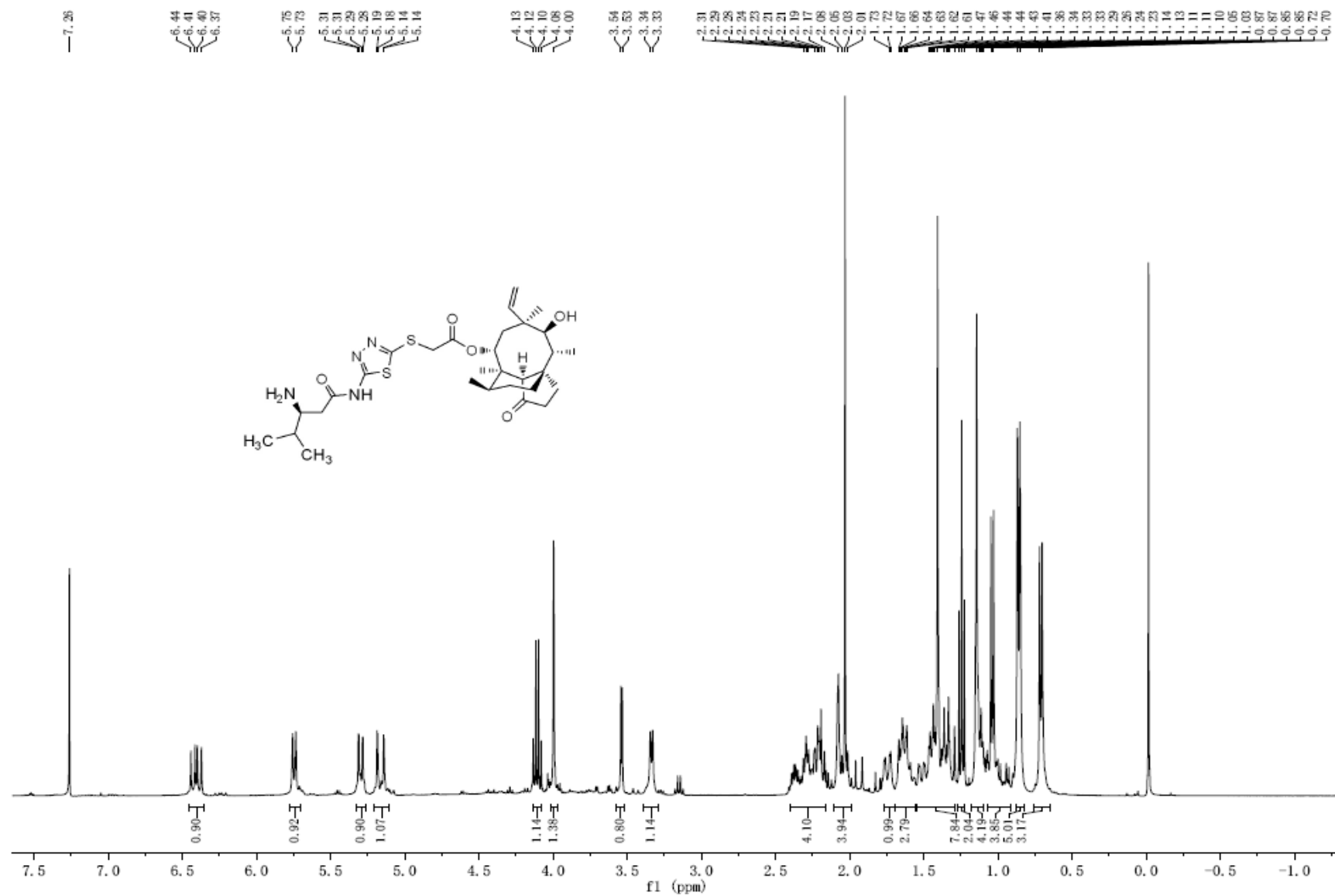
Figure S20. 1 H NMR spectrum of compound 6a.
