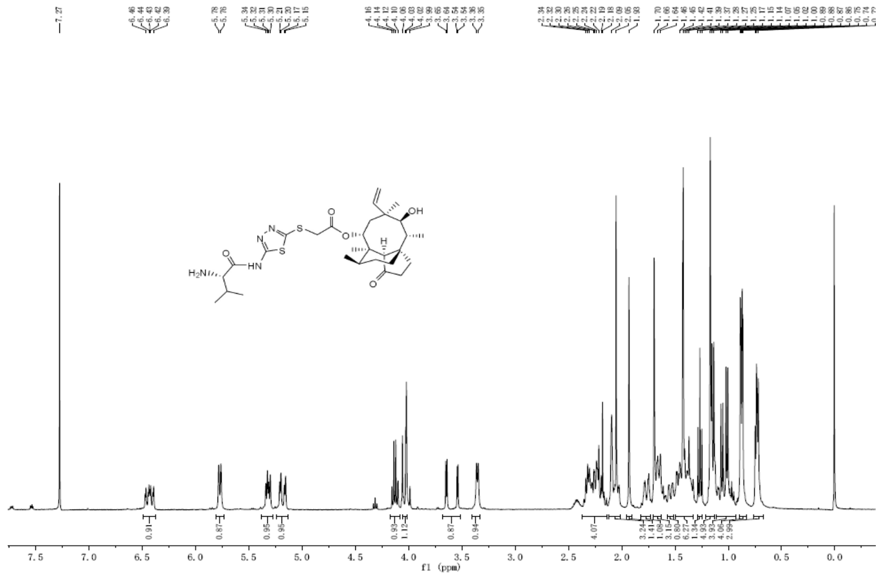
Figure S23. 1 H NMR spectrum of compound 6b.
