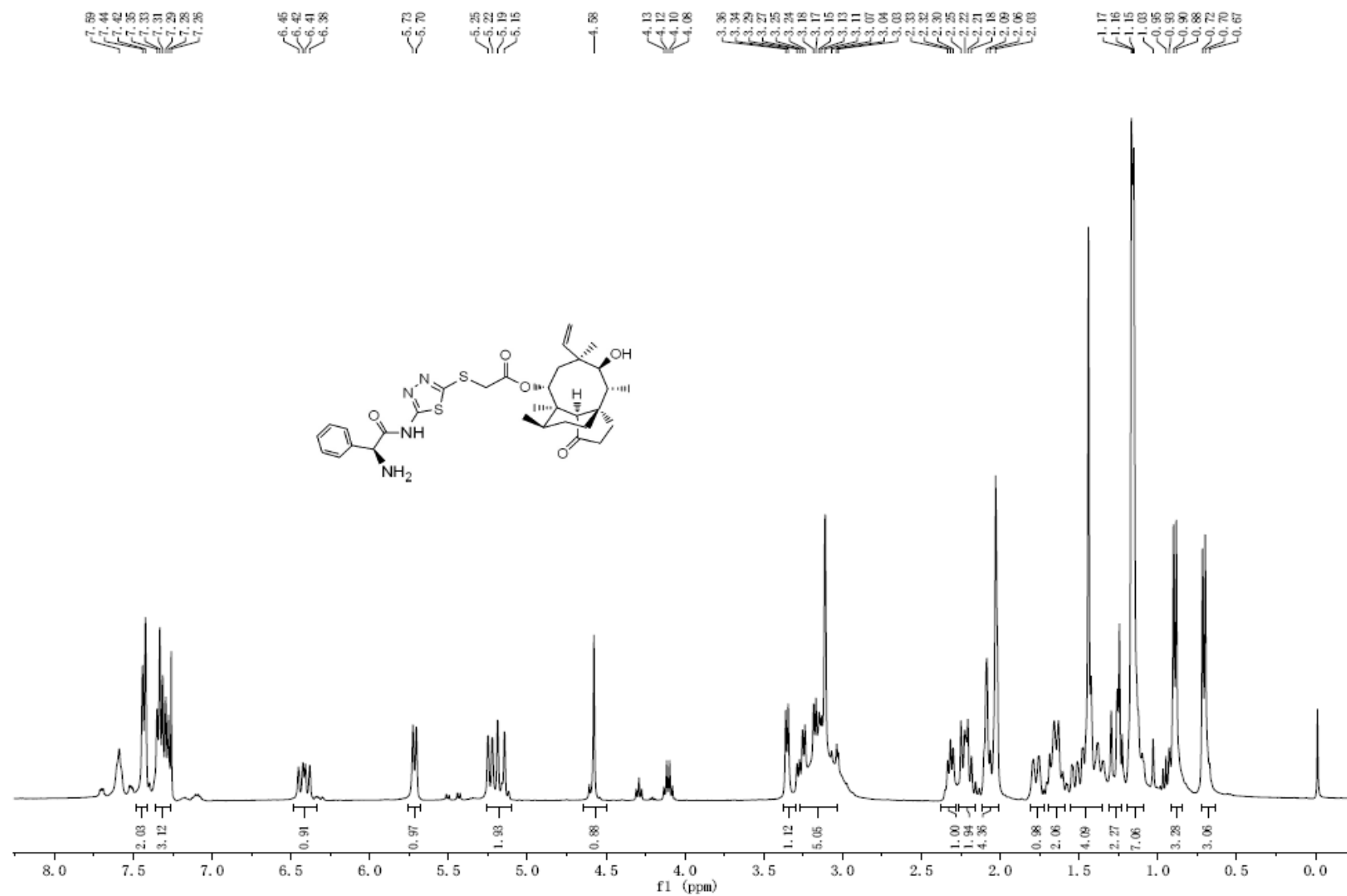
Figure S26. ^1\text{H} NMR spectrum of compound 6c.
