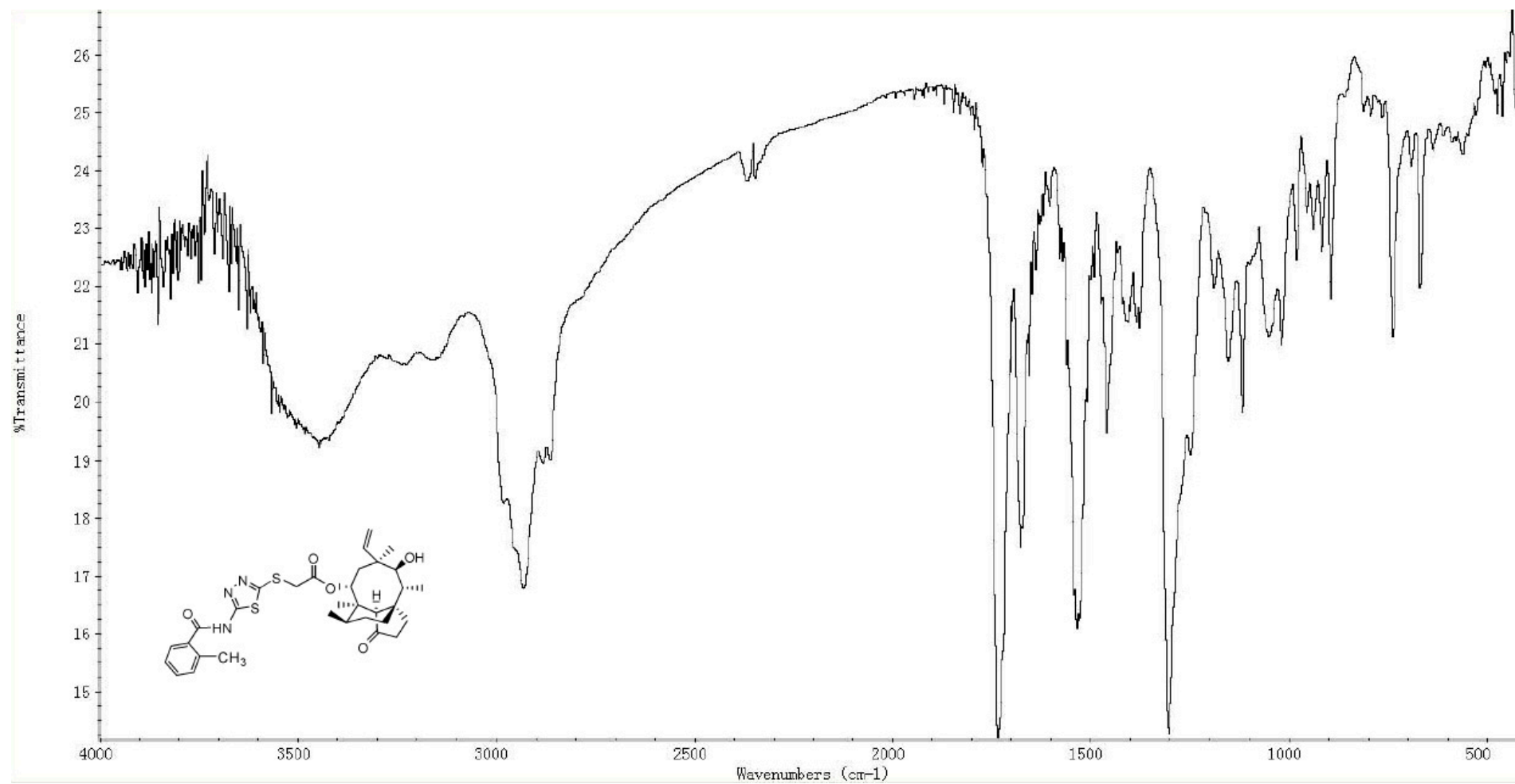
Figure S10. IR spectrum of compound 5a.
