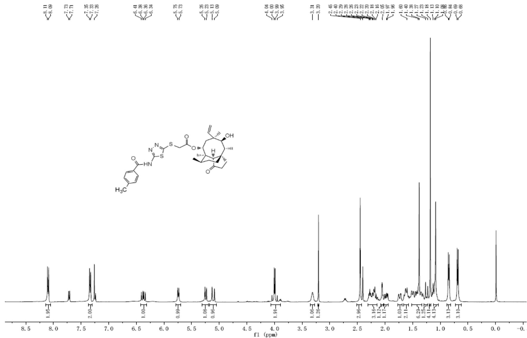
Figure S17. 1 H-NMR spectrum of compound 5c.
