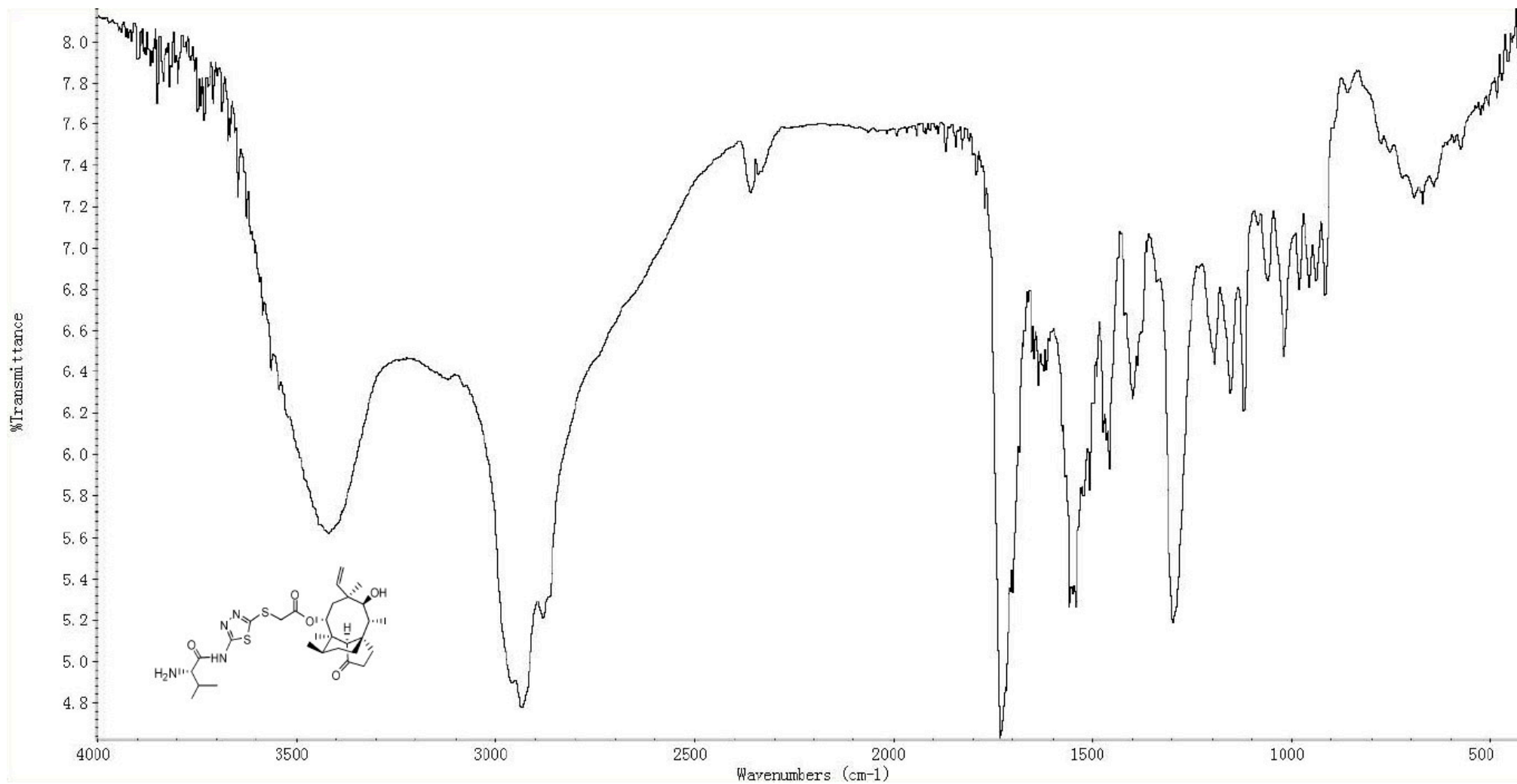
Figure S22. IR spectrum of compound 6b.
