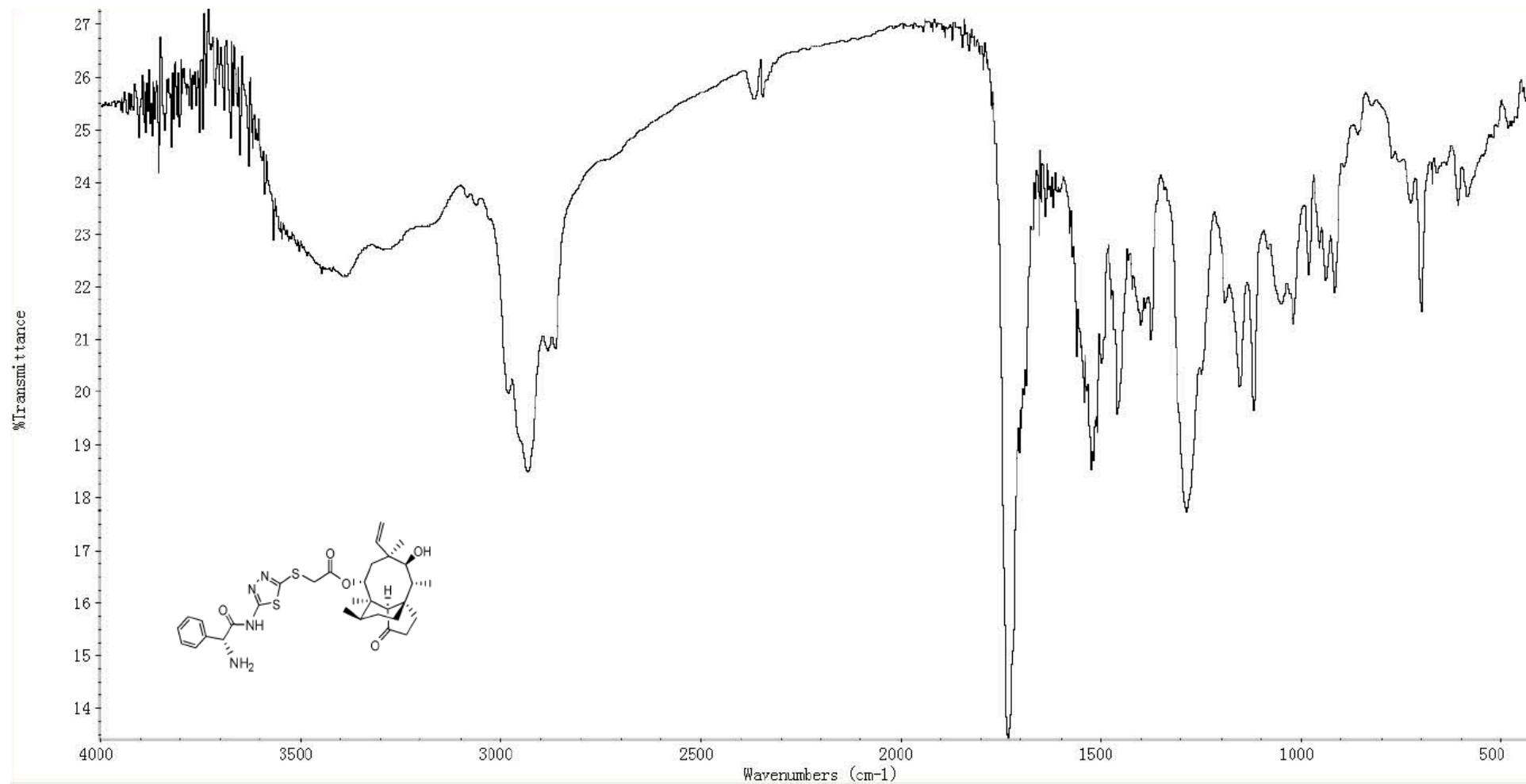
Figure S28. IR spectrum of compound 6d.
