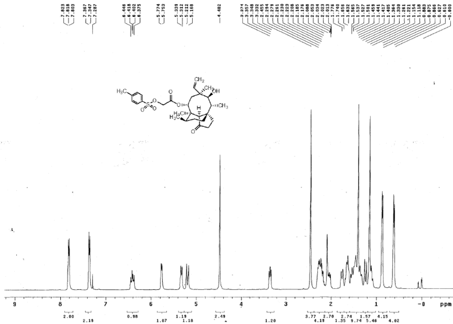
Figure S2. 1 H-NMR spectrum of compound 2.
