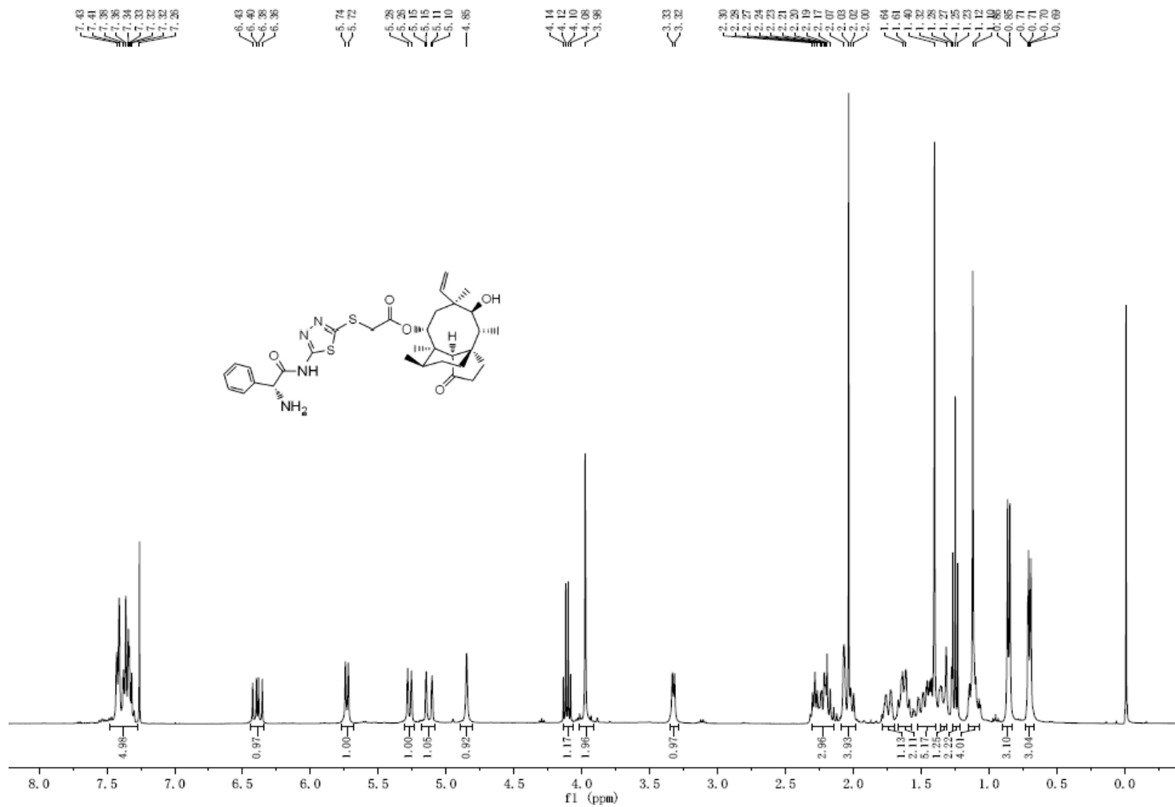
Figure S29. ^1\text{H} NMR spectrum of compound 6d.
