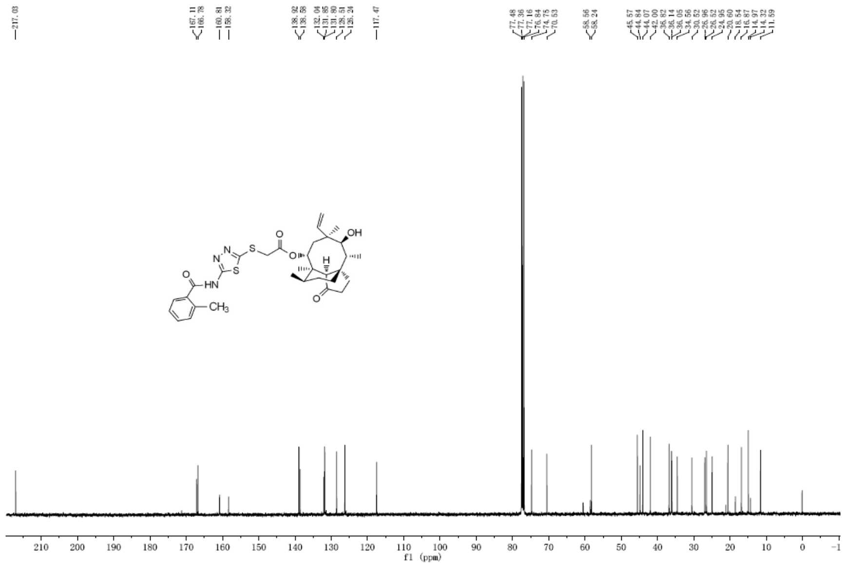
Figure S12. ^{13}\text{C} -NMR spectrum of compound 5a.
