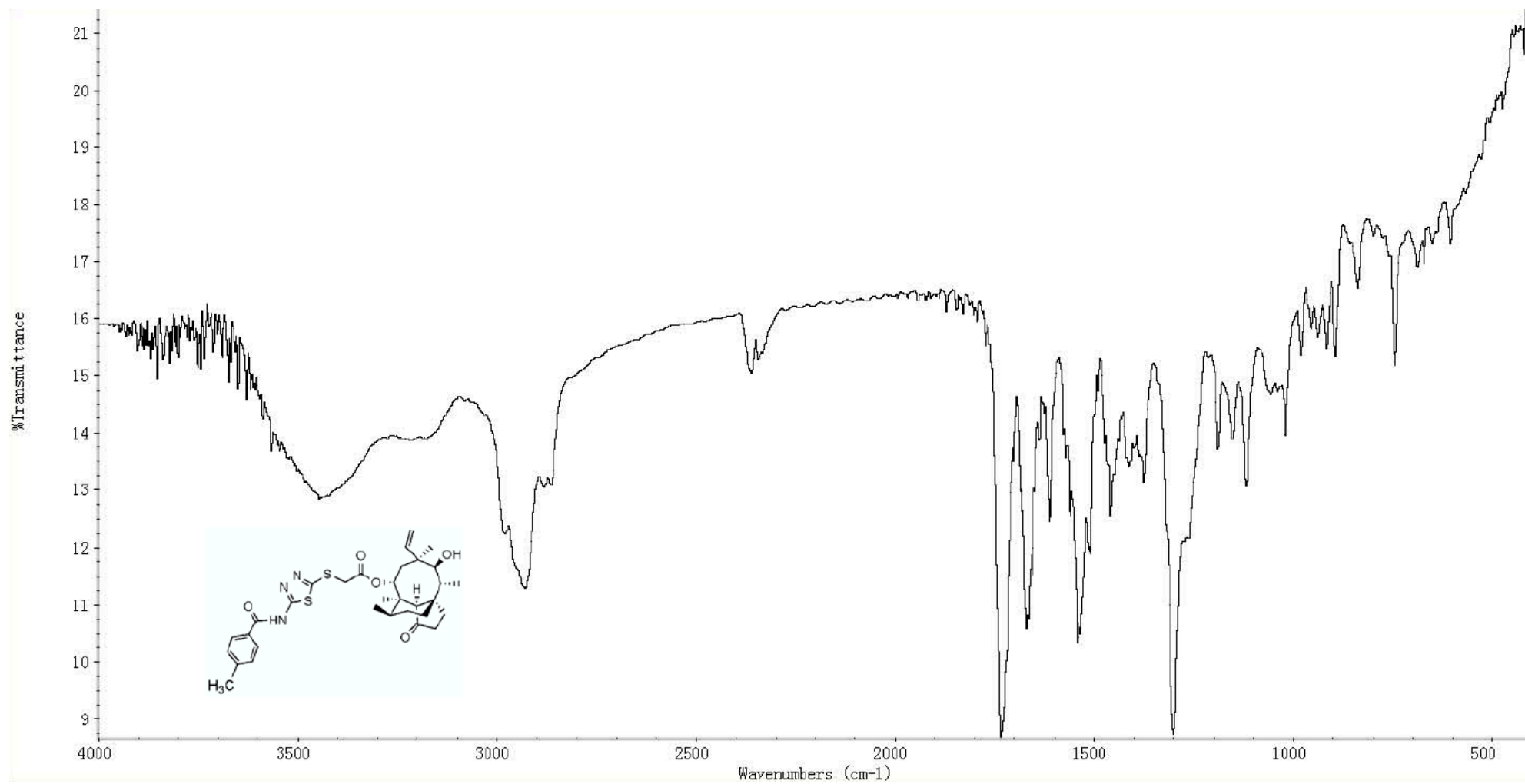
Figure S16. IR spectrum of compound 5c.
