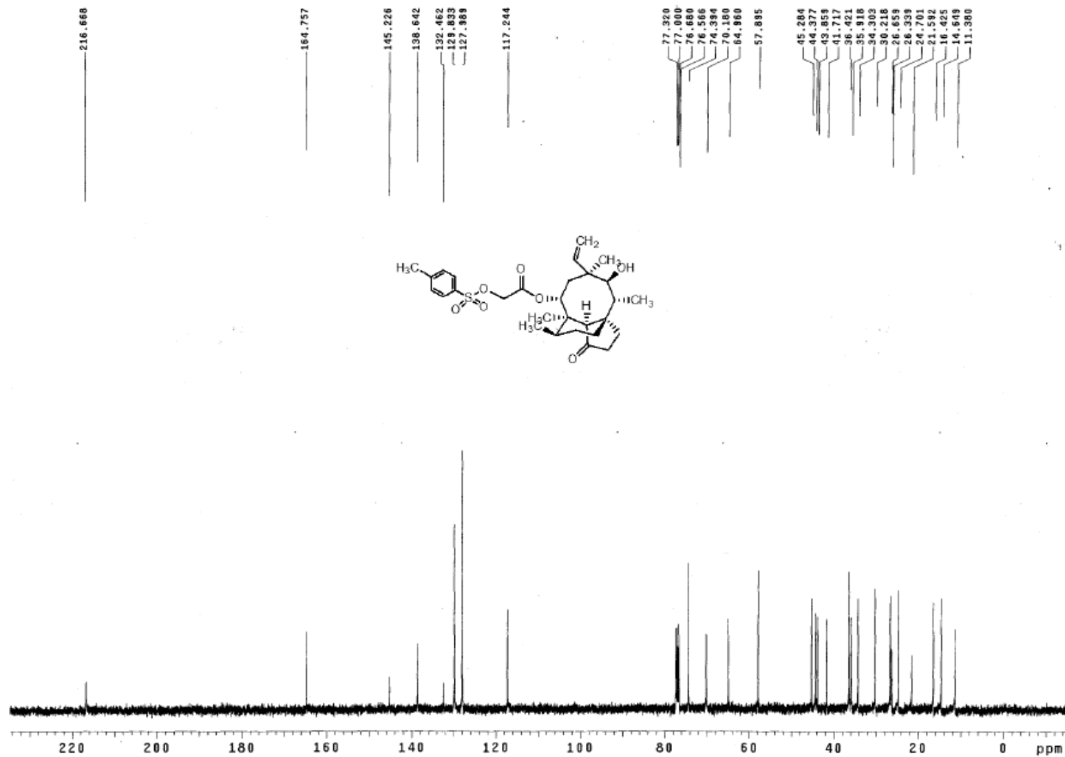
Figure S3. ^{13}\text{C} -NMR spectrum of compound 2.
