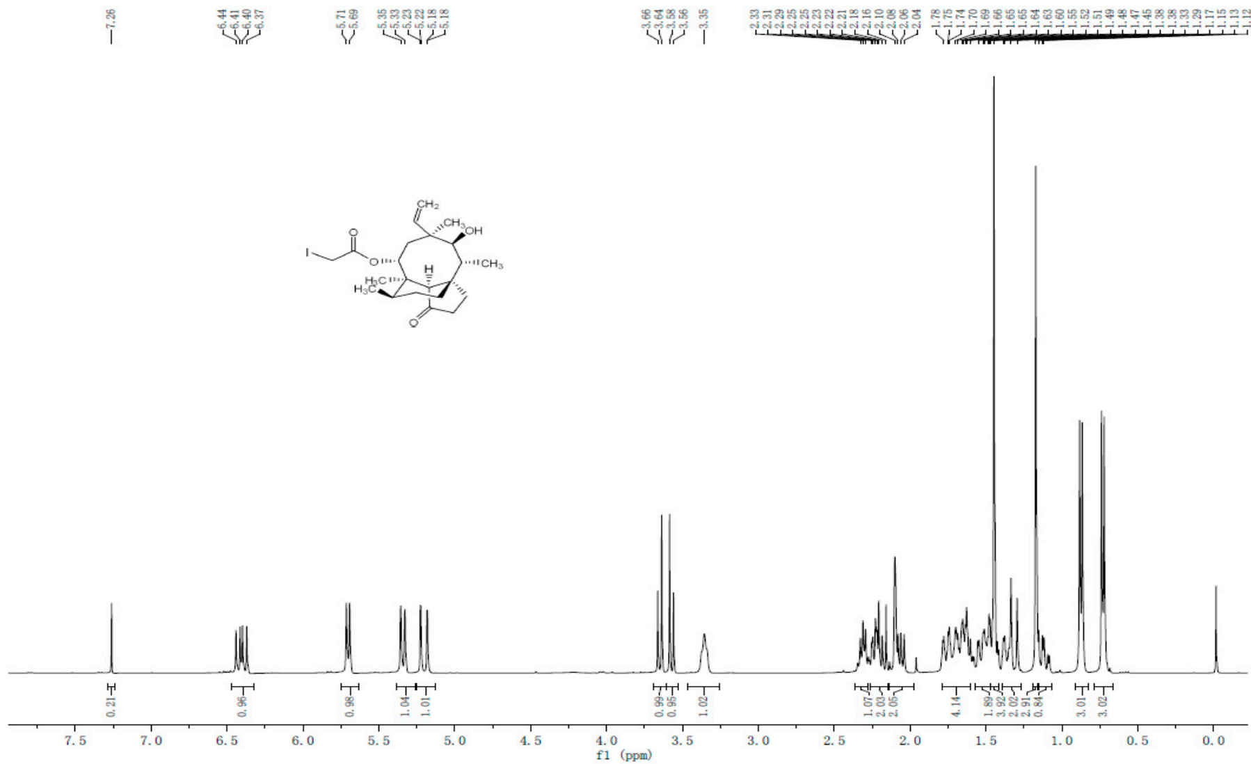
Figure S5. ^1\text{H-NMR} spectrum of compound 3.
