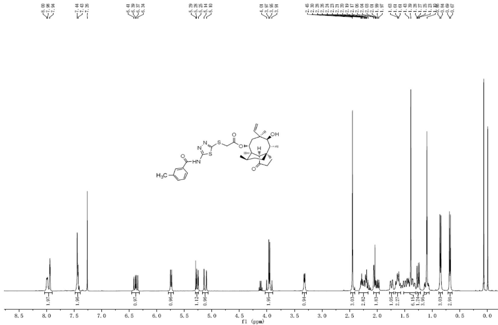
Figure S14. 1 H-NMR spectrum of compound 5b.
