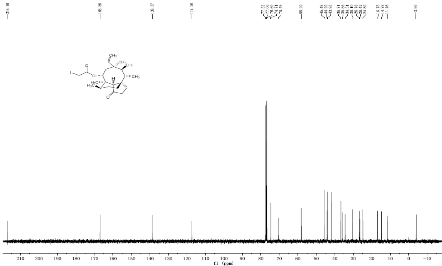
Figure S6. ^{13}\text{C} -NMR spectrum of compound 3.
