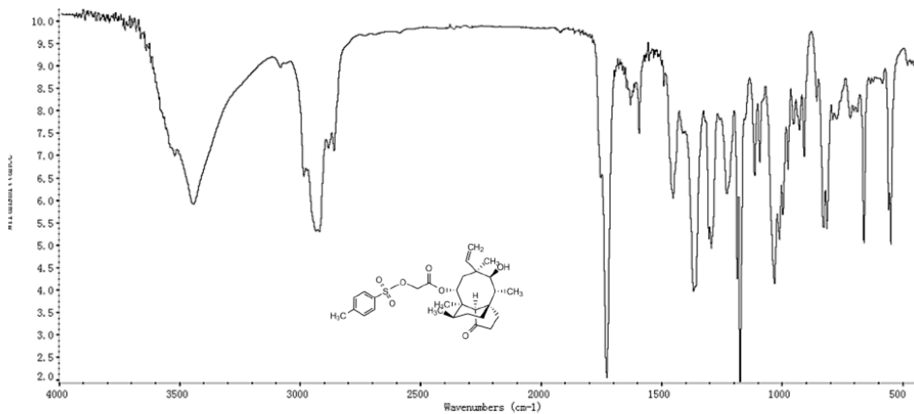
Figure S1. IR spectrum of compound 2.
