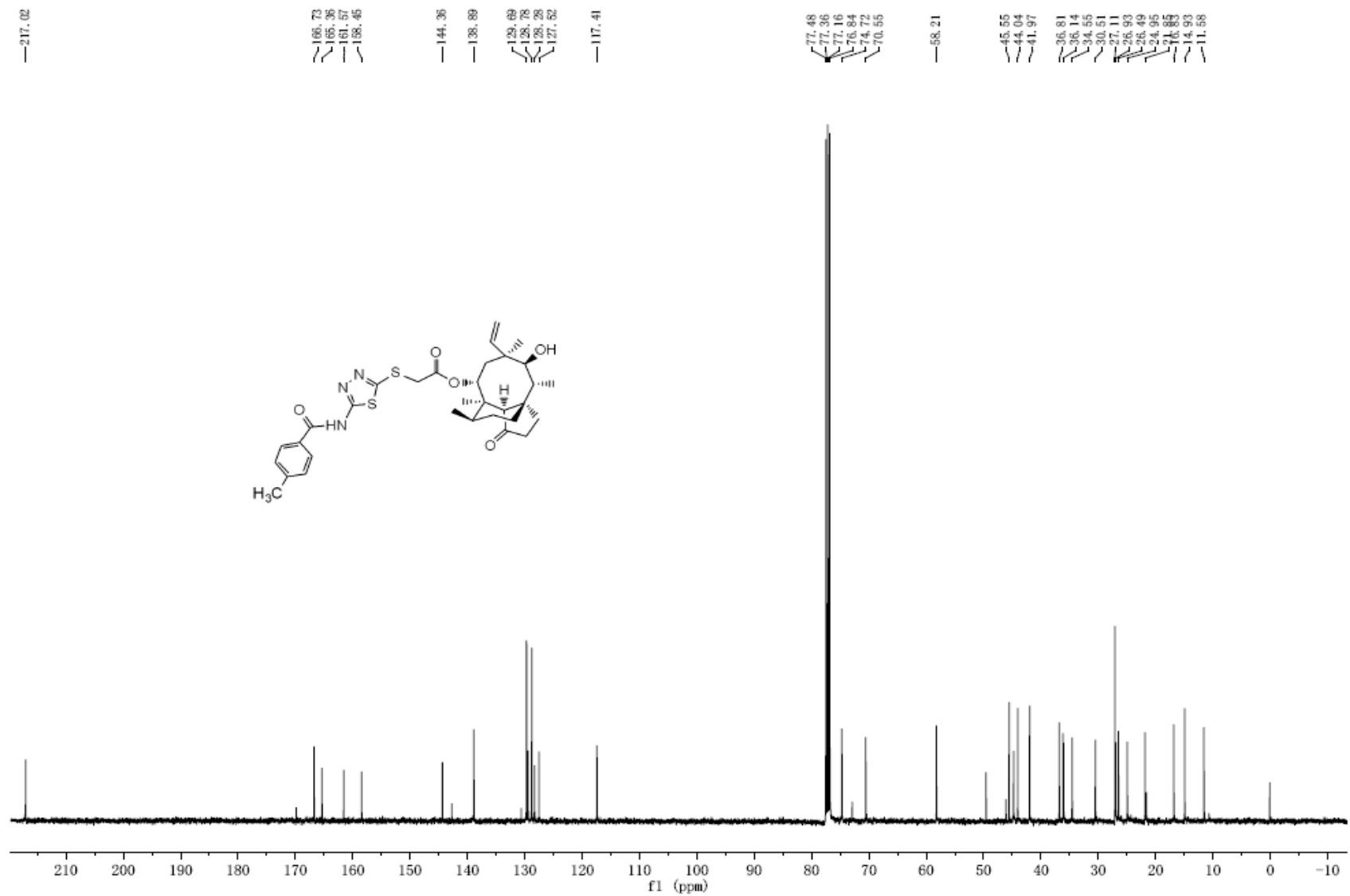
Figure S18. ^{13}\text{C} NMR spectrum of compound 5c.
