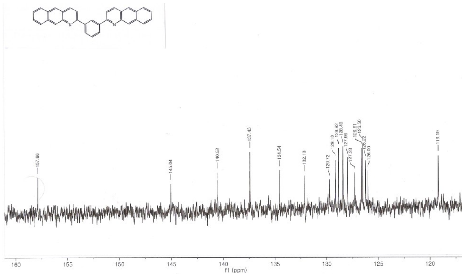
Figure S4. ^{13}\text{C} -NMR of 3c.
