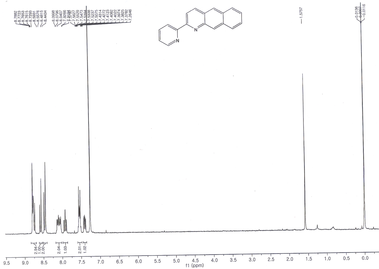
Figure S1. ^1\text{H-NMR} of 3ab .
