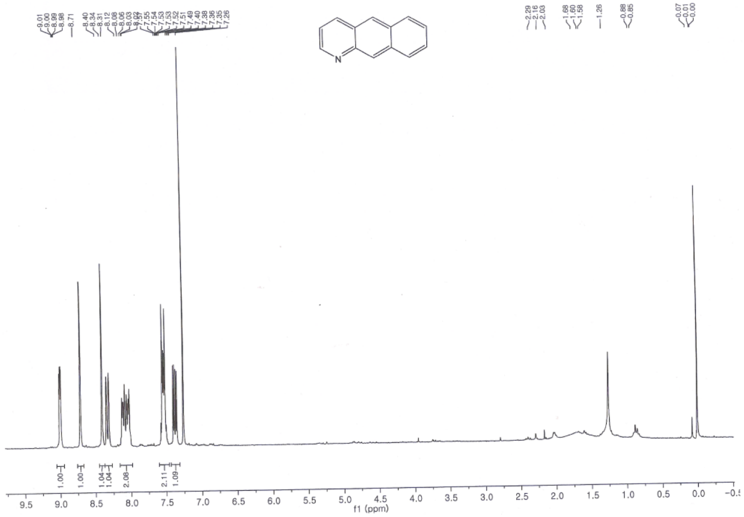
Figure S6. ^1\text{H-NMR} of 4.
