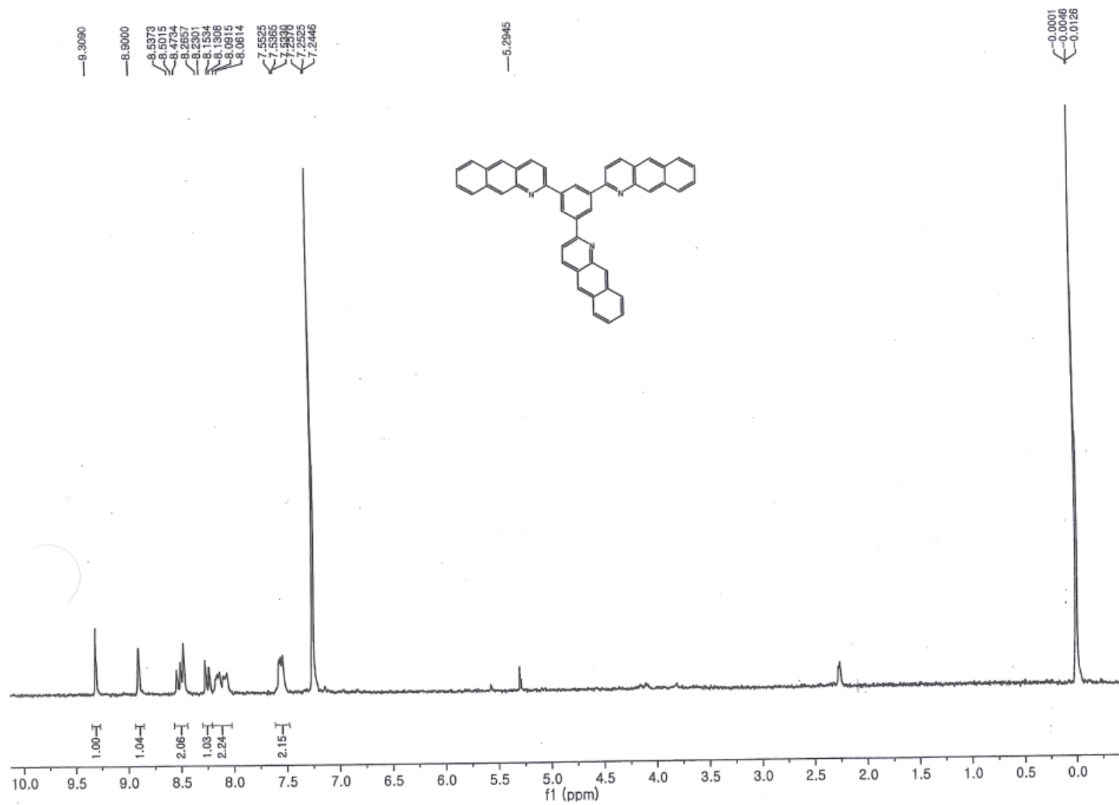
Figure S5. ^1\text{H-NMR} of 3e.
