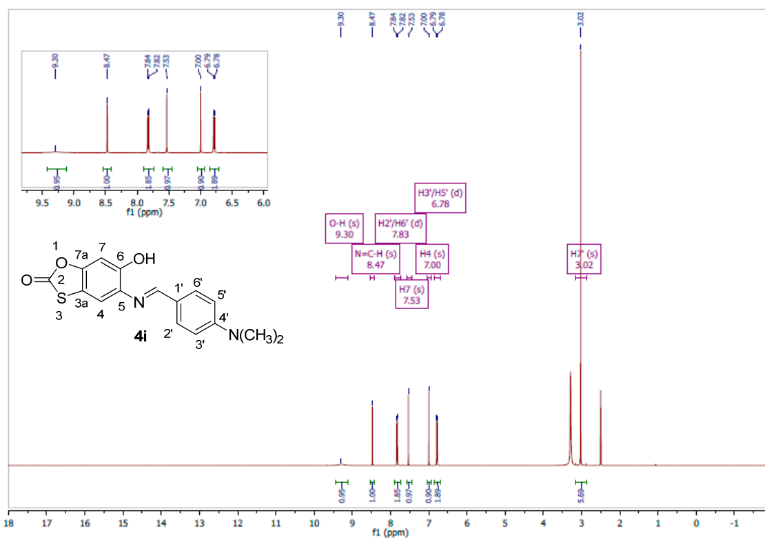
Figure S11. (E) -5-(4-(Dimethylamino)benzylideneamino)-6-hydroxybenzo[ d ][1,3]oxathiol-2-one ( 4i ).
