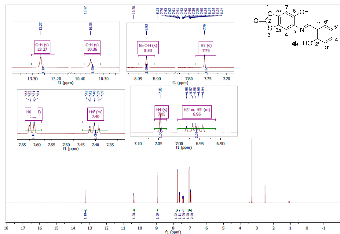
Figure S13. ( E )-6-Hydroxy-5-(2-hydroxybenzylideneamino)benzo[ d ][1,3]oxathiol-2-one ( 4k ).
