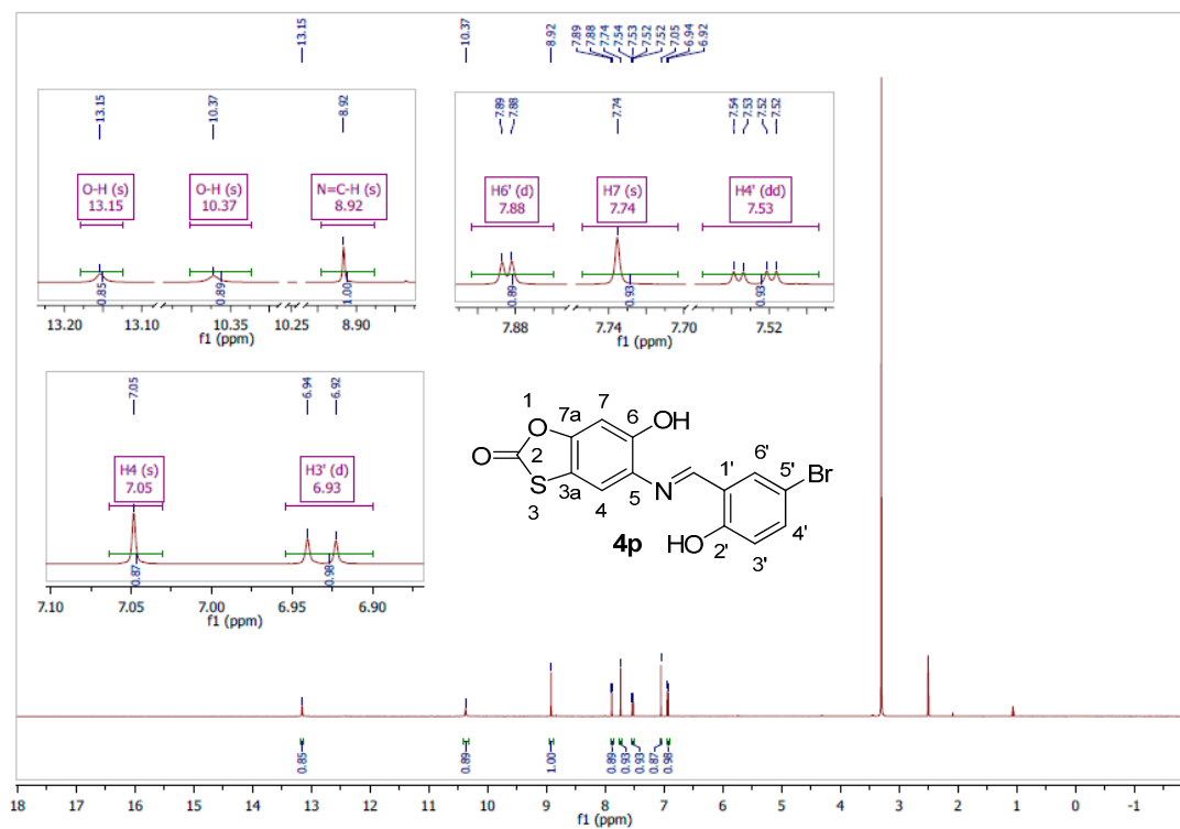
Figure S18. (E) -5-(5-Bromo-2-hydroxybenzylideneamino)-6-hydroxybenzo[ d ][1,3]oxathiol-2-one ( 4p ).
