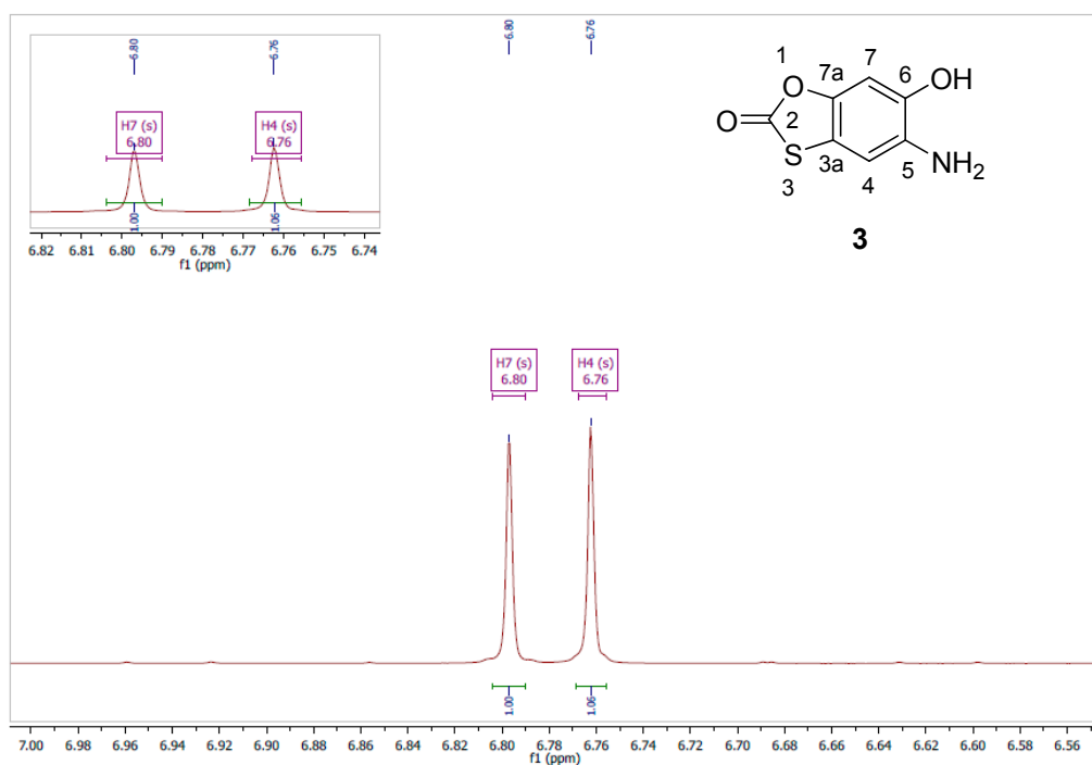
Figure S2. 5-Amino-6-hydroxybenzo[d][1,3]oxathiol-2-one ( 3 ).
