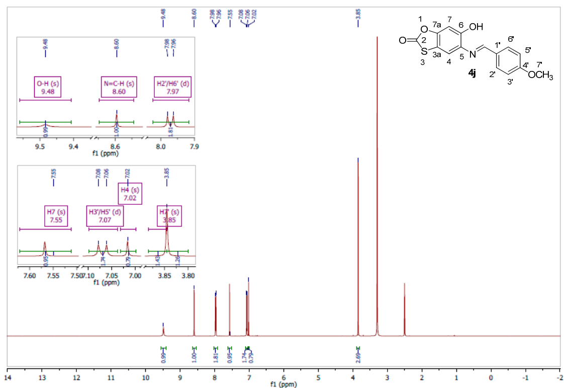
Figure S12. ( E )-6-Hydroxy-5-(4-methoxybenzylideneamino)benzo[ d ][1,3]oxathiol-2-one ( 4j ).
