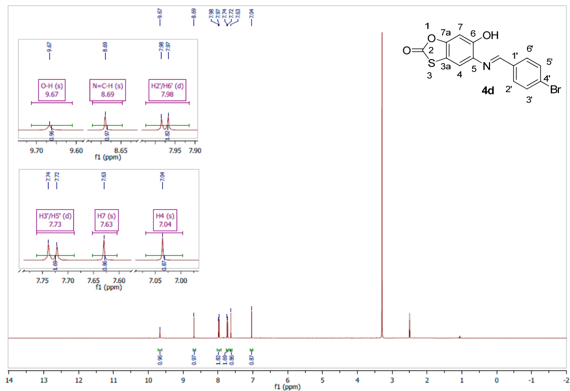
Figure S6. ( E )-5-(4-Bromobenzylideneamino)-6-hydroxybenzo[ d ][1,3]oxathiol-2-one ( 4d ).
