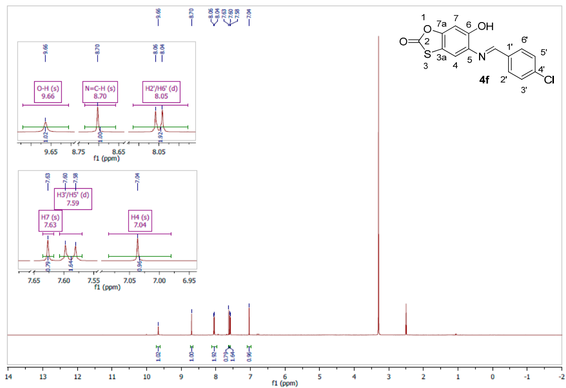
Figure S8. ( E )-5-(4-Chlorobenzylideneamino)-6-hydroxybenzo[ d ][1,3]oxathiol-2-one ( 4f ).
