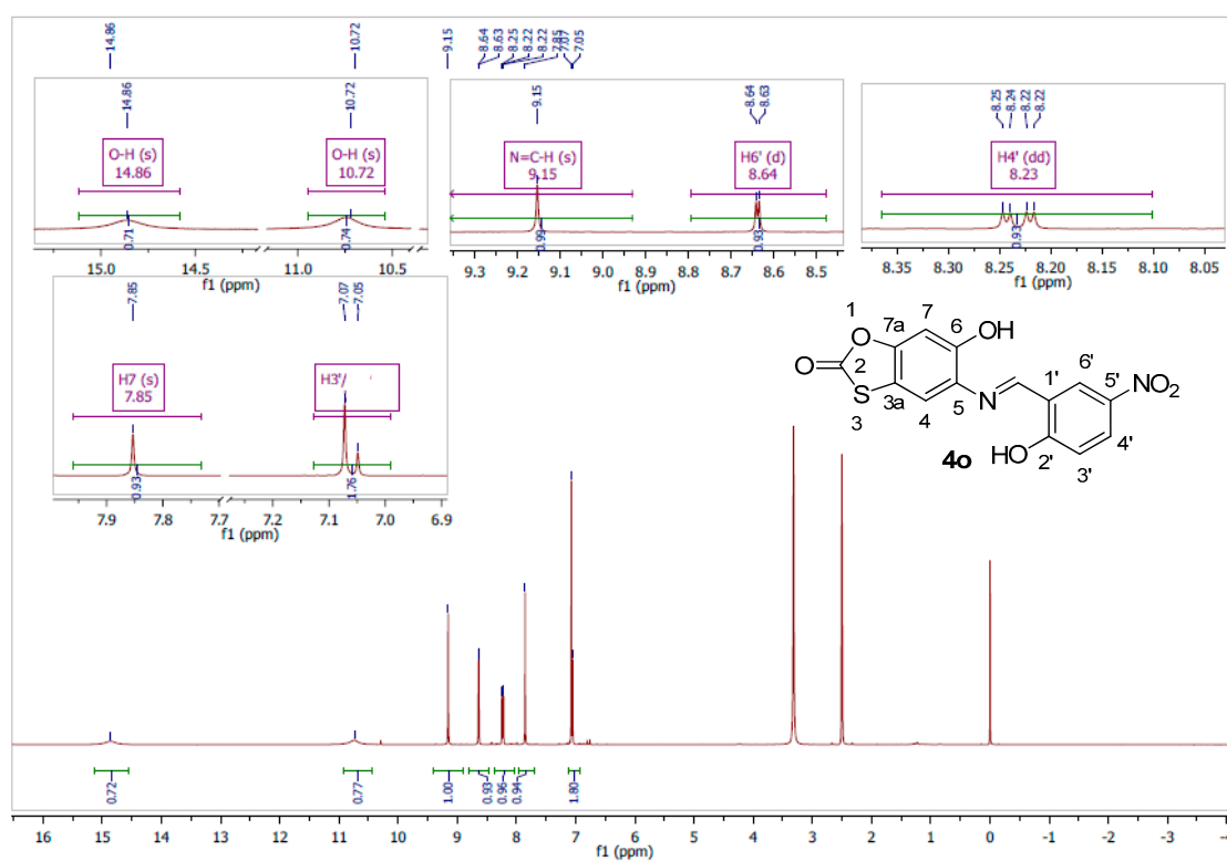
Figure S17. ^1\text{H} NMR spectrum of (E) -6-Hydroxy-5-(2-hydroxy-5-nitrobenzylideneamino)benzo[ d ][1,3]oxathiol-2-one ( 4o ).
