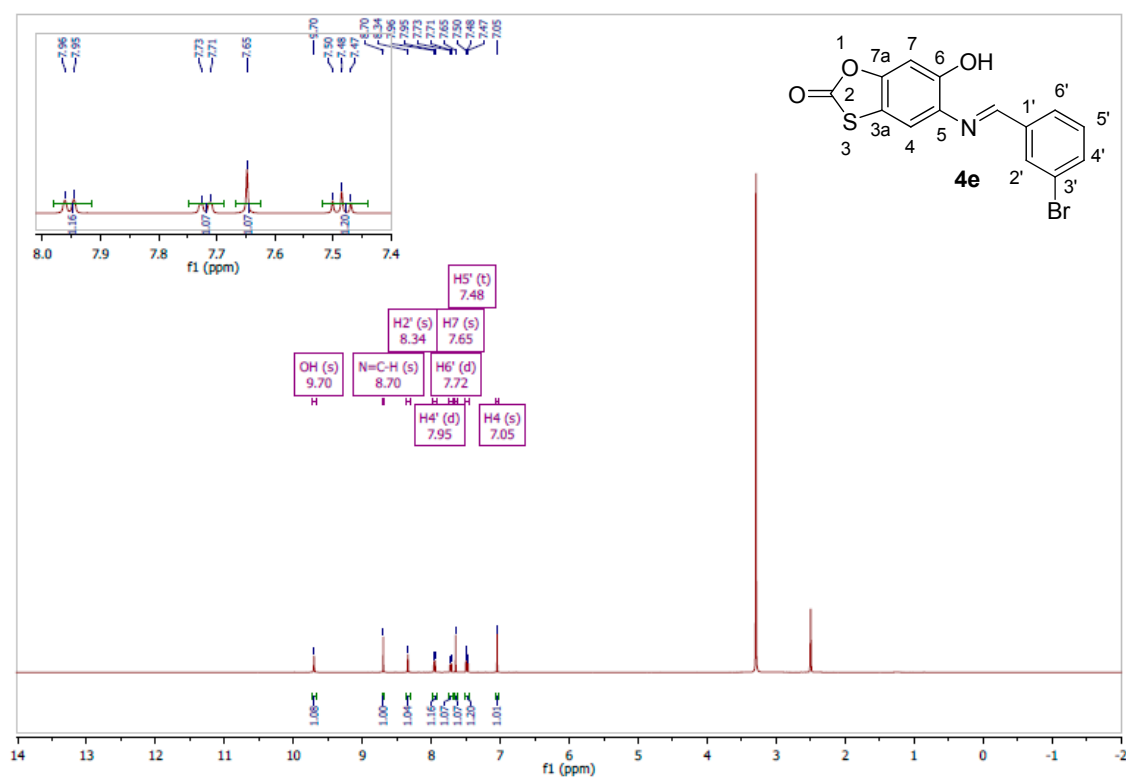
Figure S7. ( E )-5-(3-Bromobenzylideneamino)-6-hydroxybenzo[ d ][1,3]oxathiol-2-one ( 4e ).
