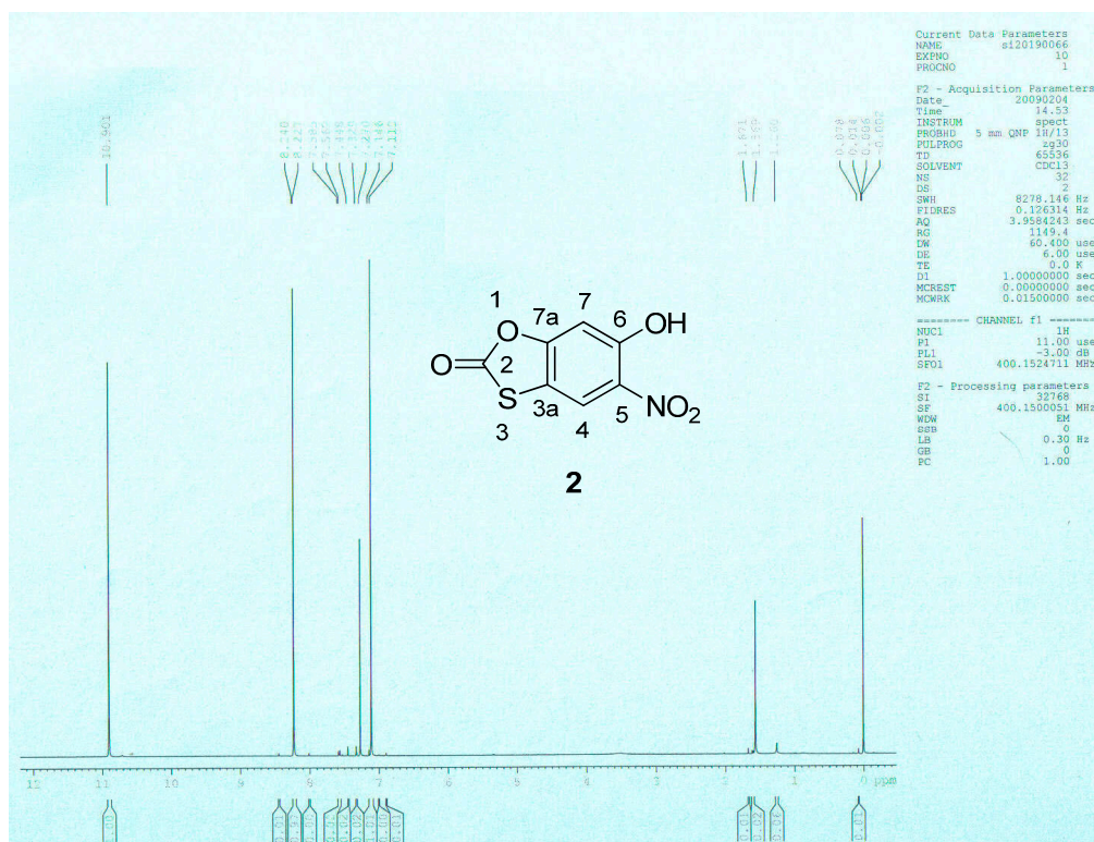
Figure S1. 6-Hydroxy-5-nitrobenzo[d][1,3]oxathiol-2-one ( 2 ).
