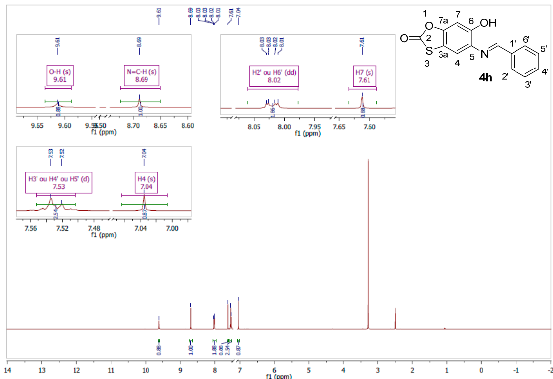
Figure S10. (E) -5-(Benzylideneamino)-6-hydroxybenzo[ d ][1,3]oxathiol-2-one ( 4h ).
