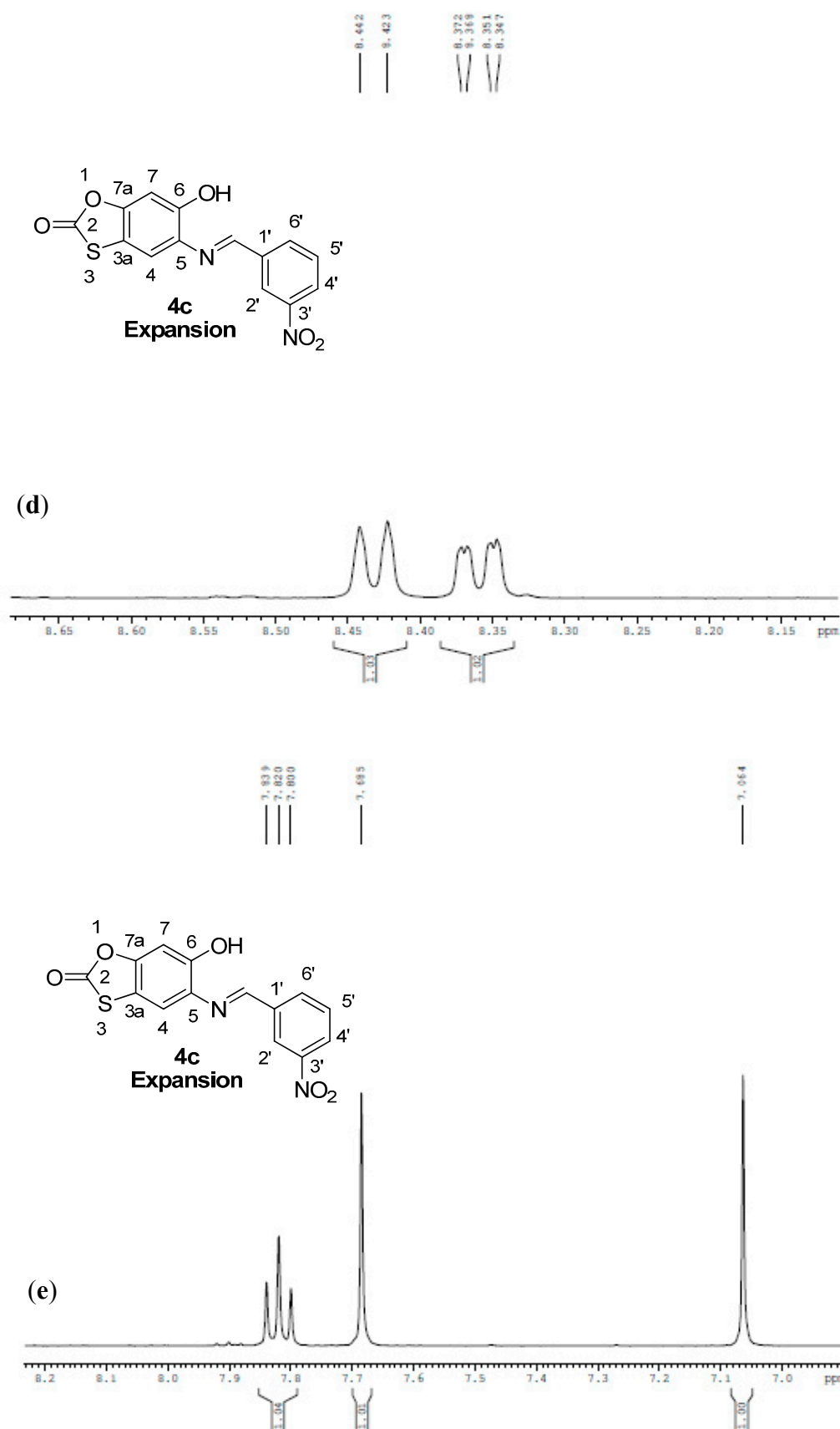
Figure S5. (a) (E) -6-Hydroxy-5-(3-nitrobenzylideneamino)benzo[ d ][1,3]oxathiol-2-one ( 4c ). (b–e) Expansion.
