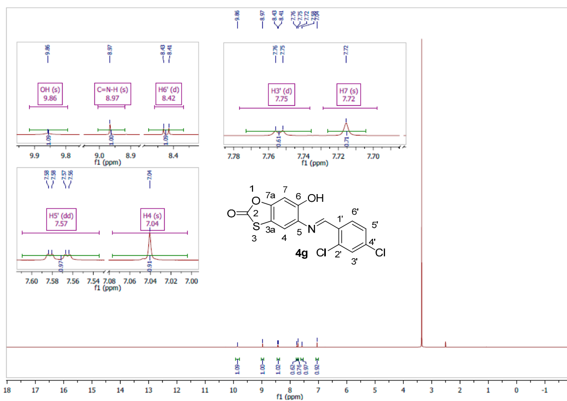
Figure S9. ( E )-5-(2,4-Dichlorobenzylideneamino)-6-hydroxybenzo[ d ][1,3]oxathiol-2-one ( 4g ).
