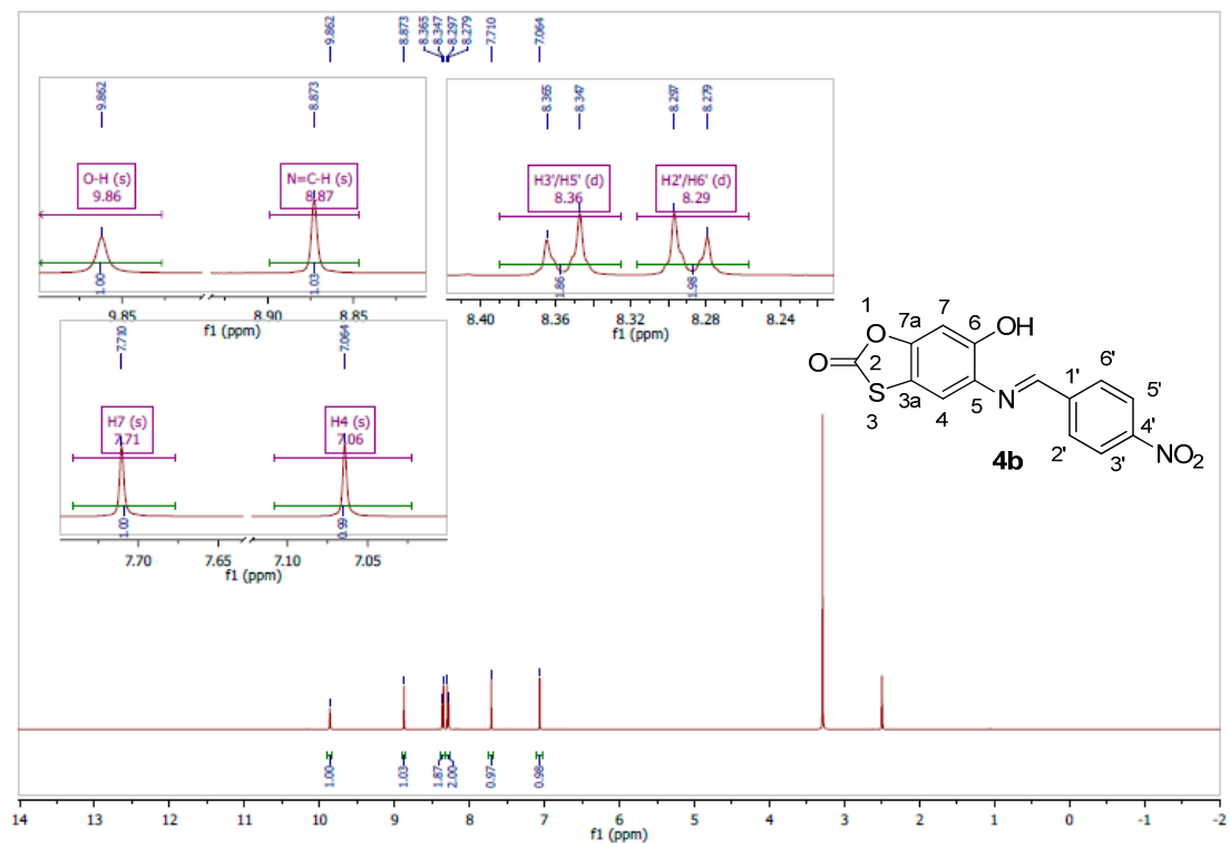
Figure S4. ( E )-6-Hydroxy-5-(4-nitrobenzylideneamino)benzo[ d ][1,3]oxathiol-2-one ( 4b ).
