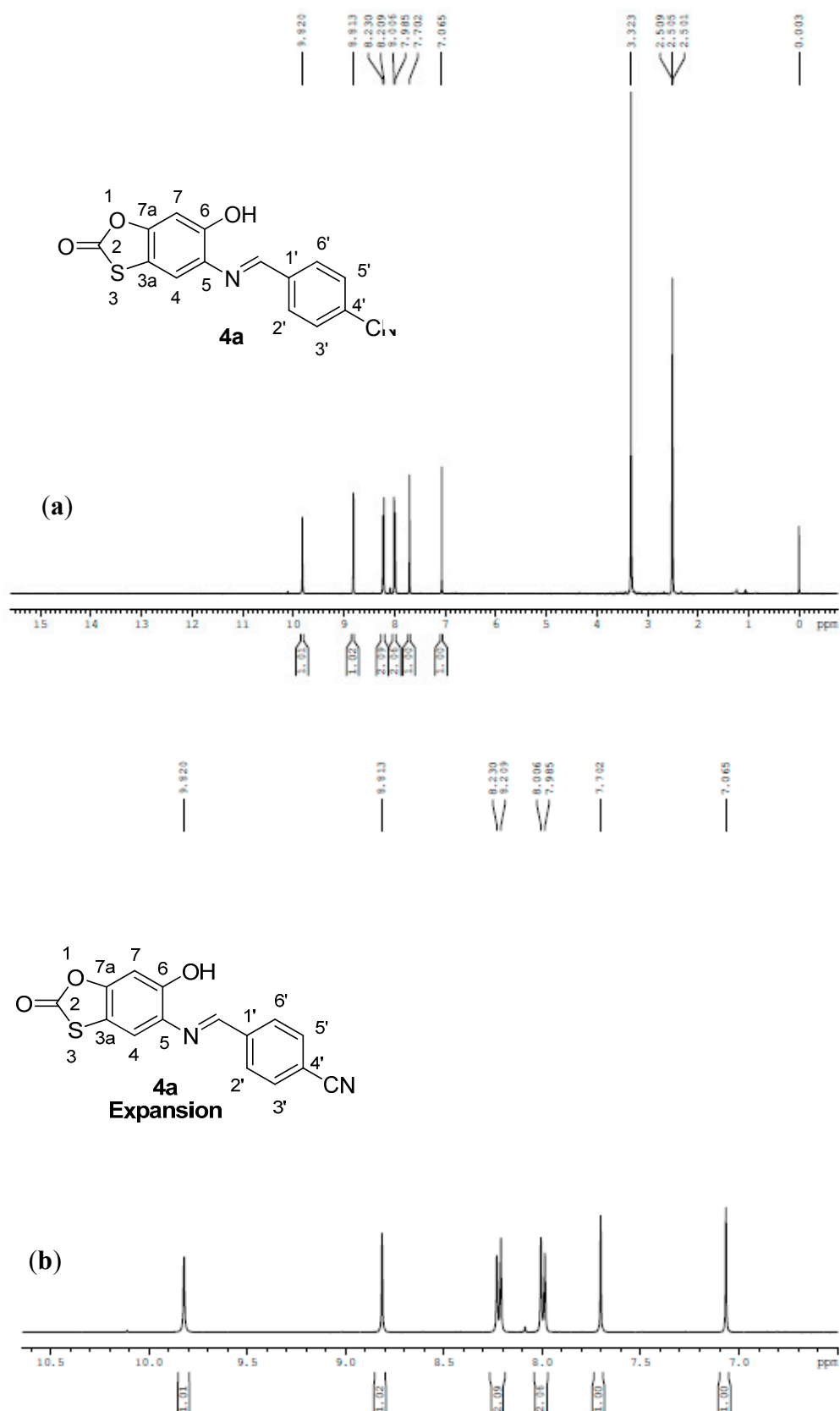
Figure S3. (a) ( E )-4-((6-Hydroxy-2-oxobenzo[ d ][1,3]oxathiol-5ylimino)methyl)benzonitrile ( 4a ), (b) Expansion.
