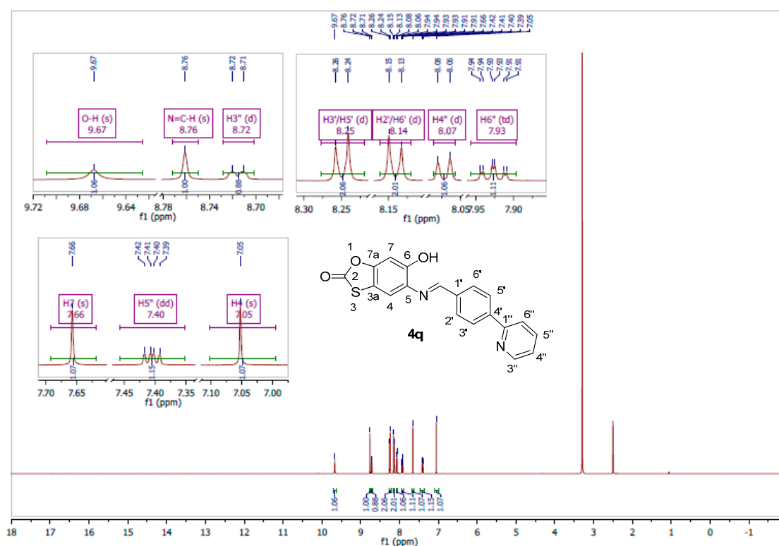
Figure S19. (E) -6-Hydroxy-5-(4-(pyridin-2-yl)benzylideneamino)benzo[ d ][1,3]oxathiol-2-one ( 4q ).
