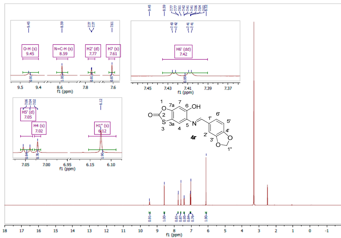
Figure S20. ( E )-5-(Benzo[ d ][1,3]dioxol-5-ylmethyleneamino)-6-hydroxybenzo[ d ][1,3]oxathiol-2-one ( 4r ).
