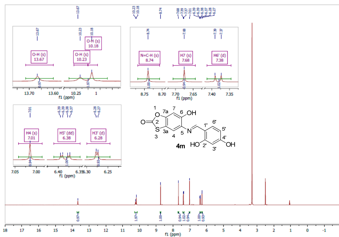
Figure S15. (E) -5-(2,4-Dihydroxybenzylideneamino)-6-hydroxybenzo[ d ][1,3]oxathiol-2-one ( 4m ).
