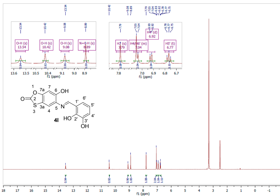
Figure S14. (E) -5-(2,3-Dihydroxybenzylideneamino)-6-hydroxybenzo[ d ][1,3]oxathiol-2-one ( 4l ).
