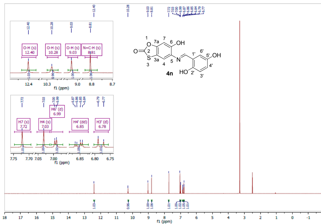
Figure S16. ^1\text{H} NMR spectrum of (E) -5-(2,5-Dihydroxybenzylideneamino)-6-hydroxybenzo[ d ][1,3]oxathiol-2-one ( 4n ).
