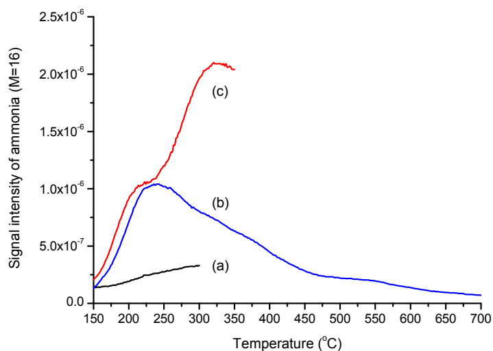
Figure S1. A comparison of thermodesorption curves of ammonia from: (a) montmorillonite; (b) zeolite Beta; and (c) ion-exchange resin Purolite.
