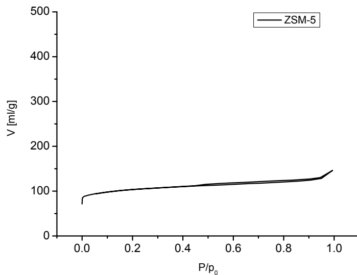
Figure S2. Adsorption/desorption isotherms of nitrogen on the ZSM-5 sample.
