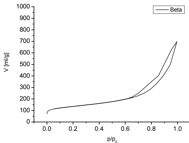
Figure S3. Adsorption/desorption isotherms of nitrogen on the Beta type zeolite.
