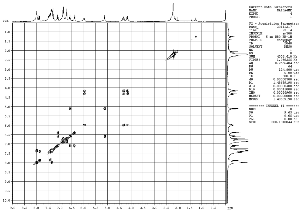
Figure 5. ^1\text{H} , ^1\text{H} -COSY spectrum of 6h .
