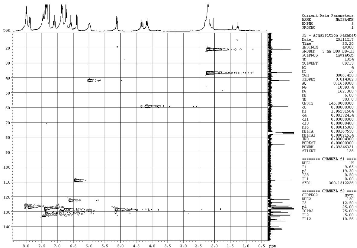
Figure 6. ^{13}\text{C} , ^1\text{H} -COSY spectrum of 6h .
