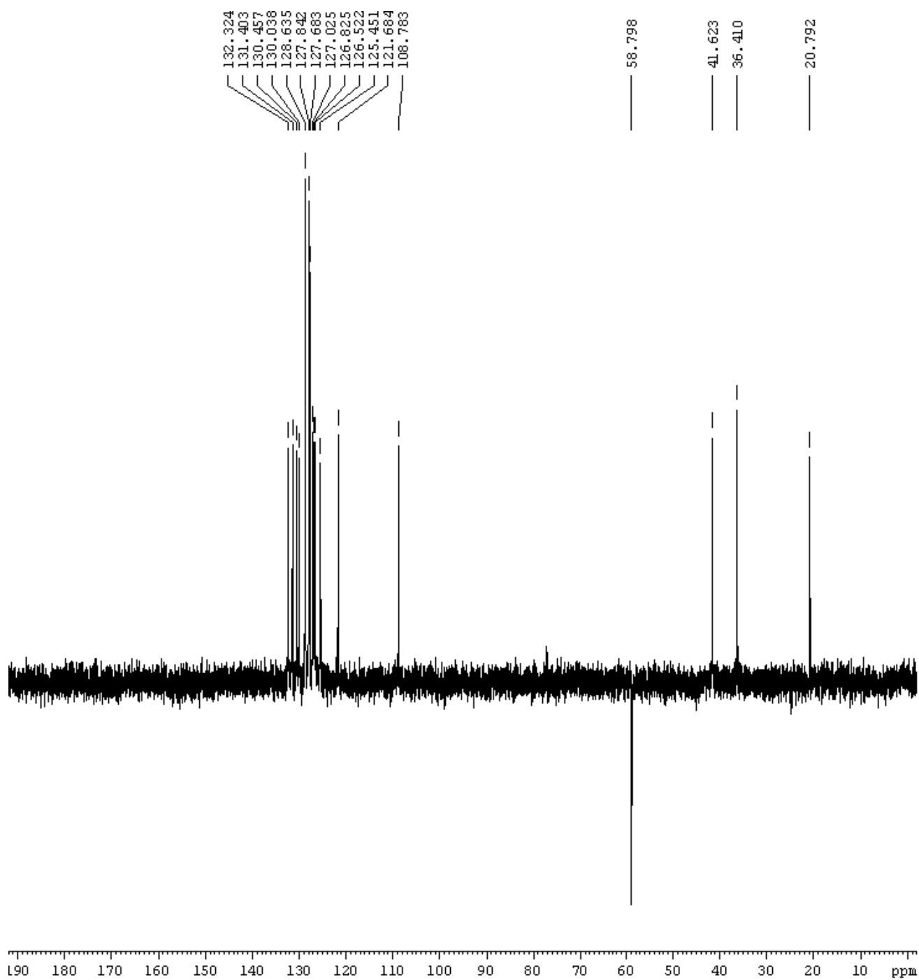
Figure 4. DEPT 135 spectrum of 6h .
