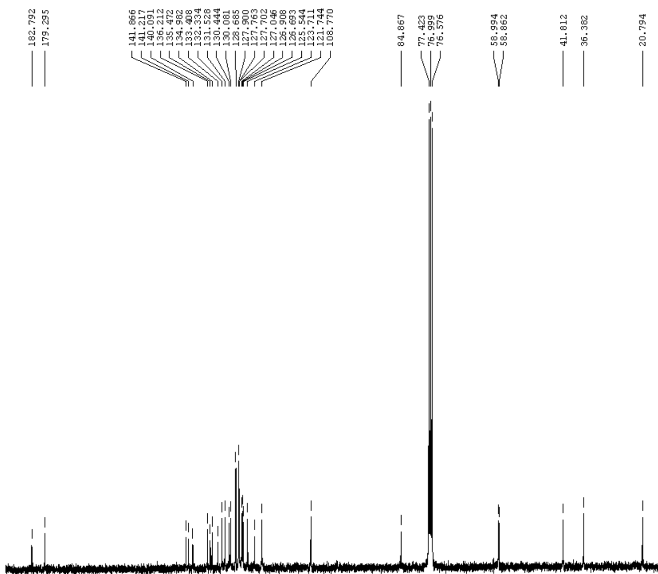
Figure 3. ^{13}\text{C} -NMR spectrum of 6h.
