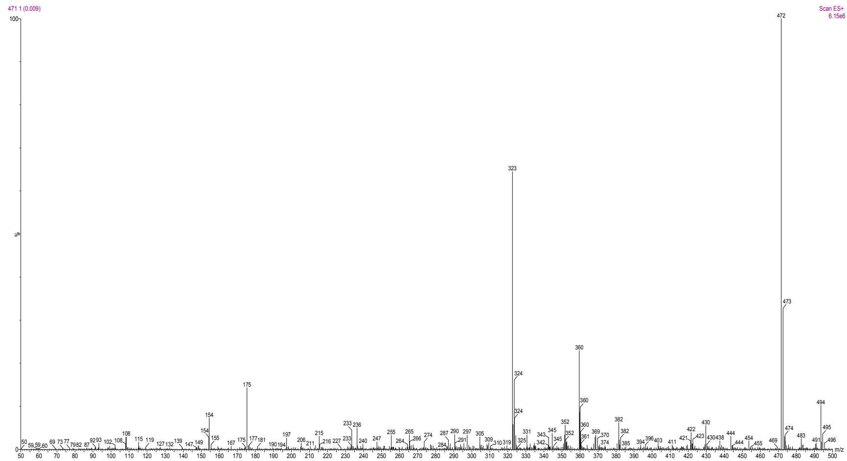
Figure 7. Mass spectrum of 6h.
