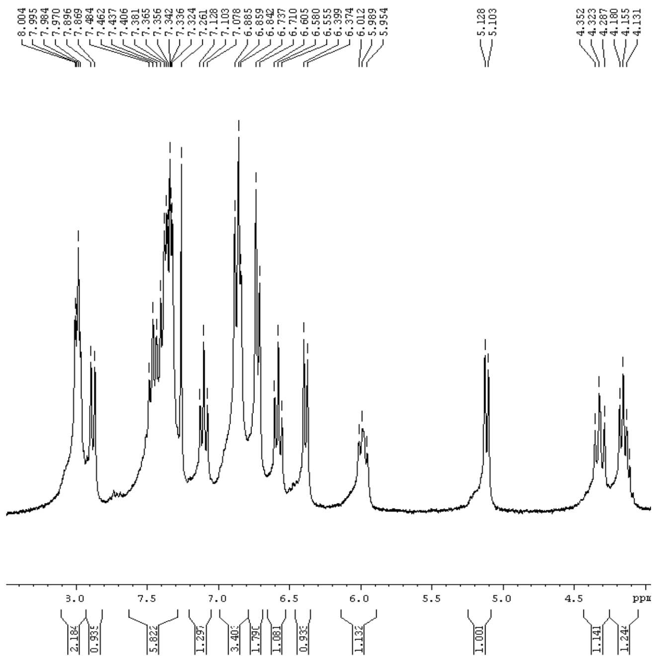
Figure 2. Expanded ^1\text{H} -NMR spectrum of 6h .
