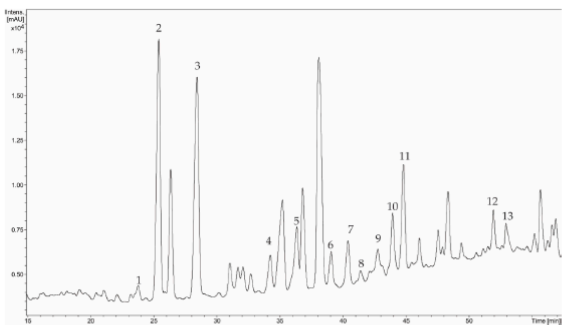
Chromatogram of Boswellia serrata . For chromatographic conditions, please refer to Materials and Methods. Peak numbers correspond to compounds listed in Table 1
