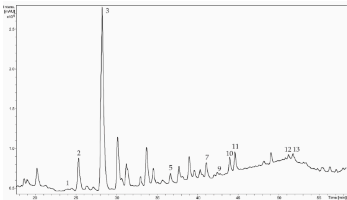
Chromatogram of Boswellia sacra . For chromatographic conditions, please refer to Materials and Methods. Peak numbers correspond to compounds listed in Table 1
