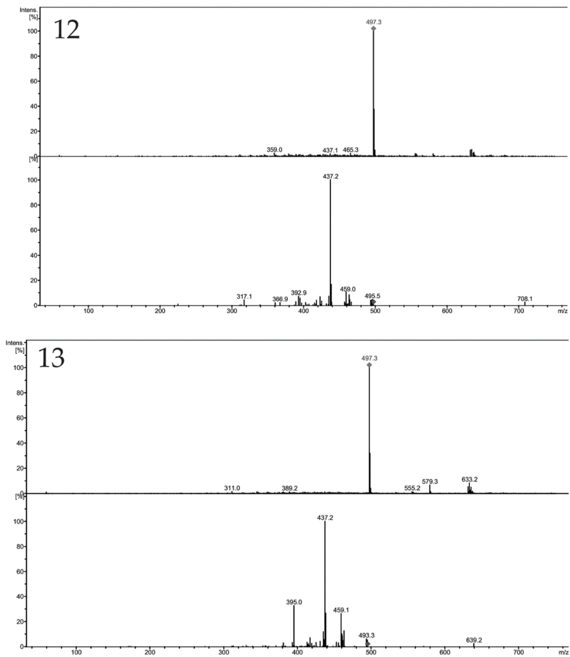
Figure S1. Mass spectra (MS 2 ) of identified boswellic acids. In each plate, upper left numbers correspond to molecules listed in Table 1.
