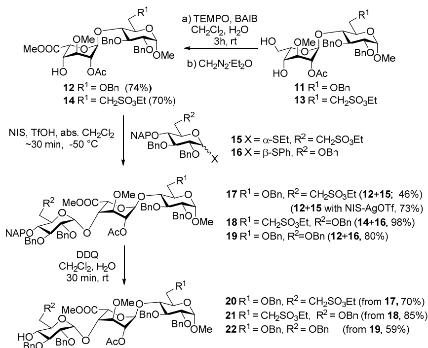
Scheme 1. Preparation of the FGH building blocks.
