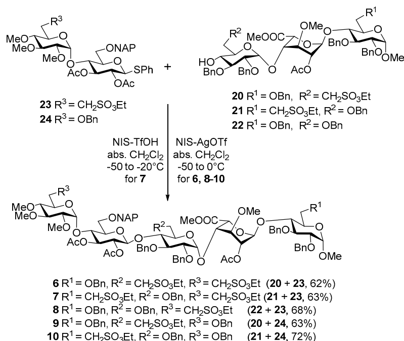
Scheme 2. Synthesis of the protected pentasaccharide derivatives.
