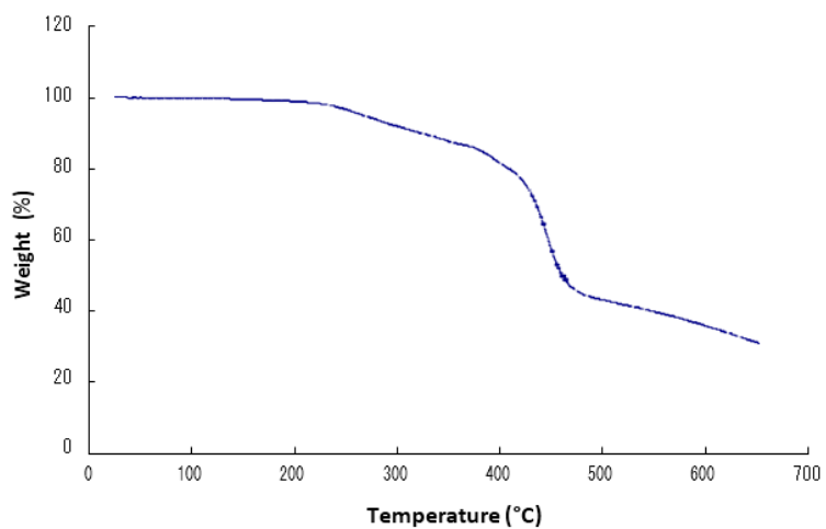
Figure S4. TGA result for the obtained PPO.
