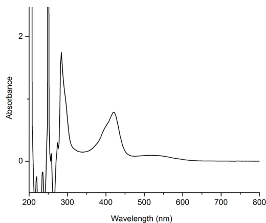
Figure S2. UV-vis spectrum of the polymerization solution.
