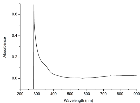
Figure S1. UV-vis spectrum of the PSt-polyTACN with CuCl 2 present in toluene.
