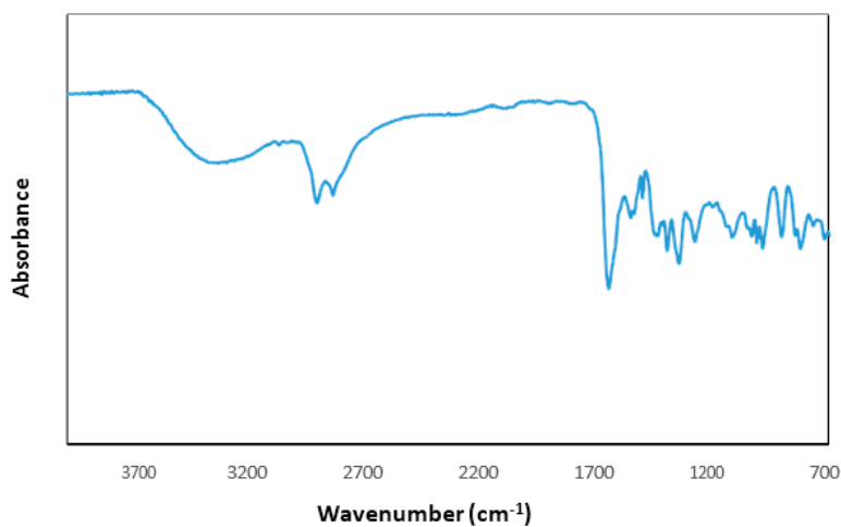
Figure S3. FT-IR spectrum of the obtained PPO.
