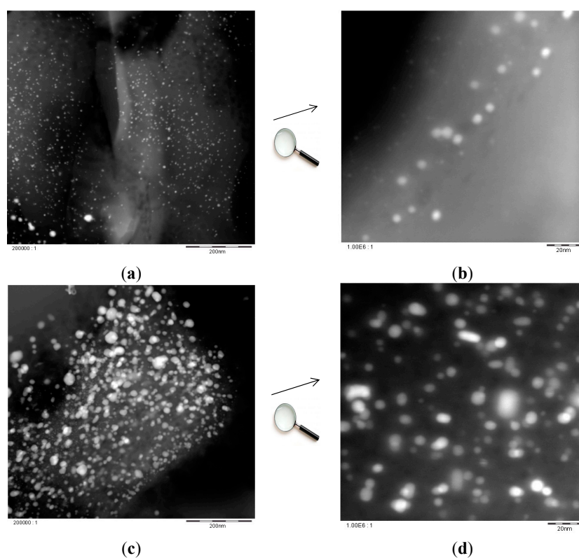
Figure 4. HAADF-STEM images of Au/silicalite-1 catalysts: (a) cat I (0.5% Au/silicalite-1 doped with CH_3COOK/Au = 20 ), enlargement 200,000:1; (b) cat I, enlargement 1,000,000:1; (c) cat M (16.3% Au/silicalite-1 doped with CH_3COOK/Au = 20 ), enlargement 200,000:1; and (d) cat M, enlargement 1,000,000:1.
