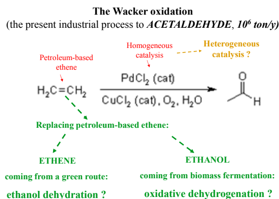
Figure 2. Potential green alternative to the Wacker oxidation.
