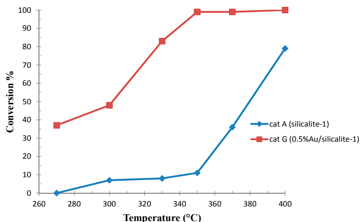
Figure 3. Comparison between unloaded silicalite-1 (cat A) and 0.5% Au/silicalite-1 (cat G) in ethanol conversion to Et 2 O and C 2 H 4 .
