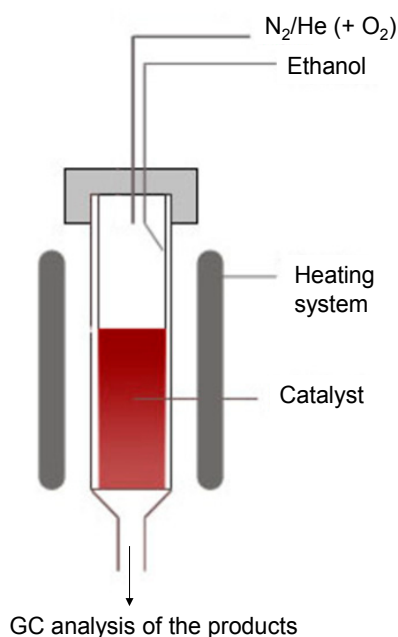
Figure 5. Vertical glass reactor.
