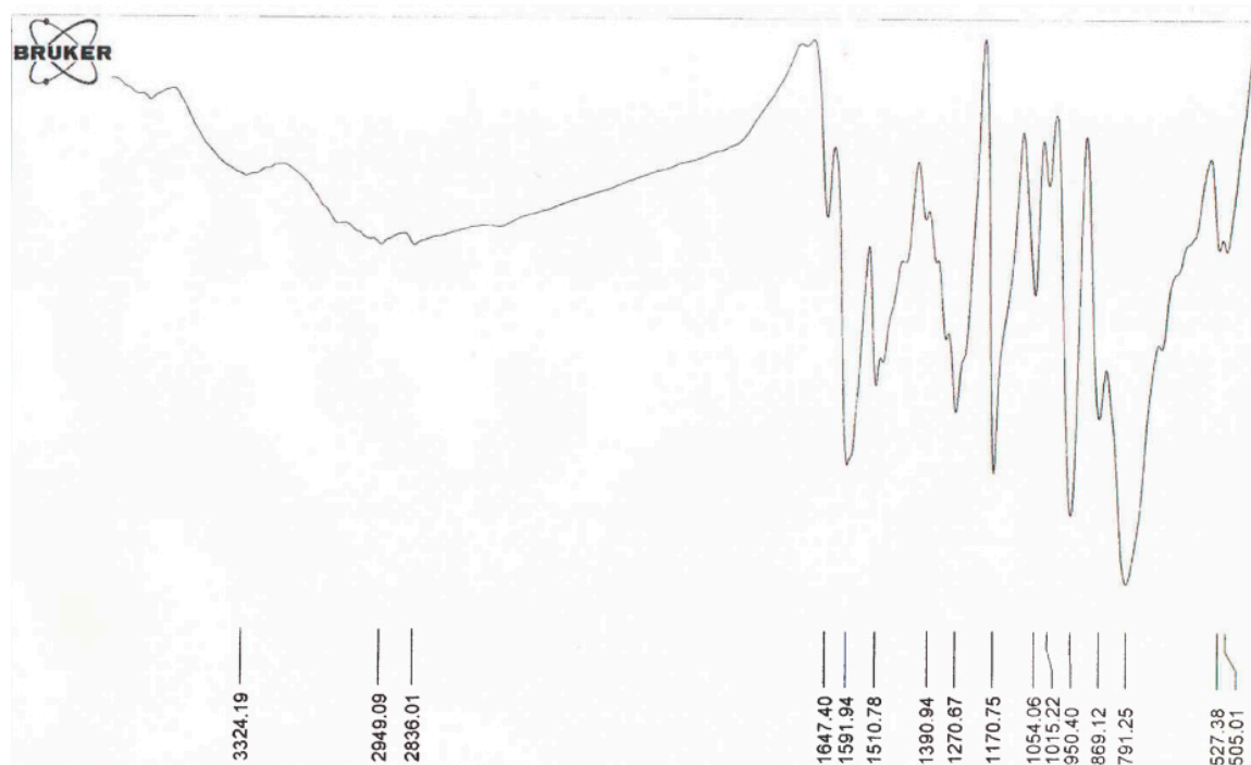
Figure S14. The FTIR spectrum of compound (Entry 11-Table 2).
