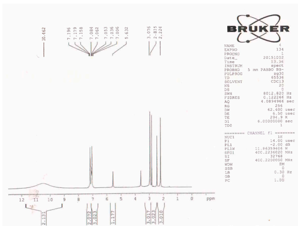
Figure S2. The 1 H-NMR spectrum of compound Entry 1-Table 2).
