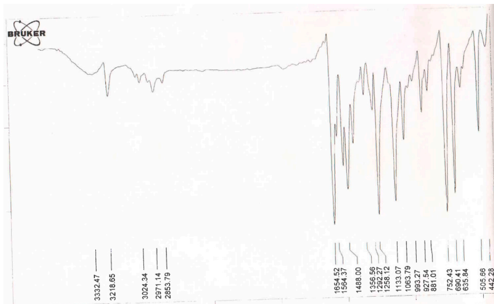
Figure S1. The FTIR spectrum of compound (Entry 1-Table 2).
