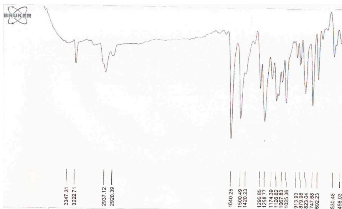
Figure S8. The FTIR spectrum of compound (Entry 6-Table 2).
