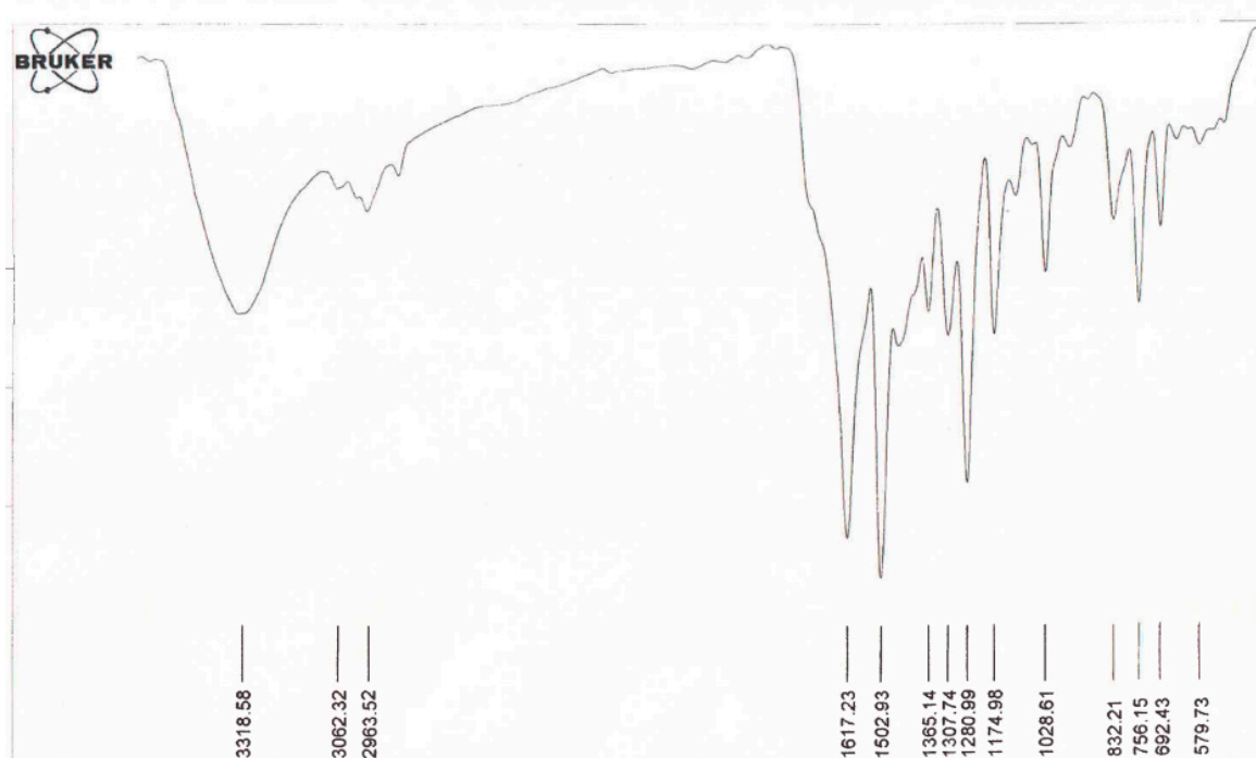
Figure S11. The FTIR spectrum of compound (Entry 8-Table 2).
