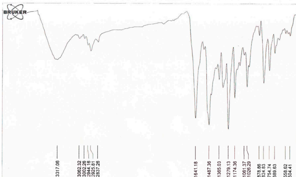
Figure S17. The FTIR spectrum of compound (Entry 13-Table 2).
