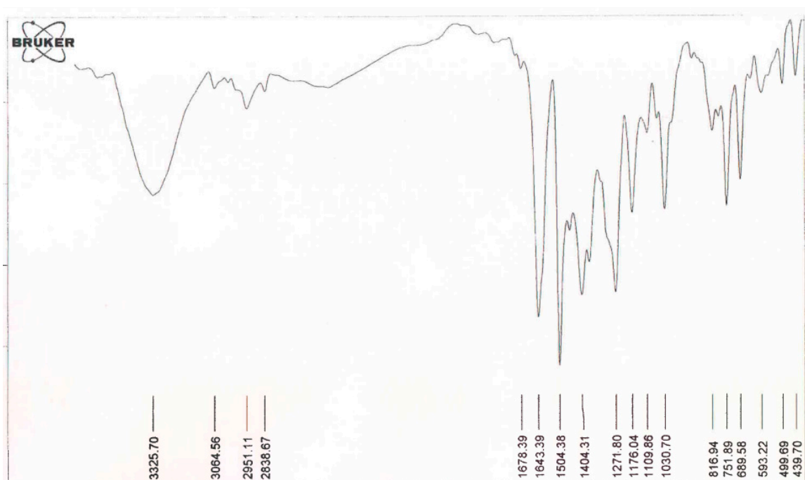
Figure S10. The FTIR spectrum of compound (Entry 7-Table 2).
