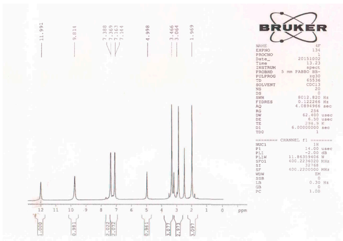
Figure S4. The 1 H-NMR spectrum of compound (Entry 3-Table 2).
