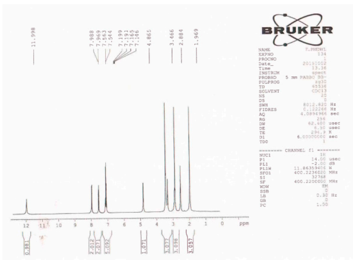
Figure S15. The ^1\text{H} -NMR spectrum of compound (Entry 12-Table 2).
