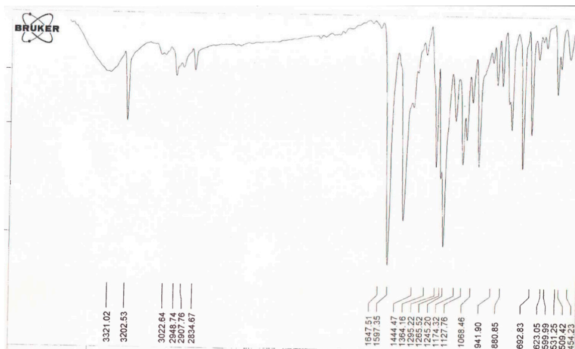
Figure S6. The FTIR spectrum of compound (Entry 4-Table 2).
