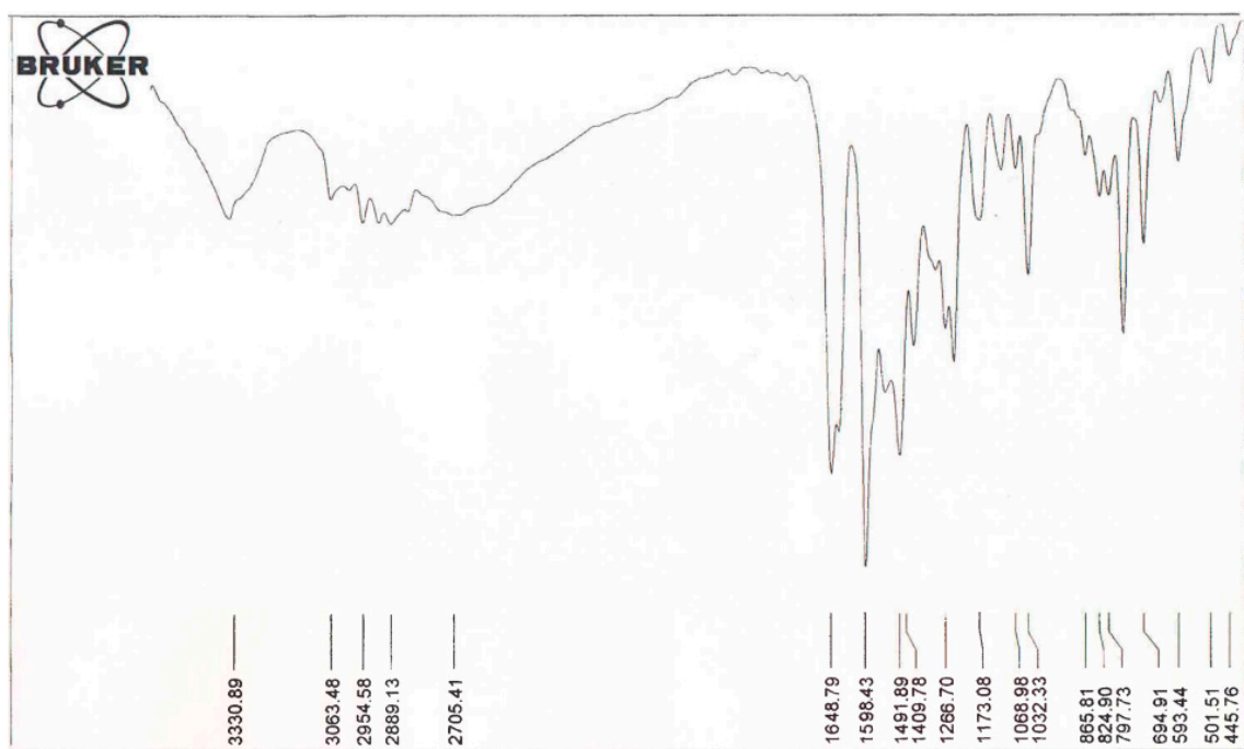
Figure S18. The FTIR spectrum of compound (Entry 14-Table 2).
