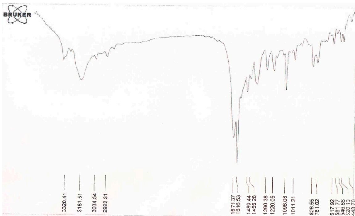
Figure S9. The FTIR spectrum of compound (Entry 6-Table 2).
