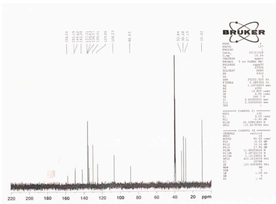
Figure S5. The ^{13}\text{C} -NMR spectrum of compound Entry 3-Table 2)
