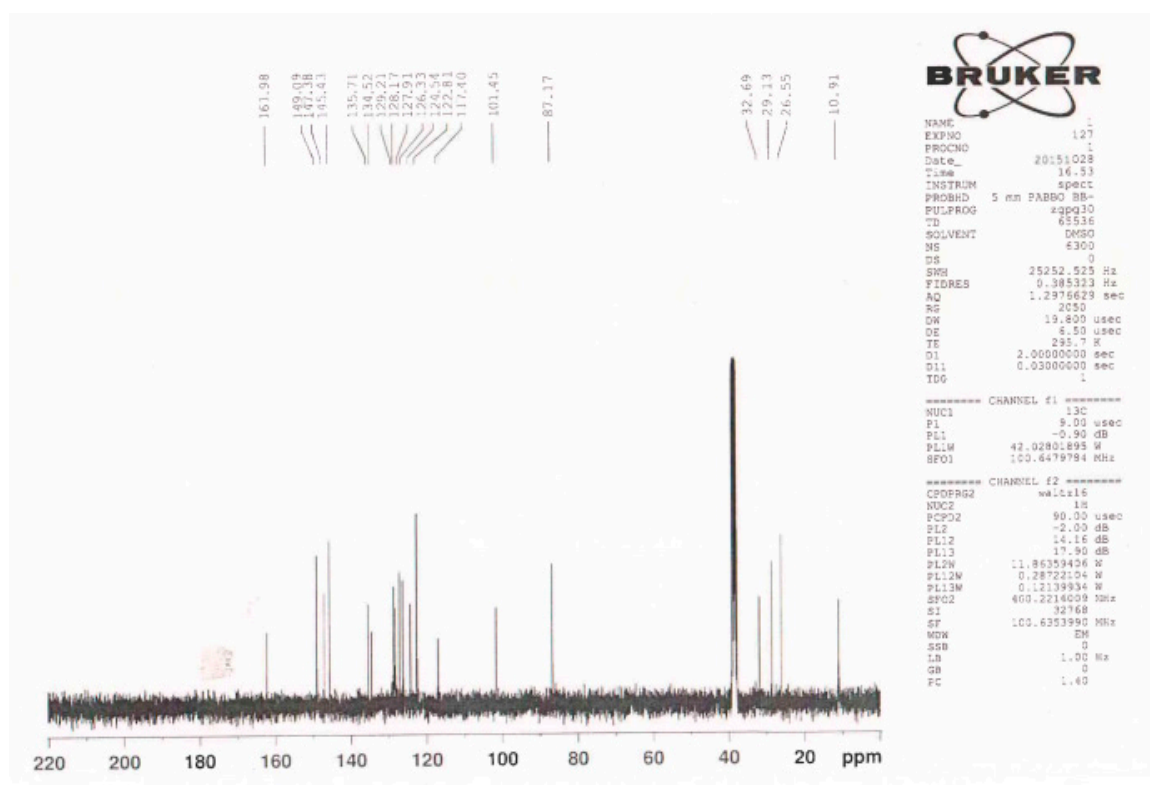
Figure S16. The ^{13}\text{C} -NMR spectrum of compound (Entry 12-Table 2).
