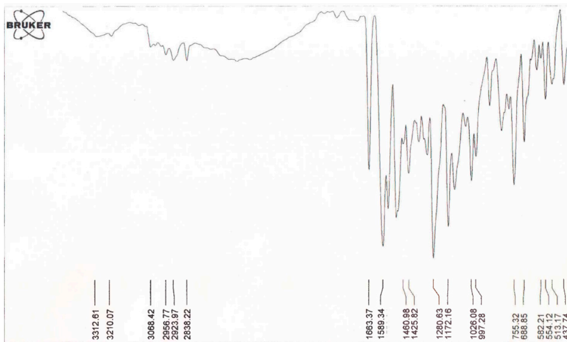
Figure S3. The FTIR spectrum of compound (Entry 2-Table 2).
