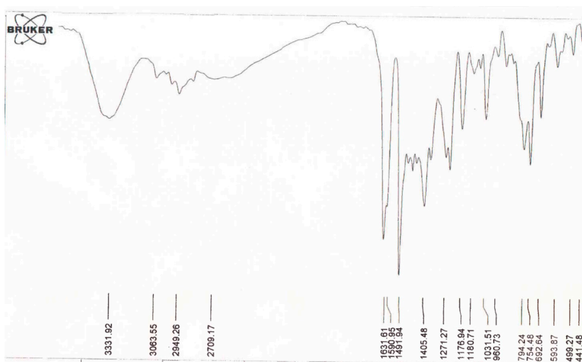
Figure S12. The FTIR spectrum of compound (Entry 9-Table 2).
