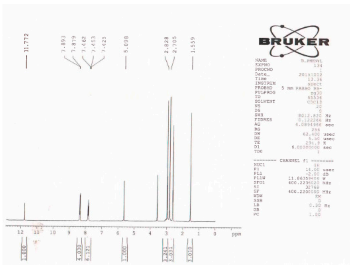
Figure S13. The ^1\text{H} -NMR spectrum of compound (Entry 10-Table 2).
