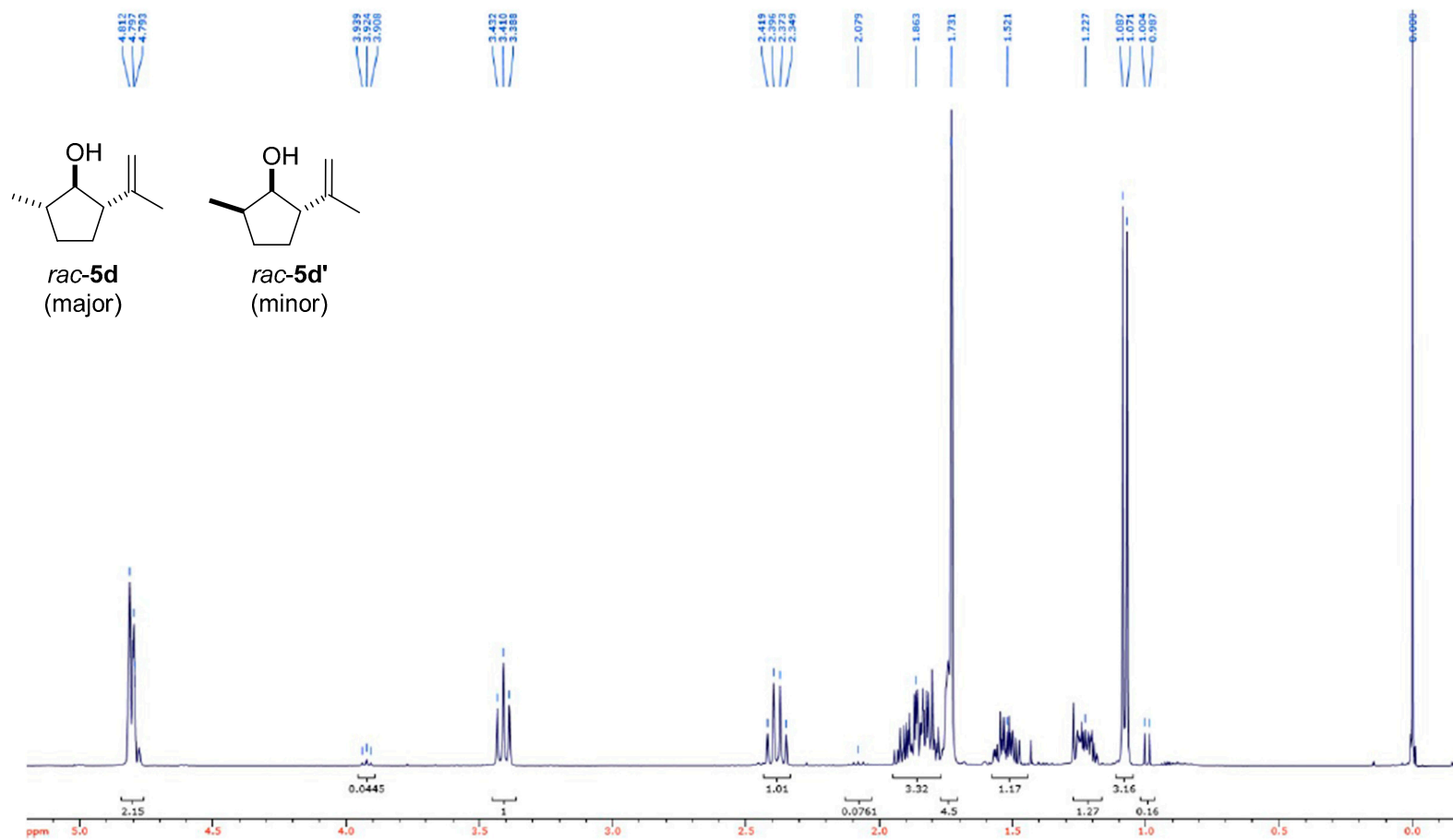
Figure S5. 1 H-NMR of 5d/d'.
