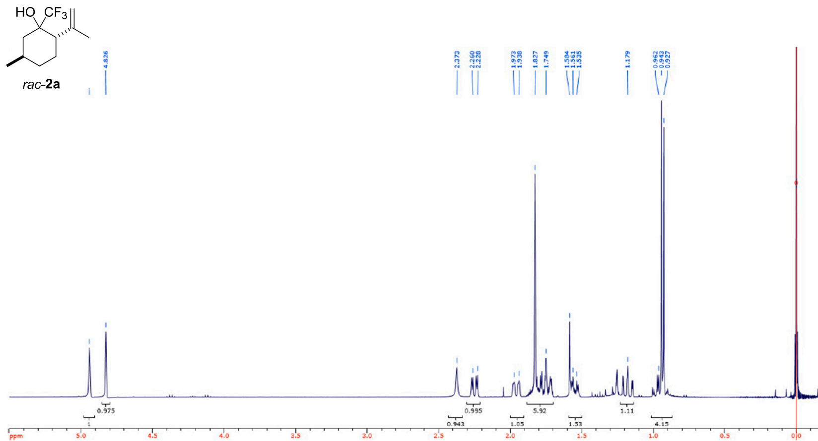
Figure S1. 1 H-NMR of 2a .
