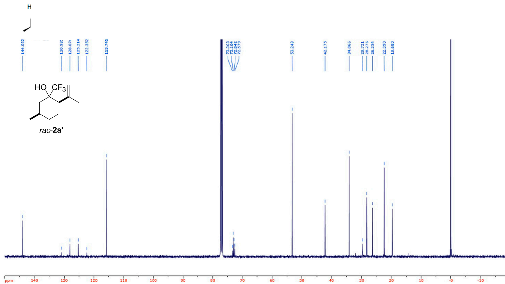
Figure S4. 13 C-NMR of 2a' .
