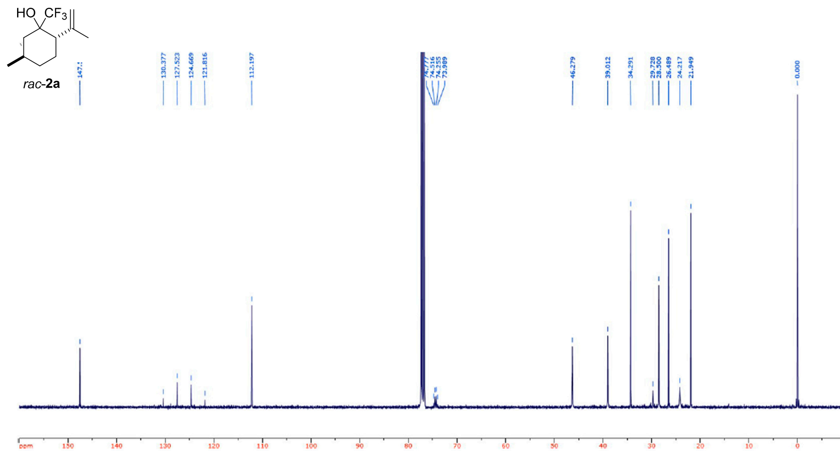
Figure S2. 13 C-NMR of 2a.
