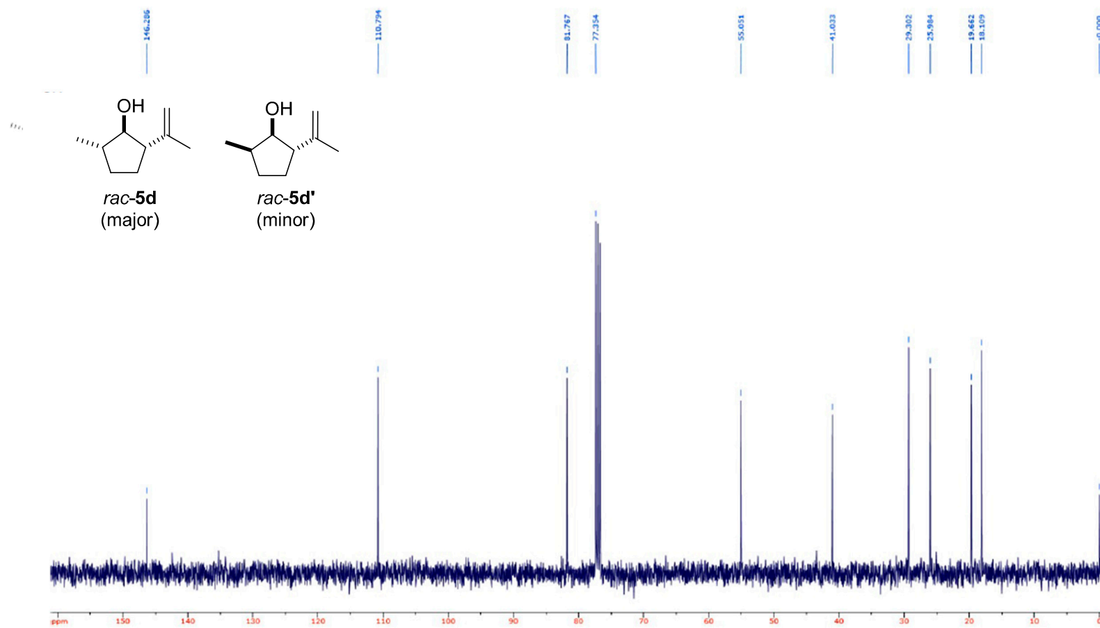
Figure S6. ^{13}\text{C} -NMR of 5d/d'.
