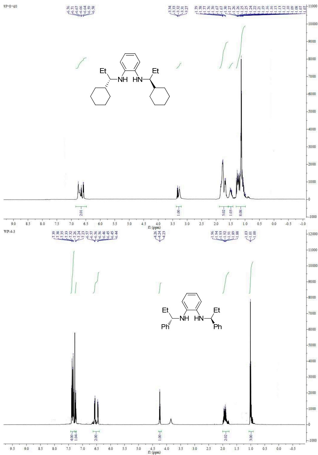
Figure S1. 1 H-NMR Spectra of compounds 1a-d.
