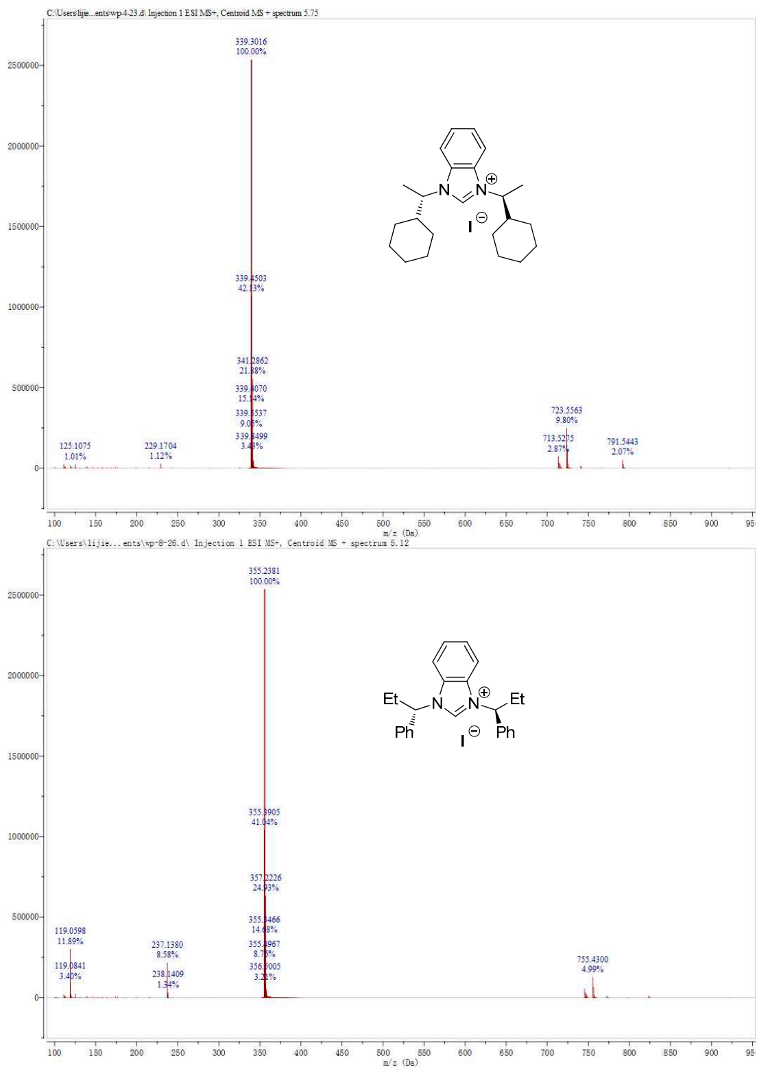
Figure S3. HR-MS Spectra for compounds 3a-d.
