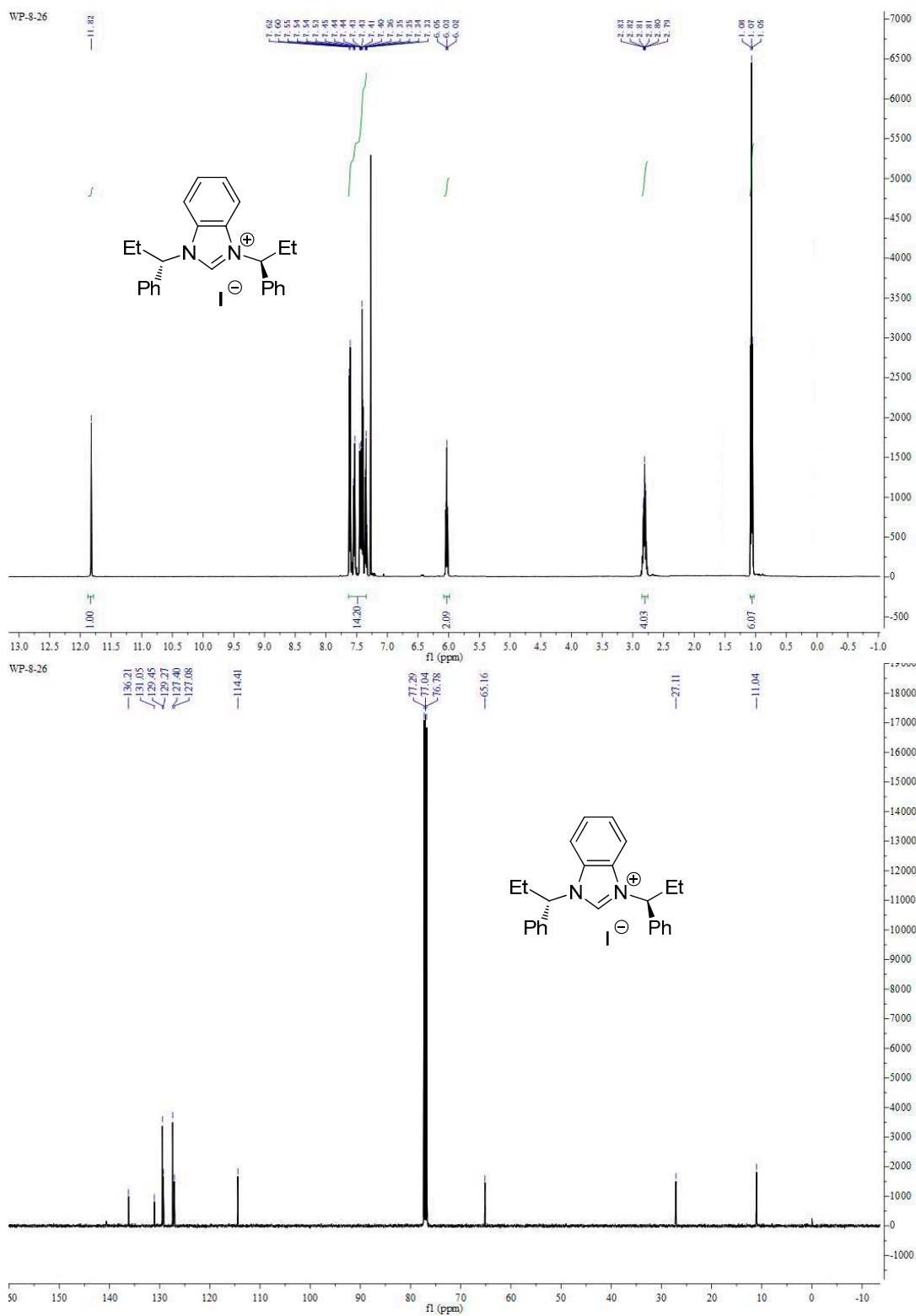
Figure S2. 1 H and 13 C-NMR Spectra of compounds 3a–d.
