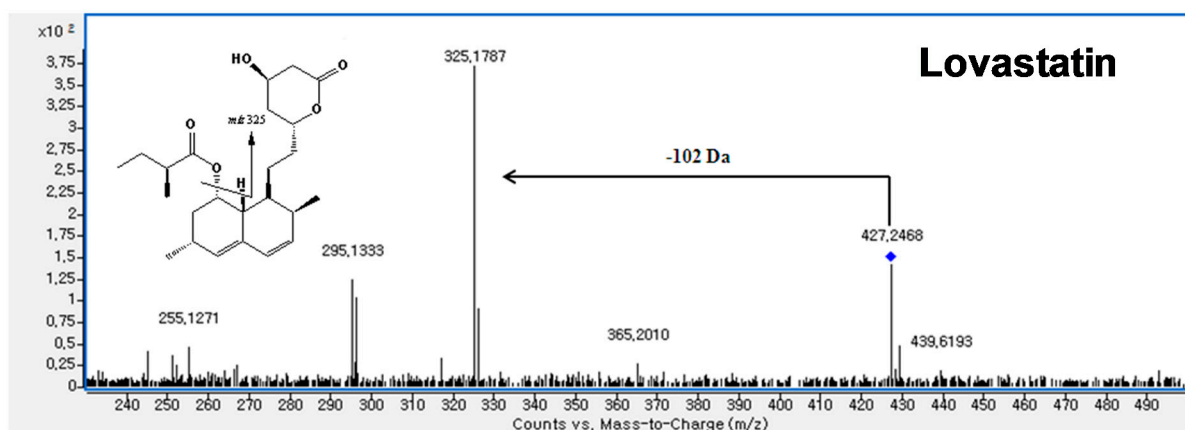
Figure S5. MS/MS spectrum of lovastatin.
