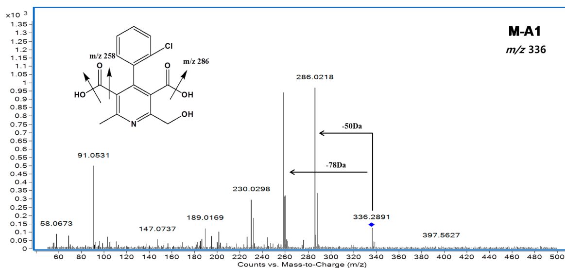
Figure S2. MS/MS spectrum of M-A1.
