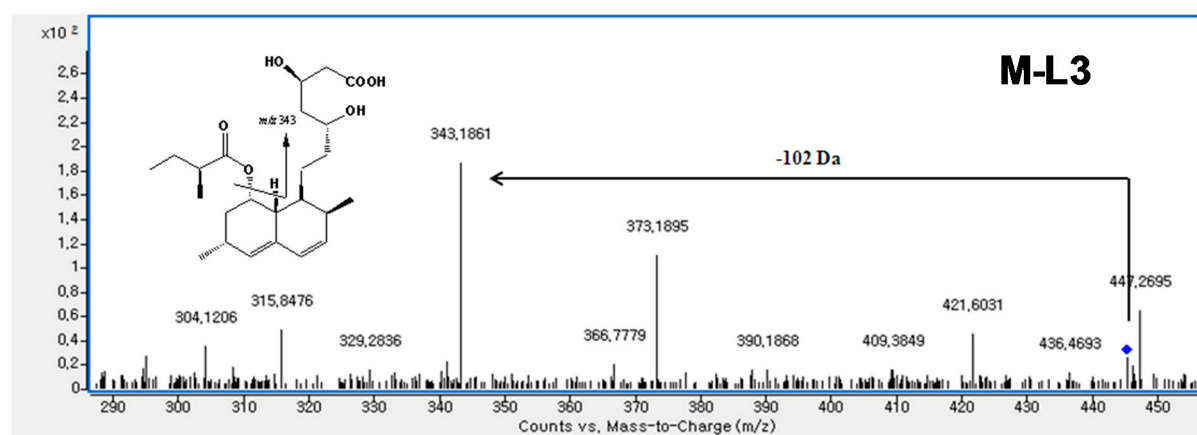
Figure S7. MS/MS spectrum of M-L3.
