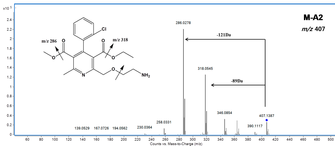
Figure S3. MS/MS spectrum of M-A2.
