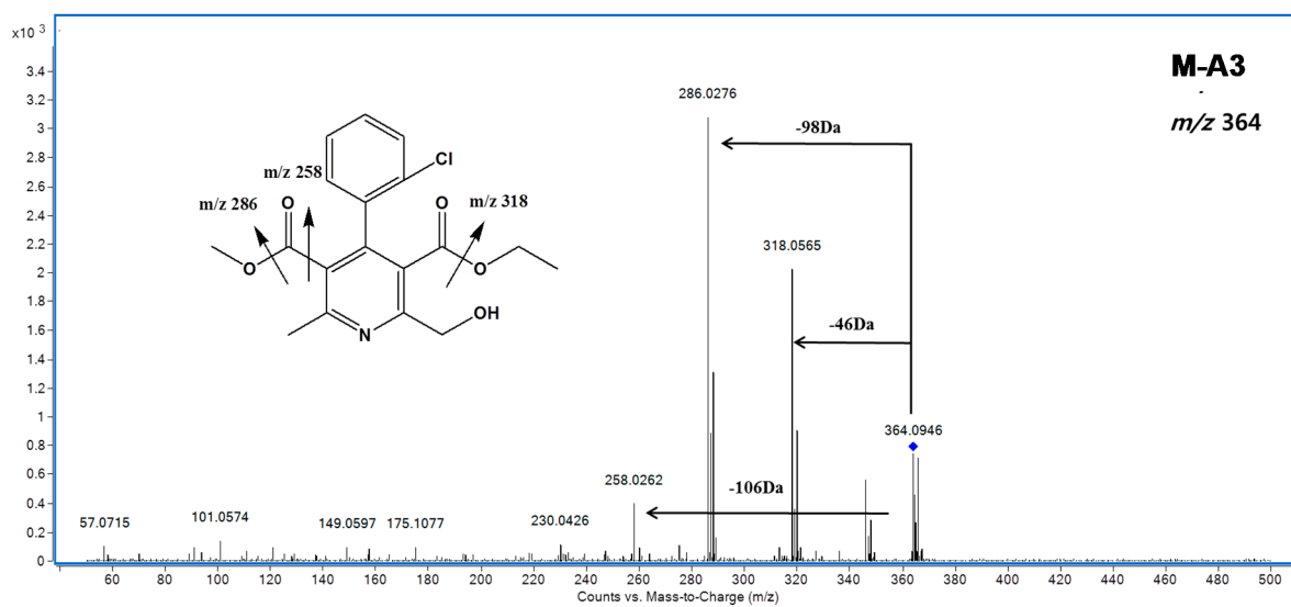
Figure S4. MS/MS spectrum of M-A3.
