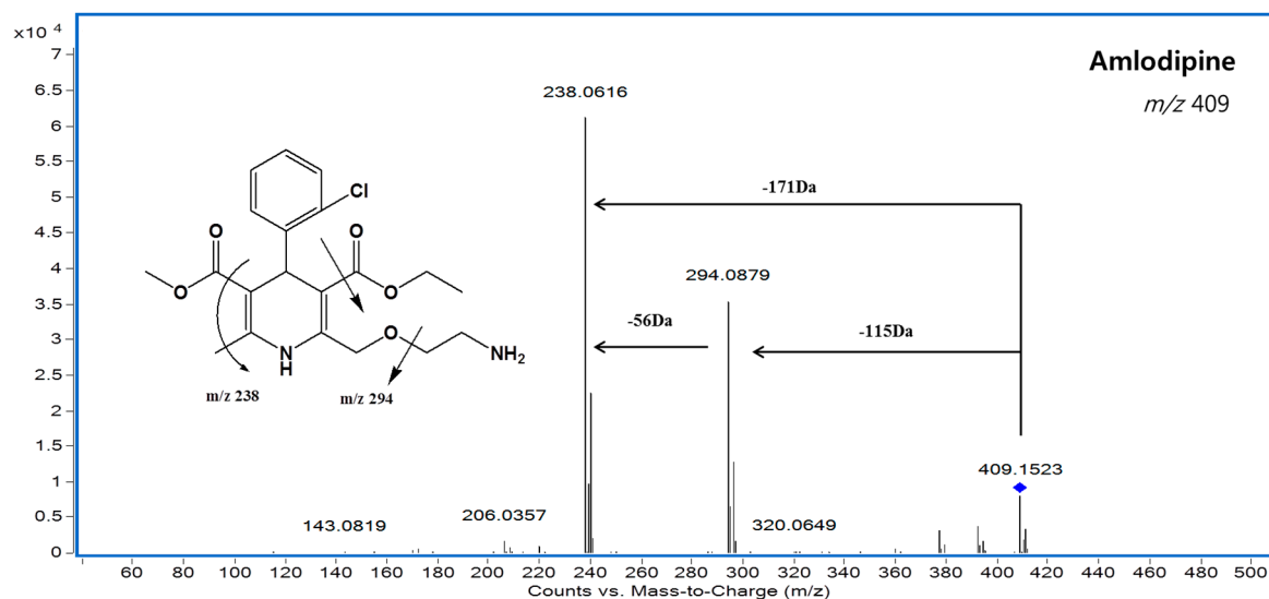
Figure S1. MS/MS spectrum of amlodipine.
