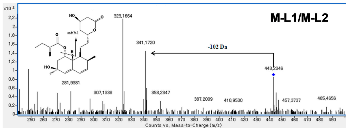
Figure S6. MS/MS spectrum of M-L1/M-L2.
