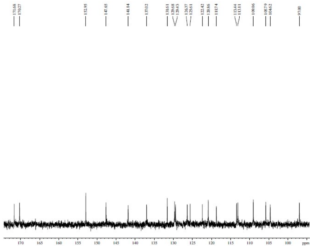
Figure 2. 13 C-NMR spectral of VIO (75 MHz, DMSO).
