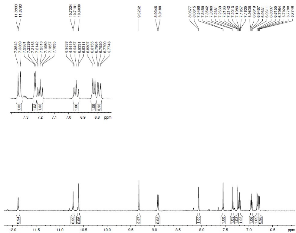
Figure 1. 1 H-NMR spectral of VIO (500 MHz, DMSO).
