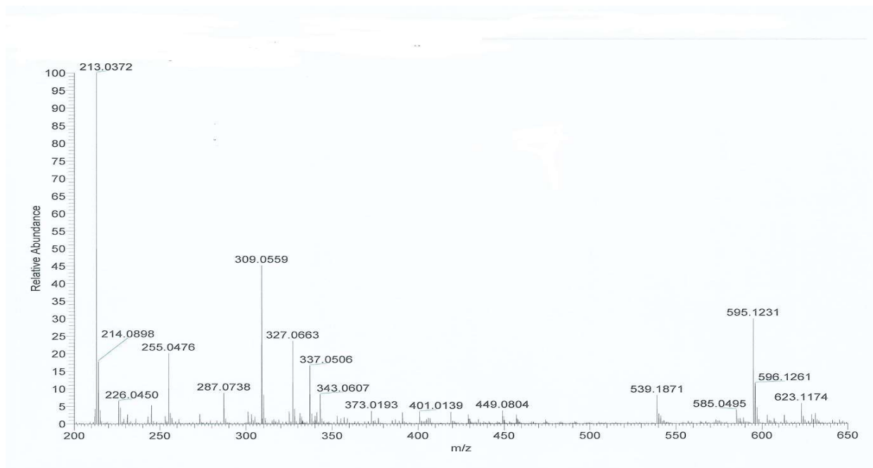
Figure T: MS spectrum of EH-6.
