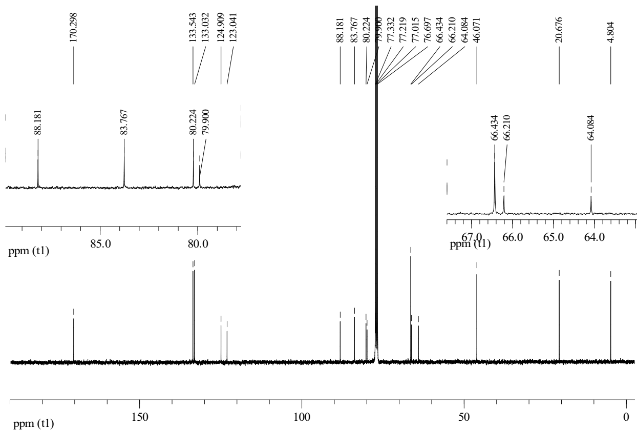
Figure D1: ^{13}\text{C} NMR spectrum of EH-7.
