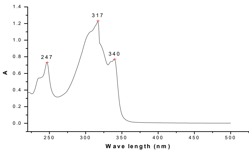
Figure J: UV spectrum of EH-2.
