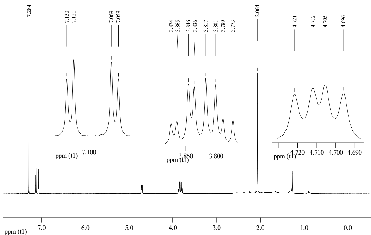
Figure D: 1 H NMR spectrum of EH-1.
