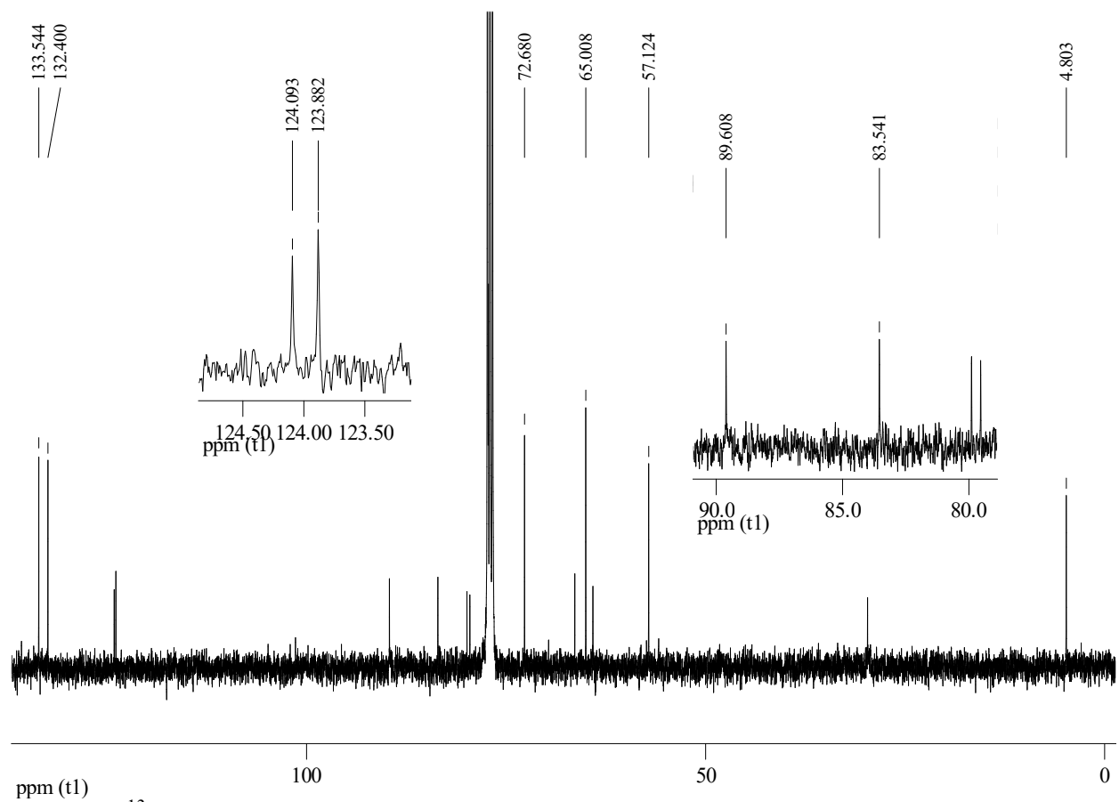
Figure L: ^{13}\text{C} spectrum of EH-2.
