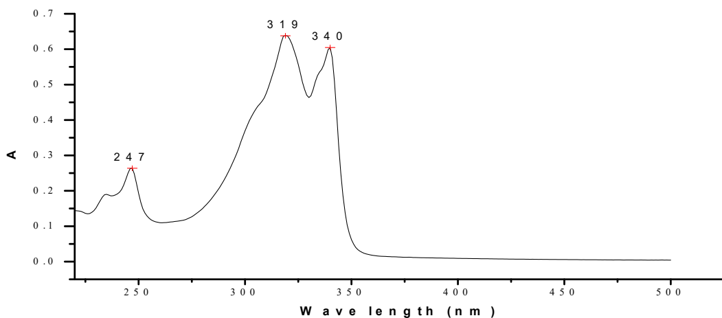
Figure V: UV spectrum of EH-6.
