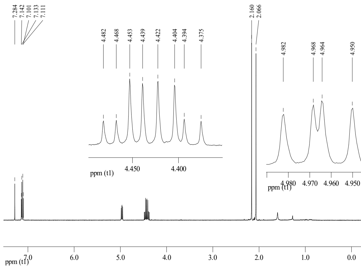
Figure C1: ^1\text{H} NMR spectrum of EH-7.
