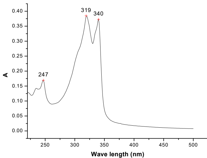
Figure C: UV spectrum of EH-1.
