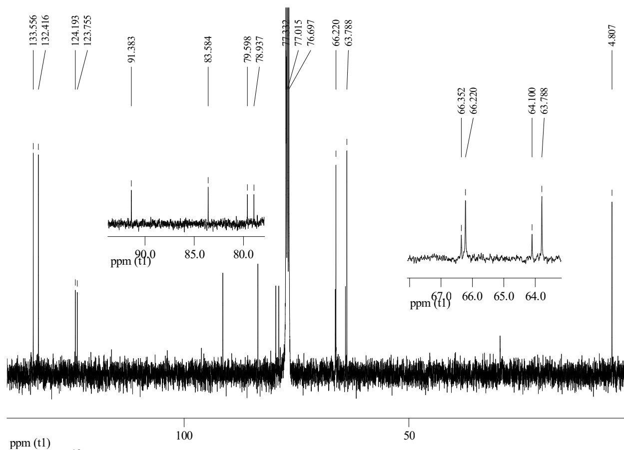
Figure E: ^{13}\text{C} NMR spectrum of EH-1.
