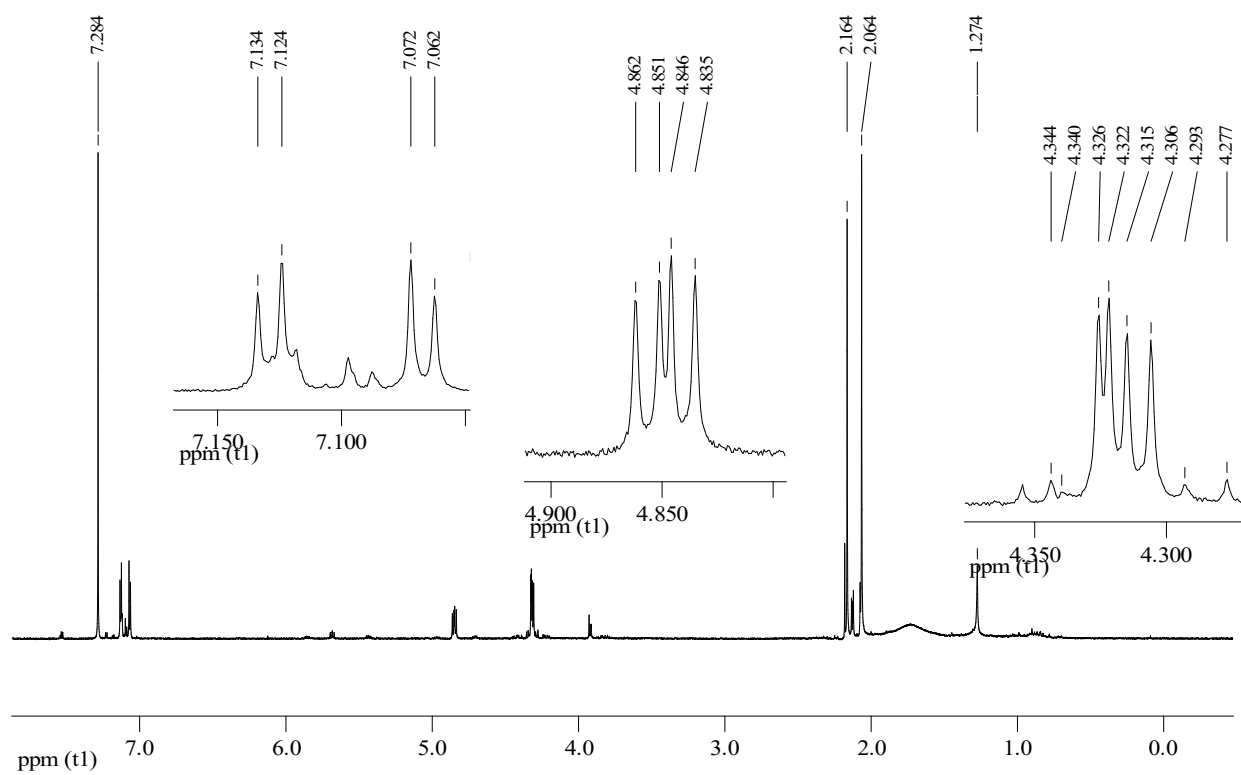
Figure Q: 1 H NMR spectrum of EH-3.
