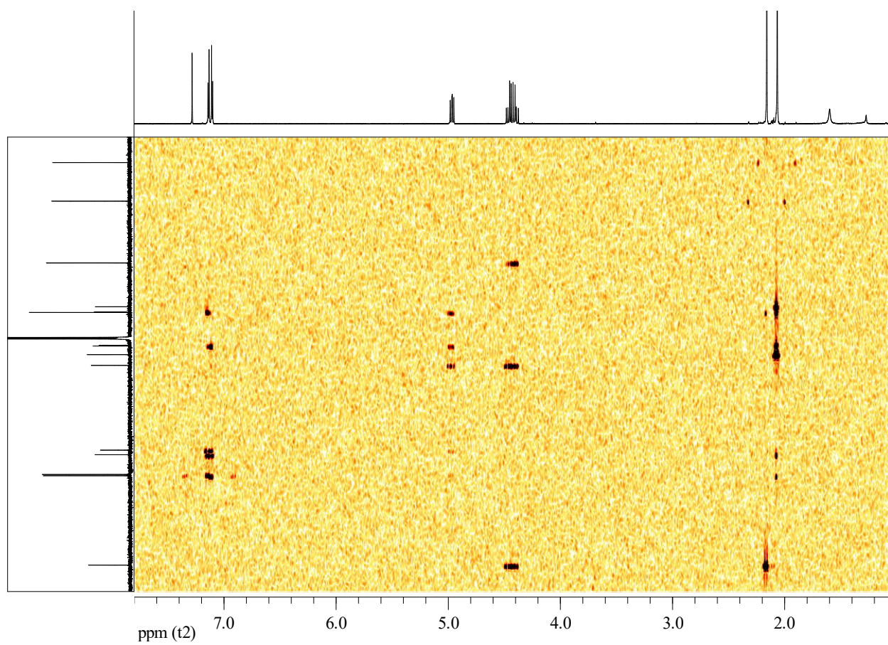
Figure F1: HMBC spectrum of EH-7.
