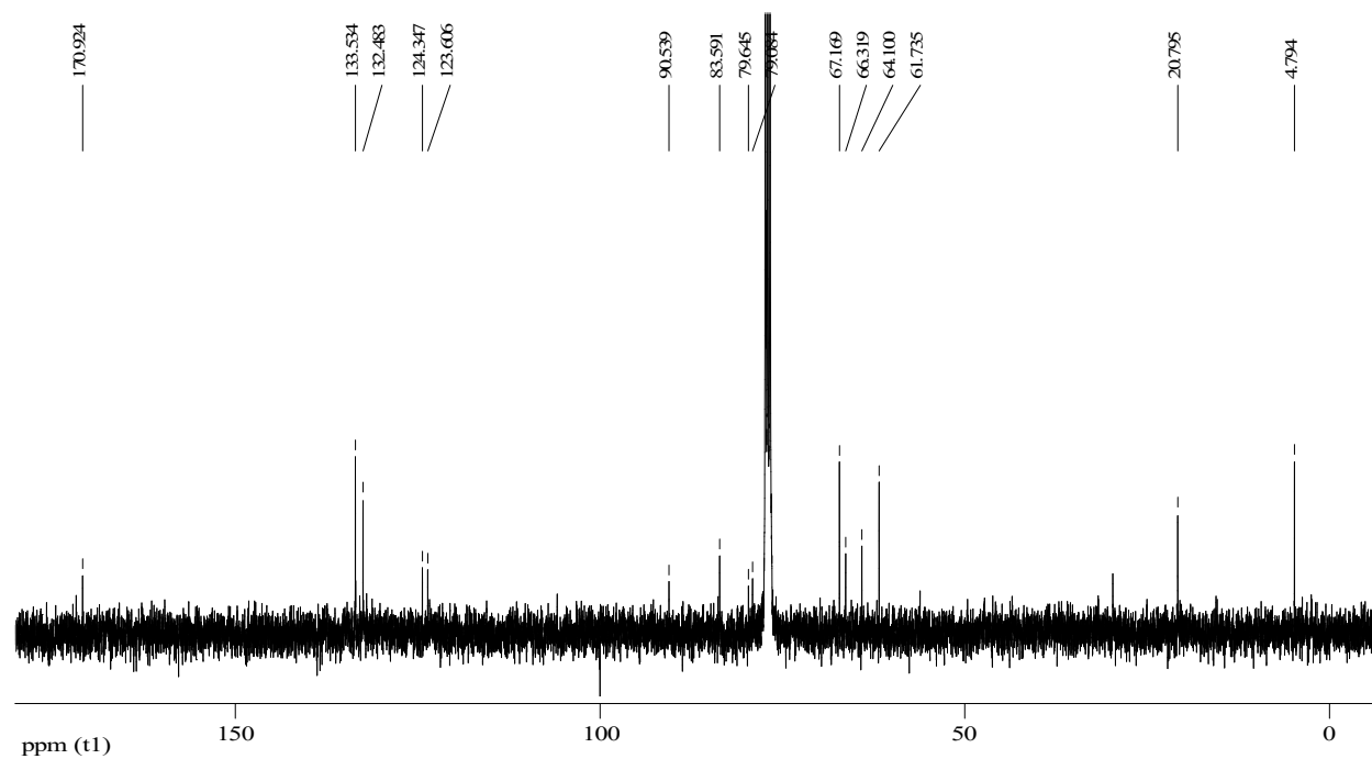
Figure R: ^{13}\text{C} NMR spectrum of EH-3.
