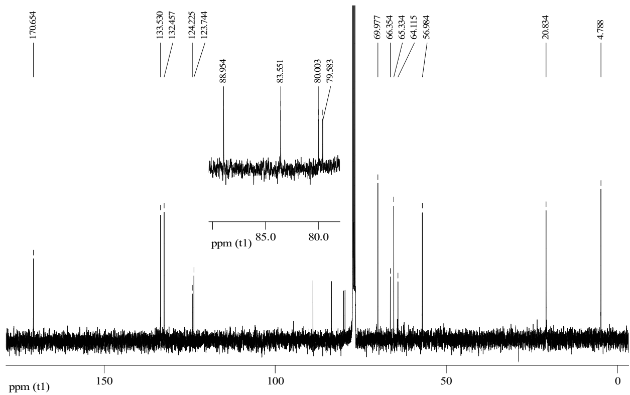
Figure X: ^{13}\text{C} NMR spectrum of EH-6.
