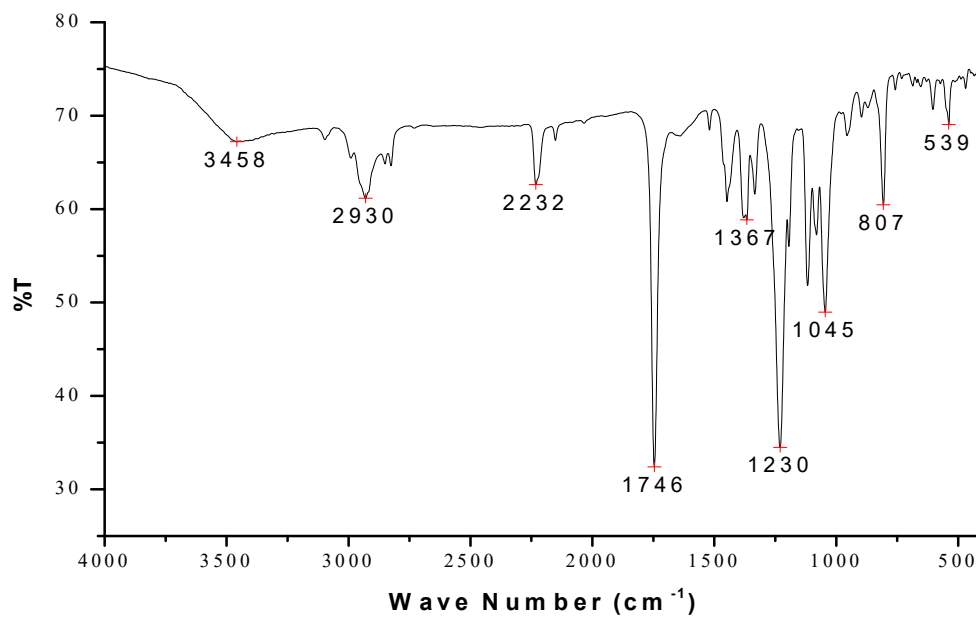
Figure U: IR spectrum of EH-6.
