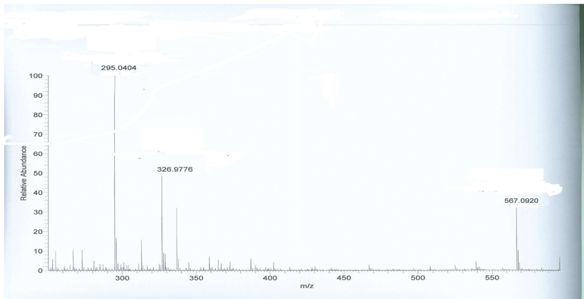
Figure N: MS spectrum of EH-3.
