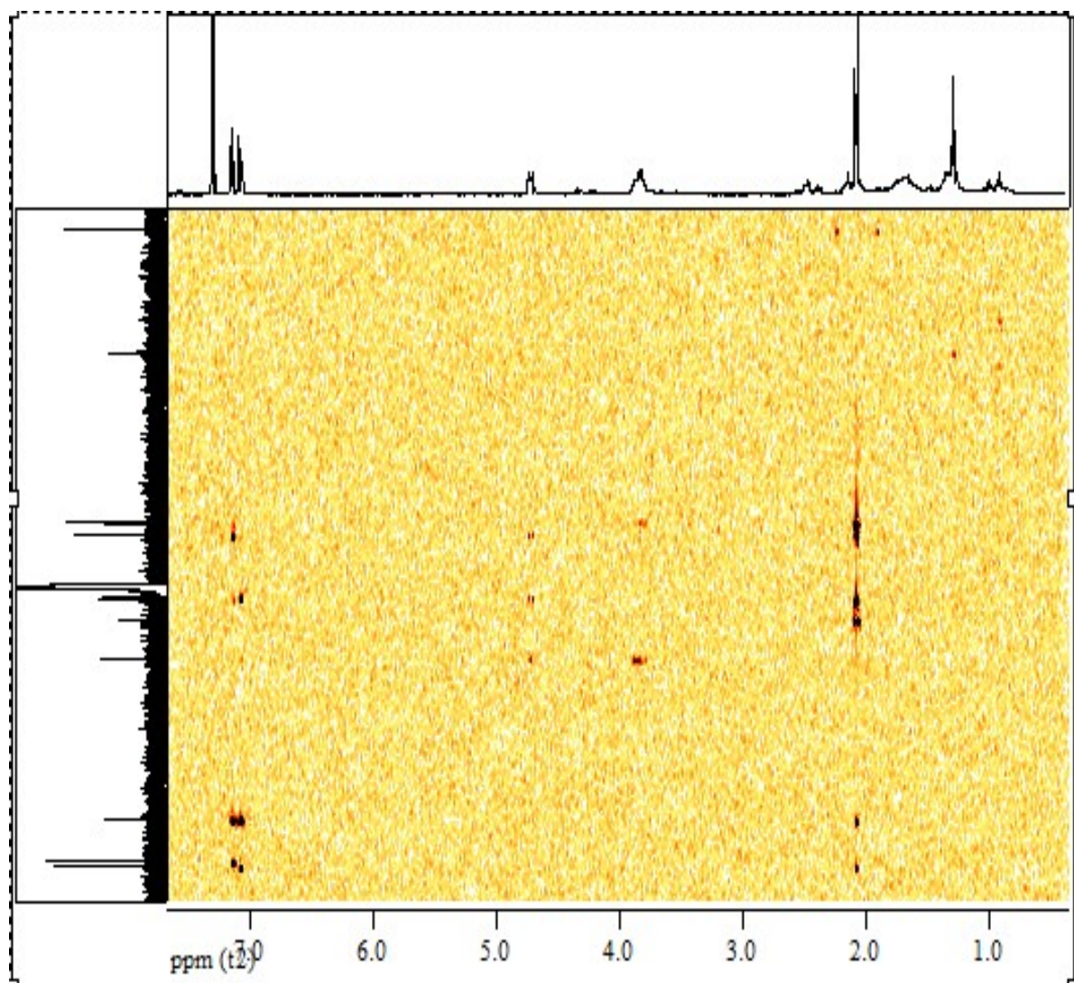
Figure G: HMBC spectrum of EH-1.
