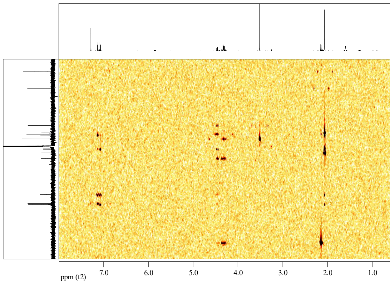
Figure Z: HMBC spectrum of EH-6.
