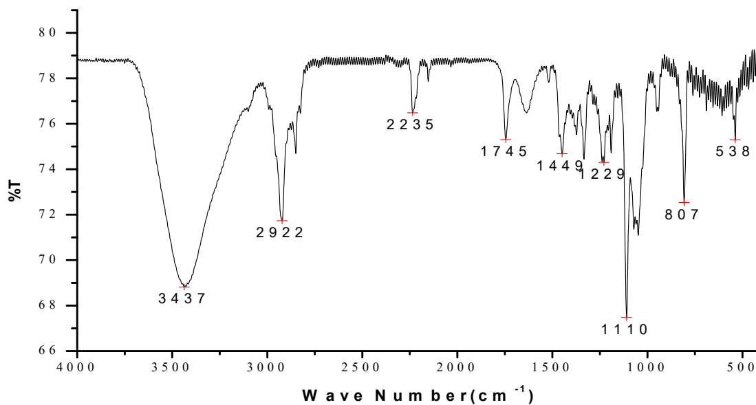
Figure H: MS spectrum of EH-2.
