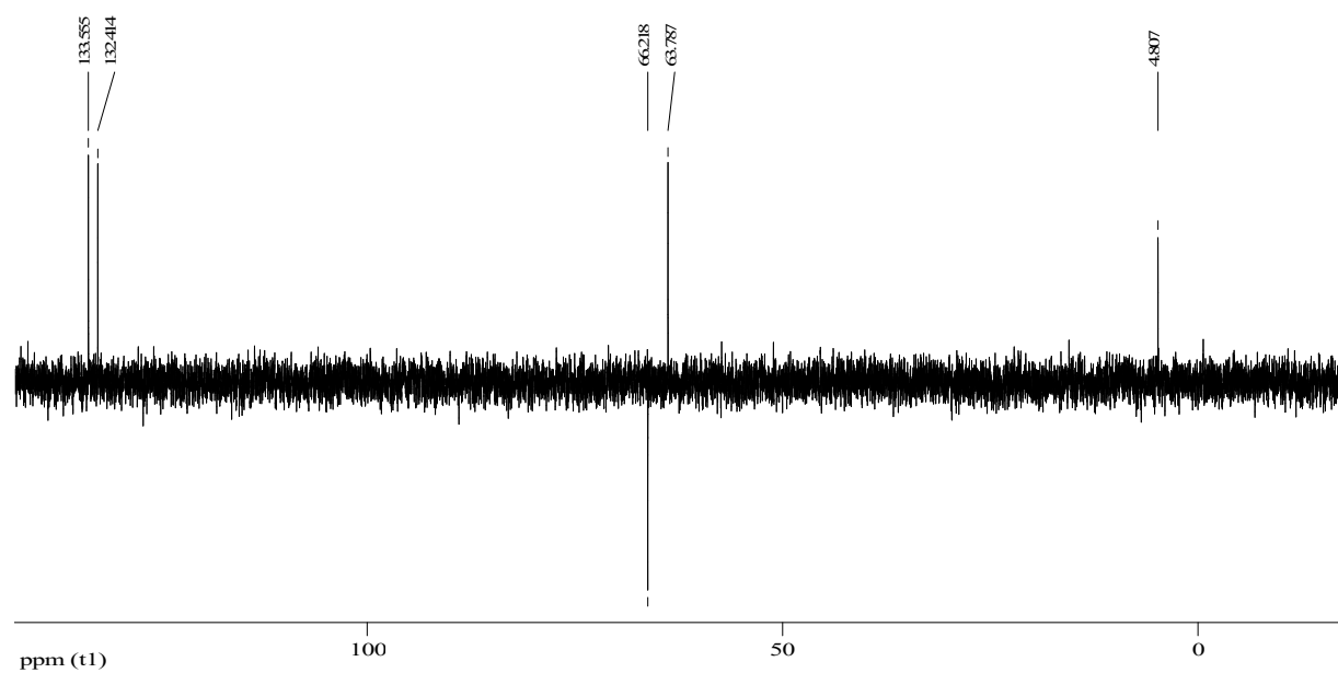
Figure F: DEPT-135 spectrum of EH-1.
