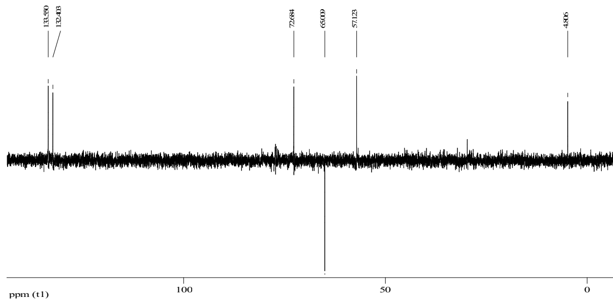
Figure M: DEPT-135 spectrum of EH-2.
