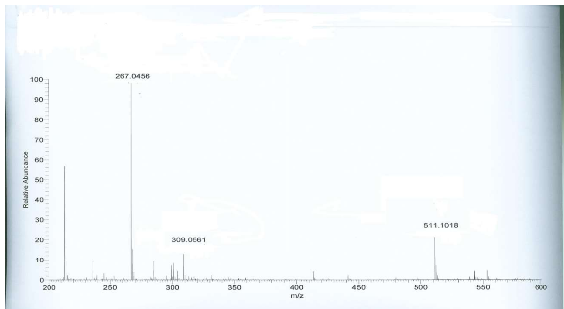
Figure H: MS spectrum of EH-2.
