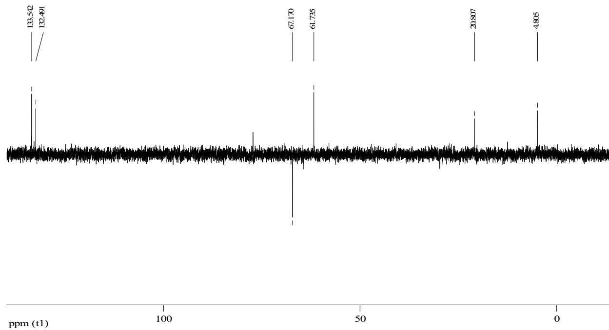
Figure S: DEPT-135 spectrum of EH-3.
