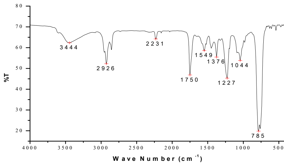
Figure O: IR spectrum of EH-3.
