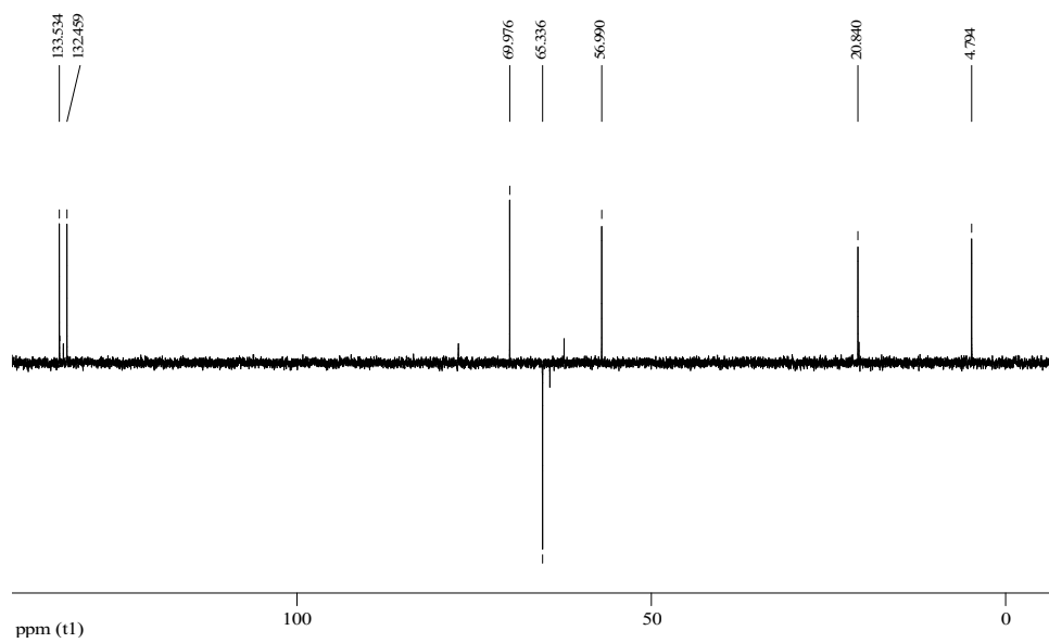
Figure Y: DEPT-135 spectrum of EH-6.
