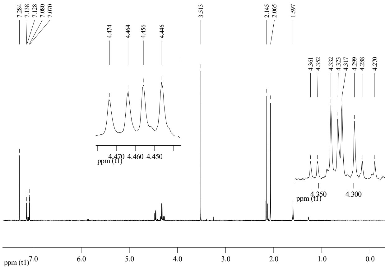
Figure W: ^1\text{H} NMR spectrum of EH-6.
