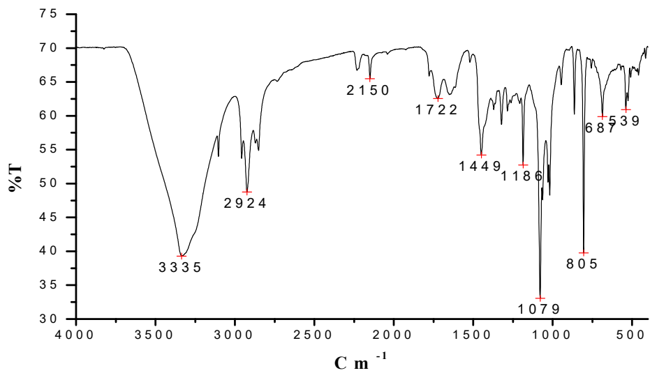
Figure B: IR spectrum of EH-1.
