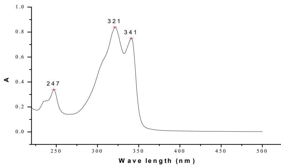
Figure B1: UV spectrum of EH-7.
