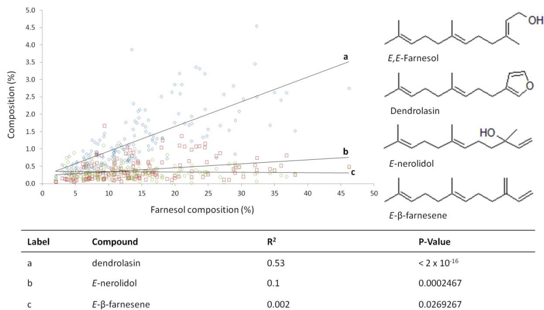
Figure S1. The linear correlation between E,E -farnesol, dendrolasin, E -nerolidol and E - \beta -farnesene based on GC-MS analysis 194 heartwood cores of S. spicatum trees in natural stands of Western Australia: 152 trees from the south-west (Wheatbelt), 19 trees from the south-east (Goldfields) and 23 trees from the north regions (Carnarvon and Shark Bay) using percent composition data.
