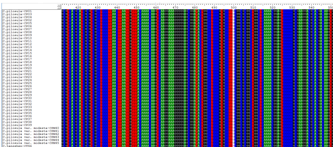
Fig. S1. The thumbnail picture of ITS sequences of 46 Codonopsis taxa specimens. The variable base sites were located at 122nd, 135th, 226th and 500th nucleotide positions respectively.
