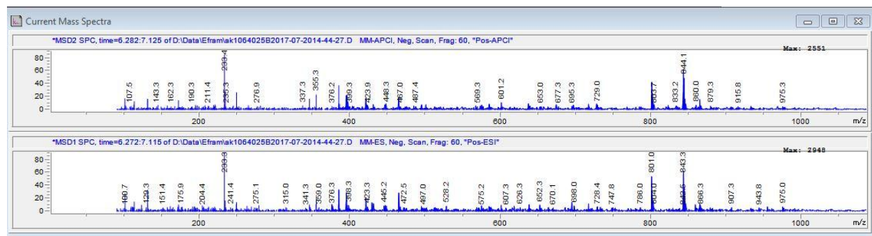
Figure S2. ESI and APCI mass spectra for compound 4: m/z: 844.22
