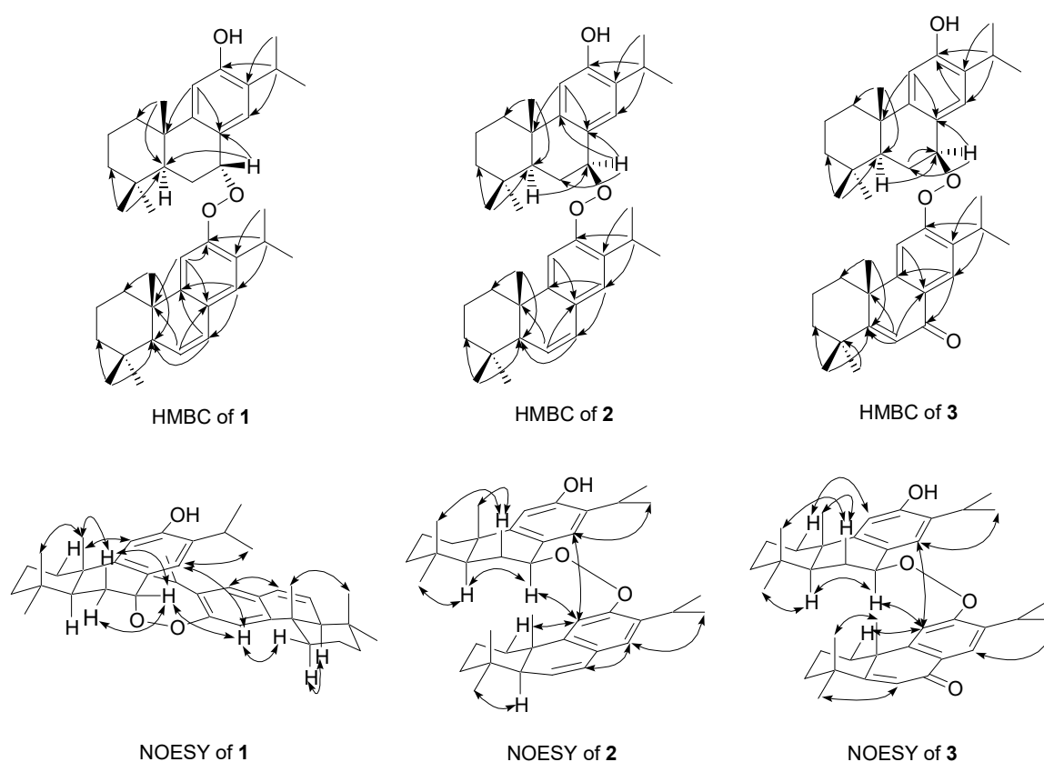
Figure 3. Significant HMBC (one-headed arrows) and NOESY (two-headed arrows) correlations of compounds 1 – 3 .
