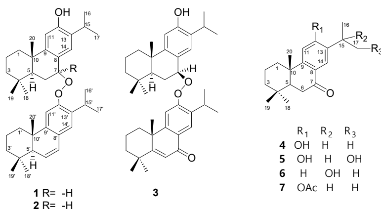
Figure 1. The chemical structures of compounds 1–7 isolated from C. japonica .
