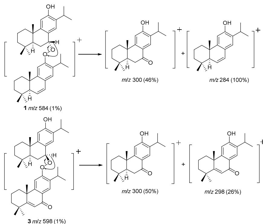
Figure 2. Some key electron impact (EI)-Mass fragmentations of compounds 1 and 3 .
