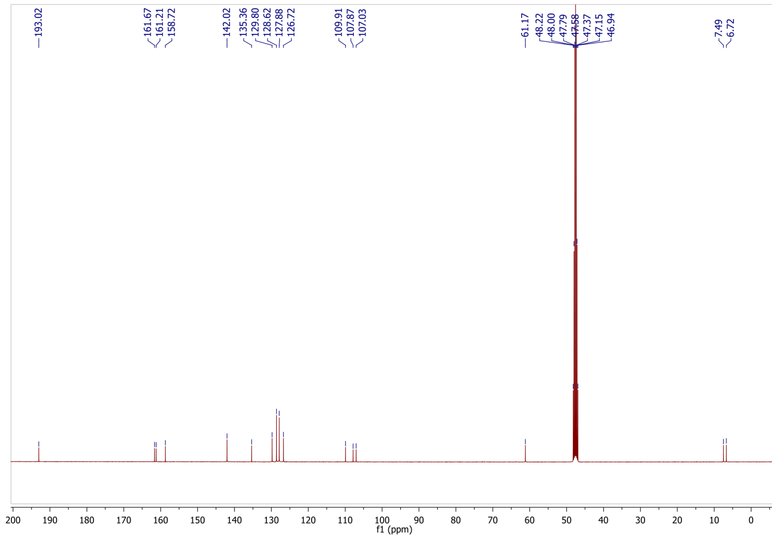
Figure 2. ^{13}\text{C} NMR of DCM (125 MHz, MeOD)
