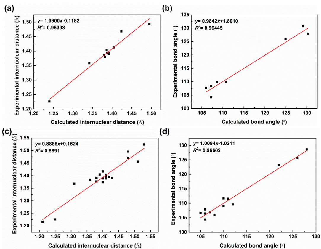
Figure S1. The correlation between computational and experimental data in literature of bond lengths and angles of indigo (a,b) and indirubin (c,d).
