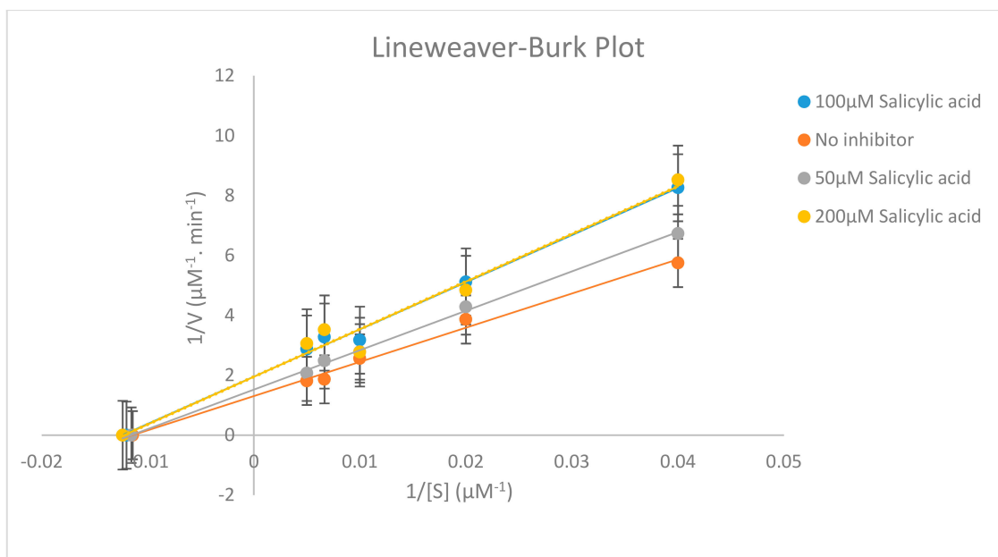
Figure 4. Lineweaver–Burk plot displaying the inhibition of CYP2C11 enzyme on the metabolism of testosterone into 16 \alpha -hydroxytestosterone using 0–200 \mu M salicylic acid. Each point represents averages of triplicate determinations.
