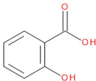
Figure 1. Structure of salicylic acid.
