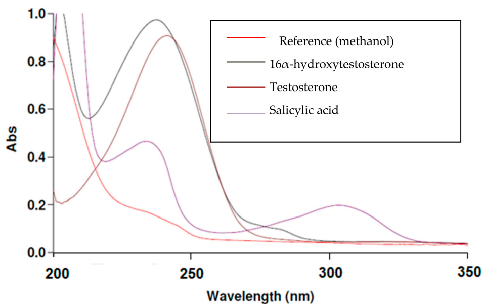
Figure 2. Overlain spectra of salicylic acid, testosterone and 16 \alpha -hydroxytestosterone components in the CYP2C11 assay.
