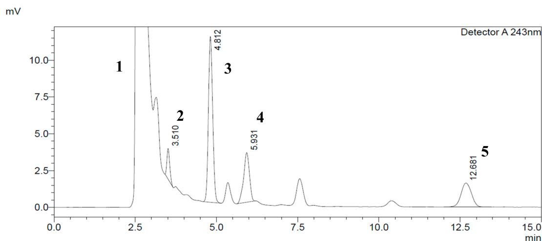
Figure 3. Typical HPLC chromatogram of CYP2C11 components in standard rat microsomal medium at 243 nm wavelength detection and a concentration of 150 \mu M testosterone. The peaks marked are: (1) NADPH (Nicotinamide Adenine Dinucleotide Phosphate Hydrogen)-regenerating system; (2) salicylic acid (100 \mu M); (3) phenacetin; (4) 16 \alpha -hydroxytestosterone; and (5) testosterone respectively.
