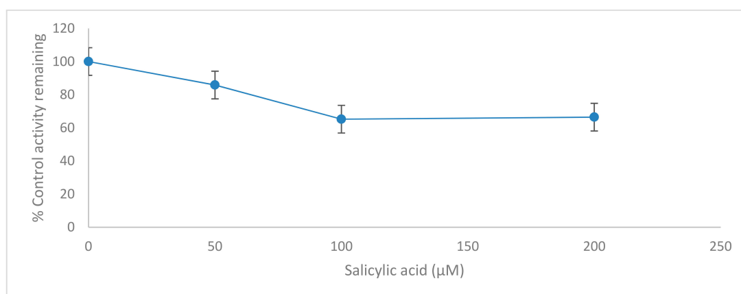
Figure 5. Inhibition of CYP2C11 isoform by salicylic acid (0–200 \mu M) in rat liver microsomes. Data represent averages of triplicates and are expressed as percentage of remaining control activity.
