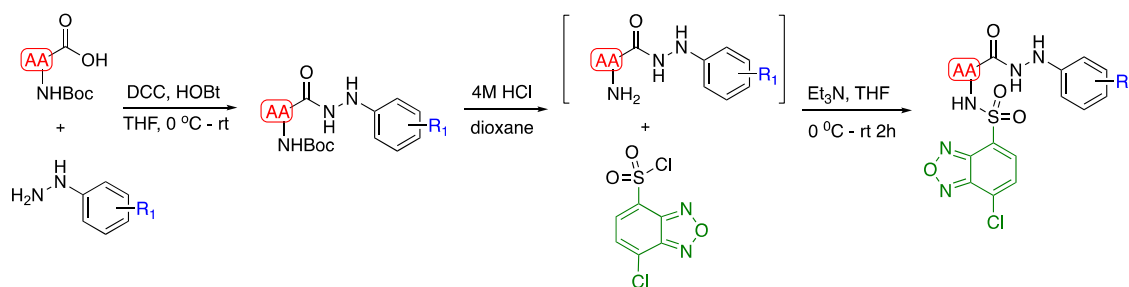
Scheme 1. Synthesis of amino acid hydrazides and the desired benzoa-[2,1,3]-diazole amino acid hydrazides.
