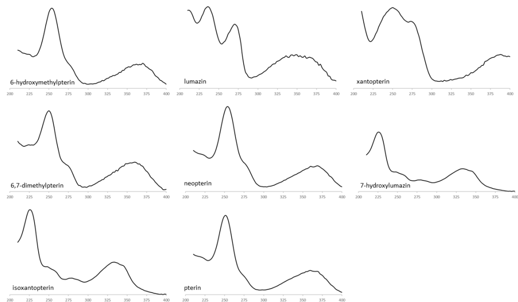
Figure S1. UV absorbance spectra of the selected analytes.
