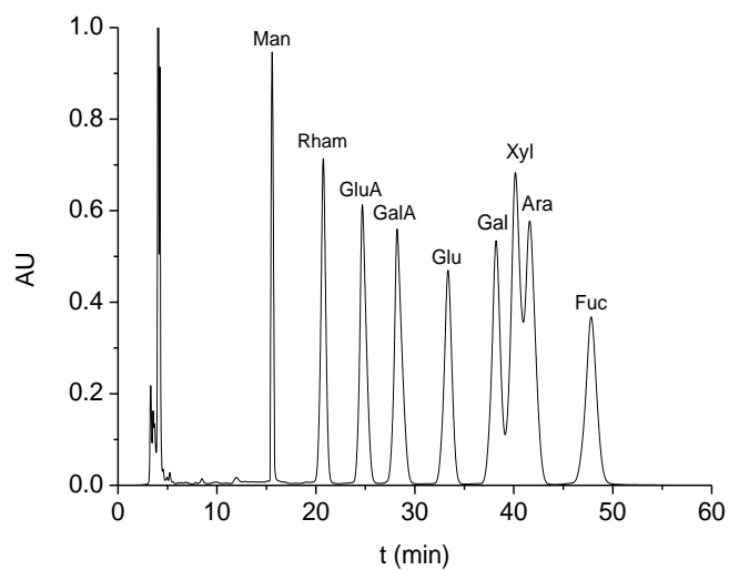
Figure S1. The elution curve of PMP derivatives of mixed monosaccharide standards hydrolysate by HPLC
