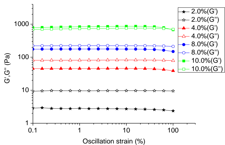
Figure S2. Strain dependency of shear modulus G' (storage) and G'' (loss) of TSP at different concentrations at 25 °C
