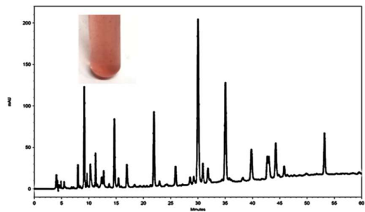
Figure S1. Chromatographic profiles and appearance of acid hydrolysis resultant (1 N HCl, 121 °C for 30 min) of SPEI 's acetone-soluble fraction (ASfr). SPEI , substances with pectin methylesterase inhibitory activity.
