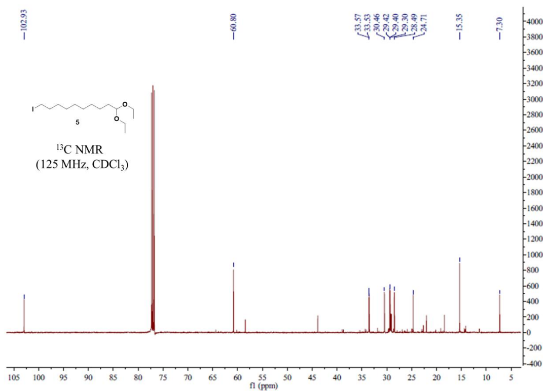
The 13 C NMR spectrum of compound 5
