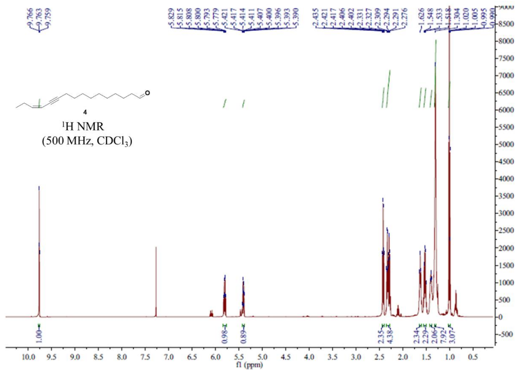
The 1 H NMR spectrum of compound 4
