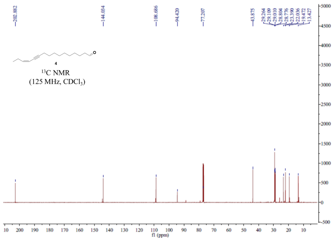
The 13 C NMR spectrum of compound 4
