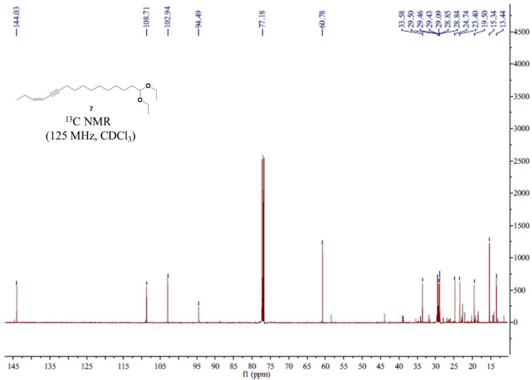
The 13 C NMR spectrum of compound 7
