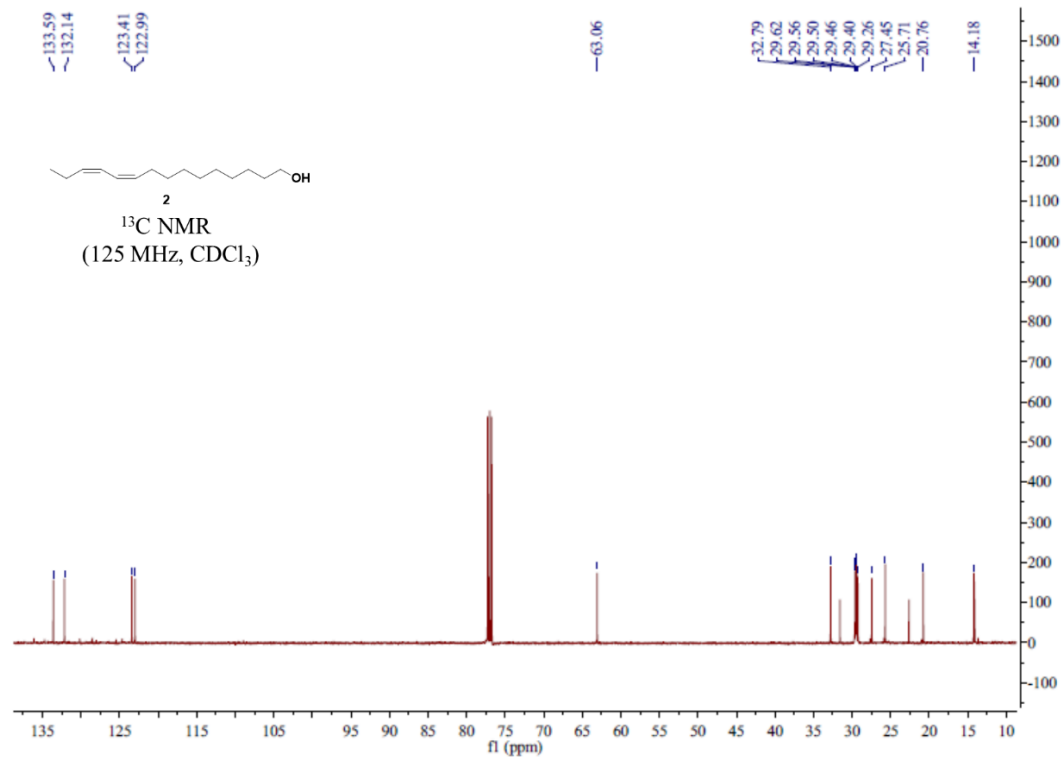
The 13 C NMR spectrum of compound 2
