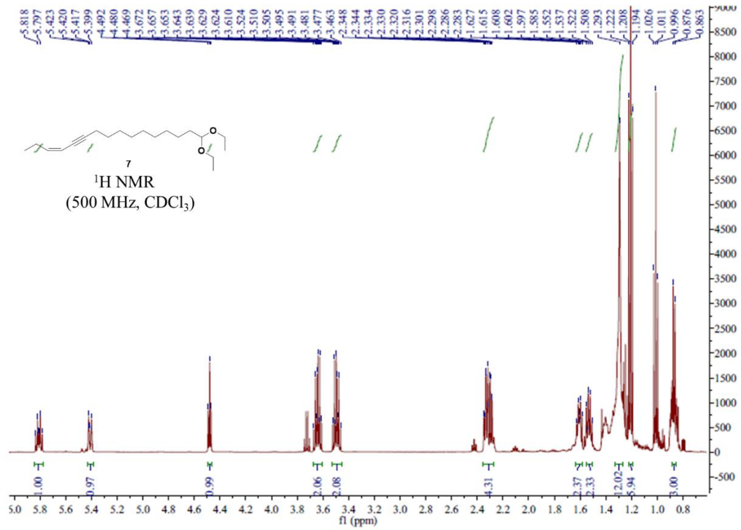
The 1 H NMR spectrum of compound 7
