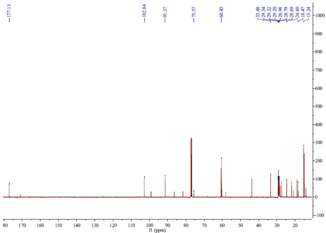
The 13 C NMR spectrum of compound 6
