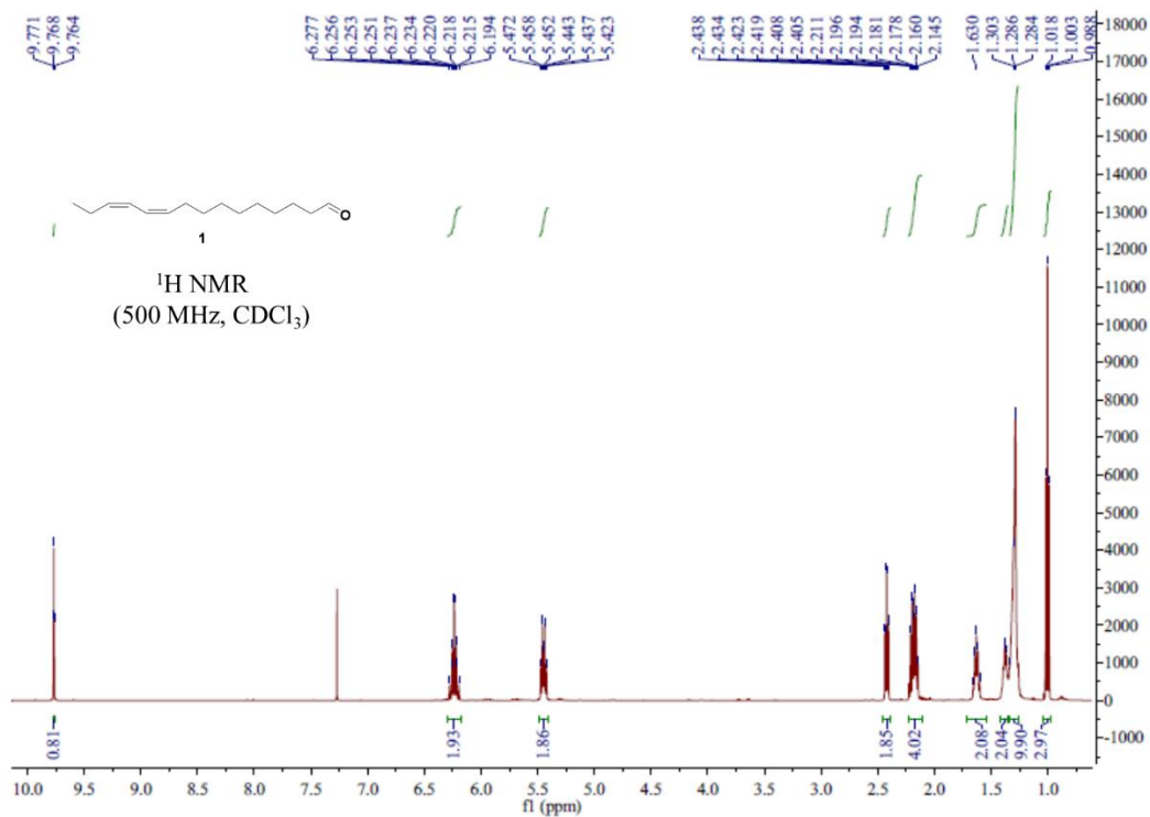
The 1 H NMR spectrum of compound 1
