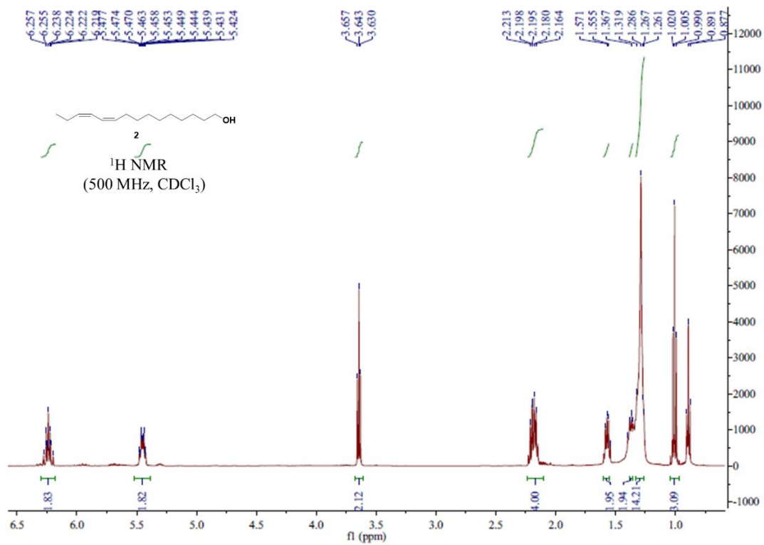
The 1 H NMR spectrum of compound 2
