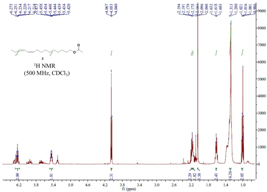
The 1 H NMR spectrum of compound 3
