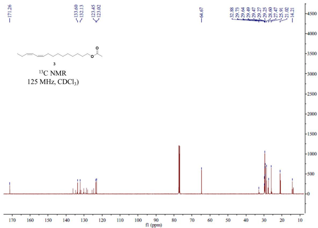
The 13 C NMR spectrum of compound 3
