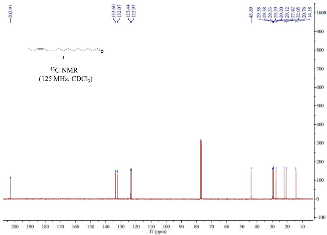
The 13 C NMR spectrum of compound 1
