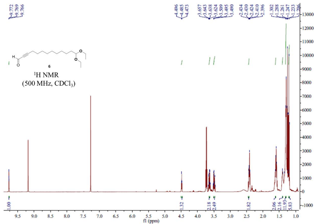
The 1 H NMR spectrum of compound 6
