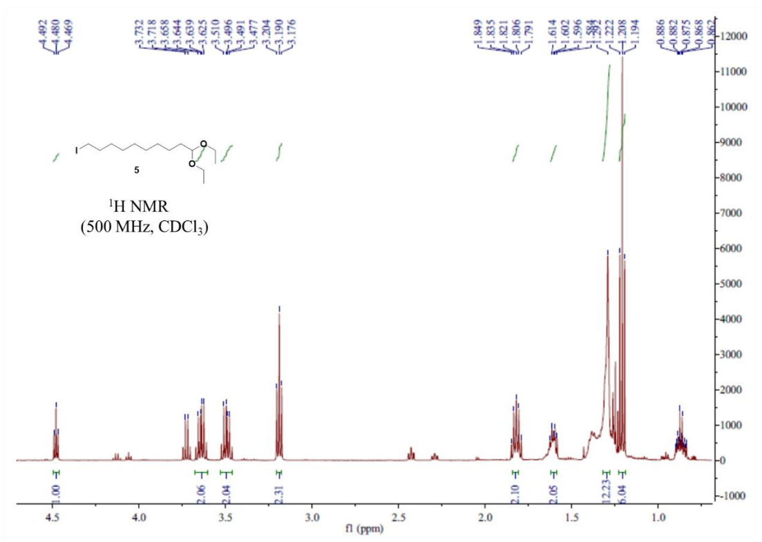
The 1 H NMR spectrum of compound 5
