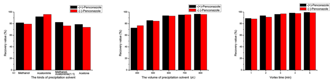
Figure S1. The optimization of PPT sample pretreatment method for penconazole enantiomers.
