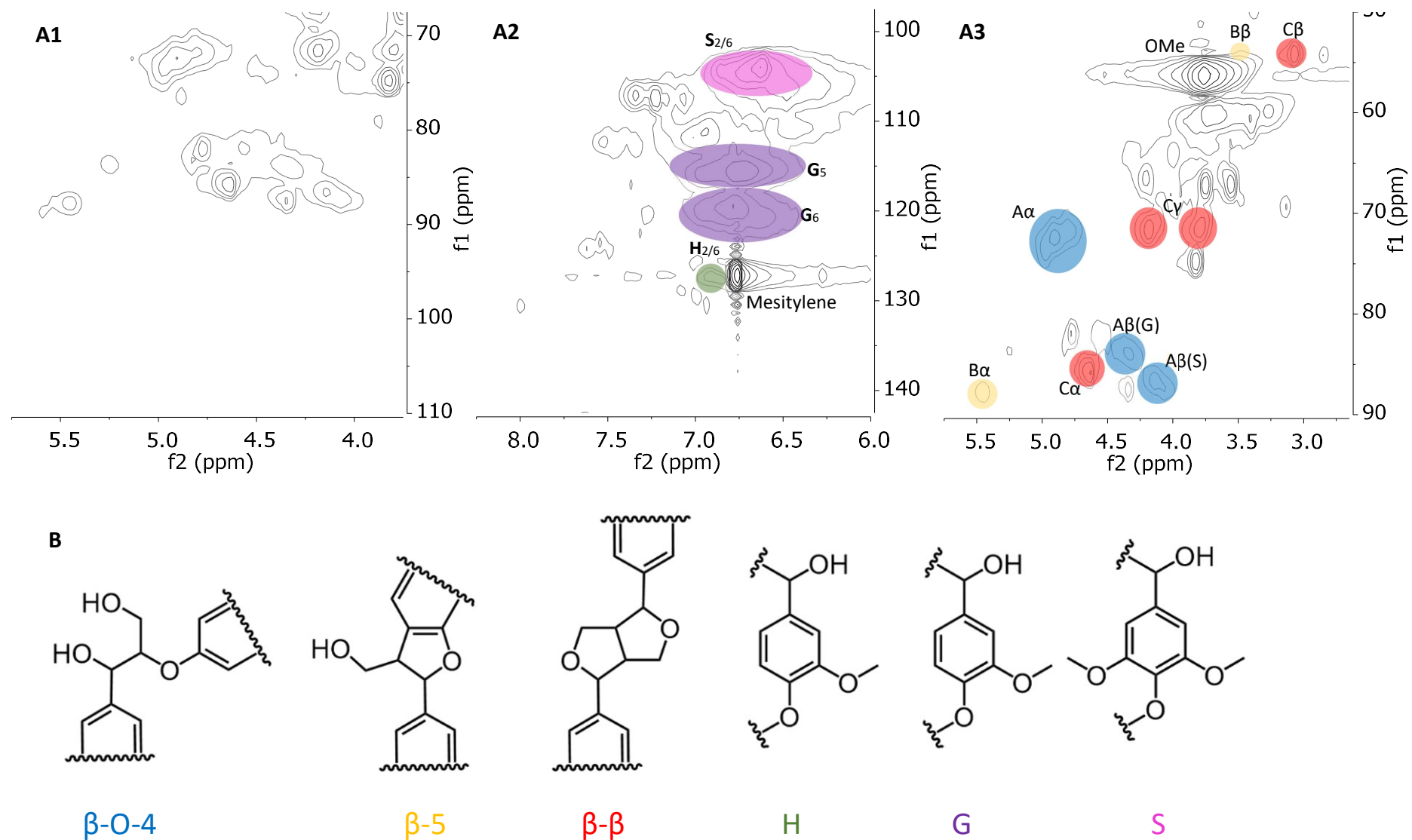
Figure S1: Expansion of HSQC NMR spectrum of OrganoCat lignin, A1 (carbohydrate region), A2 (lignin region) and A3 (aliphatic region), B investigated linkages and monomer units.
