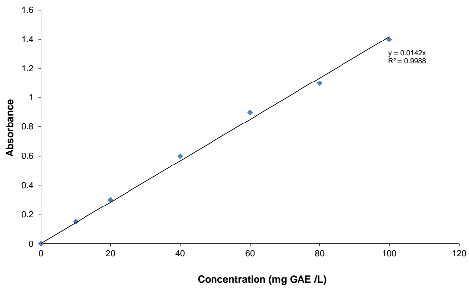
Figure S1. Gallic acid standard curve for total phenolic content.
