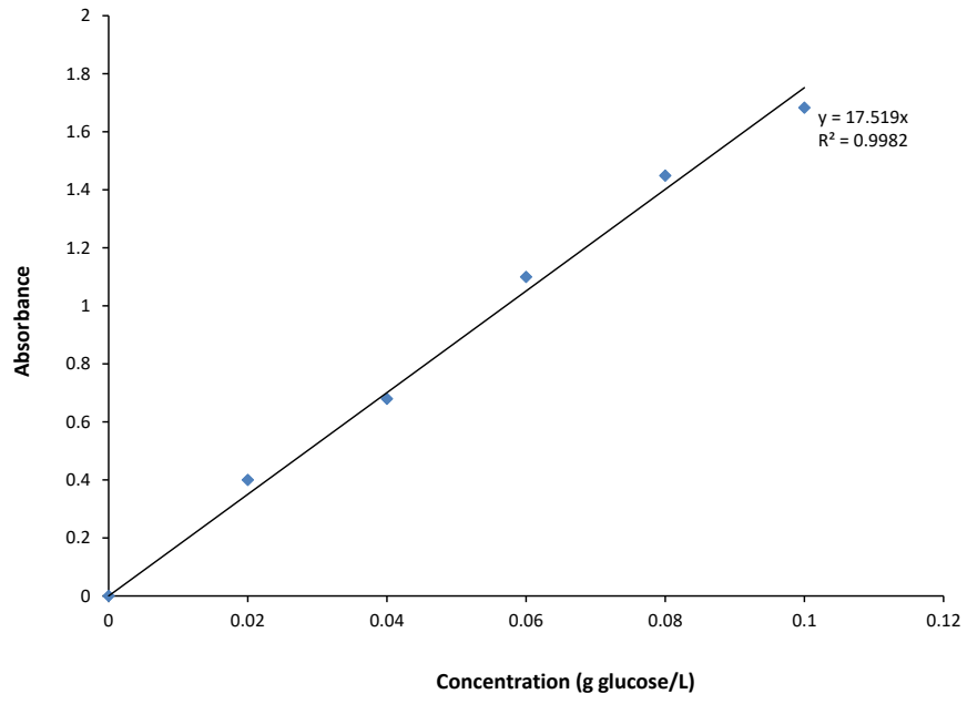
Figure S3. Standard curve of total carbohydrate content.
