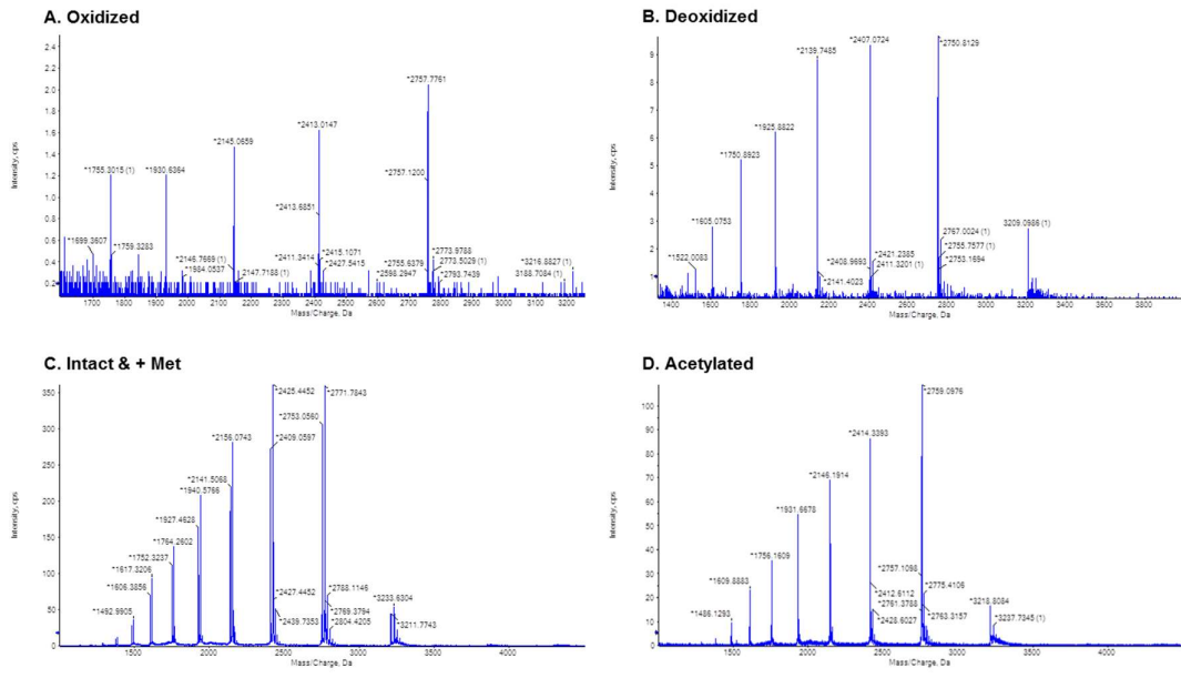
Figure S1. Non-deconvoluted mass spectra of IFN \alpha 2b variants. A. Spectrum from 14.095 to 14.420 min of sample 6P. B. Spectrum from 15.927 to 16.098 min of sample 7Y. C. Spectrum from 16.509 to 16.920 min of sample 6P. D. Spectrum from 17.246 to 17.588 min of sample 6P.
