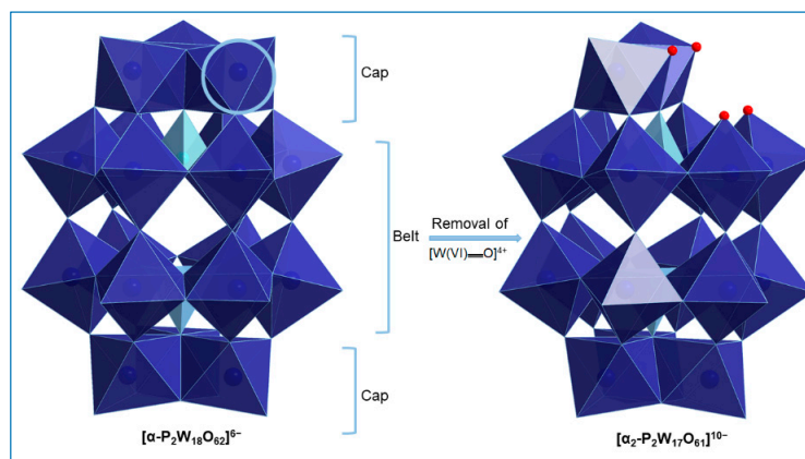
Figure 2. Formation of the [\alpha\text{-}2\text{-P}_2\text{W}_{17}\text{O}_{61}]^{10-} isomer by removal of a [\text{W}(\text{VI})=\text{O}]^{4+} unit from the “cap” segment of the parent [\alpha\text{-P}_2\text{W}_{18}\text{O}_{62}]^{6-} anion. Color code: \text{WO}_6 blue octahedra, \text{PO}_4 sky blue tetrahedra, O red spheres.
