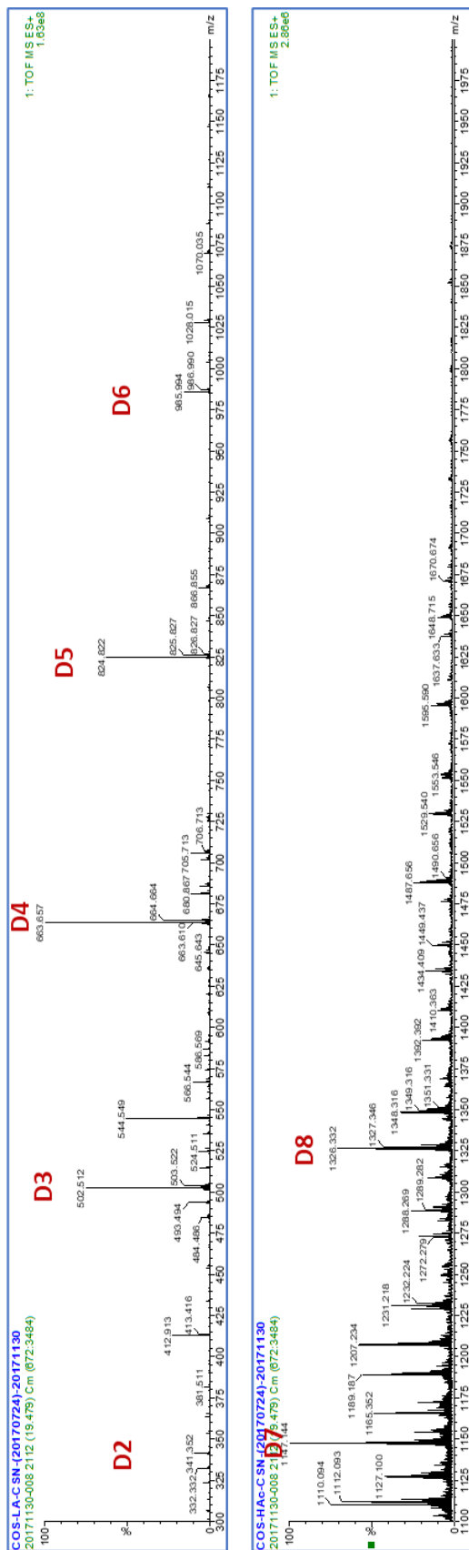
Figure S1. The characterization of COS by UPLC-Q TOF MS spectrometry in the positive ion mode.
