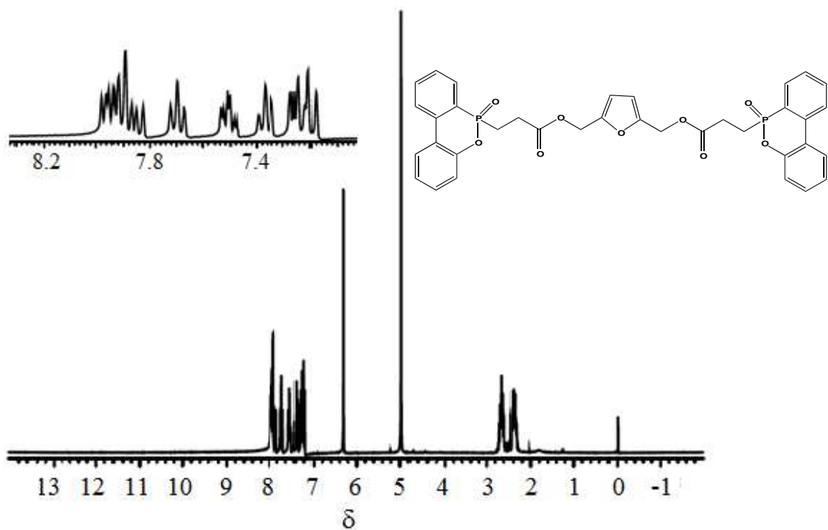
Figure S24. The ^1\text{H} NMR Spectrum for 2,5-Di[(3-dopylpropanoyl)methyl]furan (DDMF)
