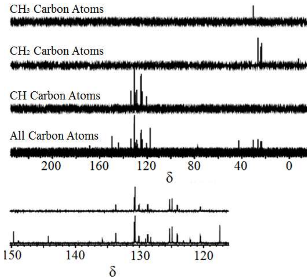
Figure S15. The DEPT NMR Spectrum for 2,2-Di[3,5-dibromo-4-(3-dopylpropanoyl)phenyl]propane (DBDPP).
