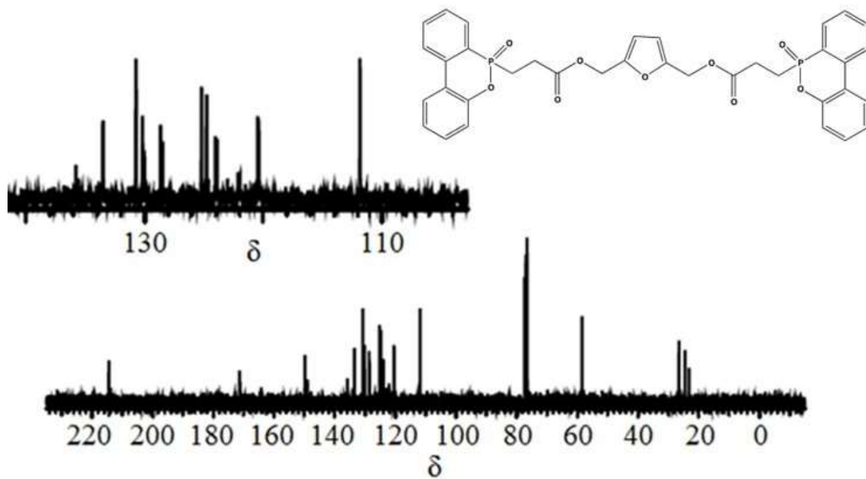
Figure S26. The ^{13}\text{C} NMR Spectrum for 2,5-Di[(3-dopylpropanoyl)methyl]furan (DDMF)
