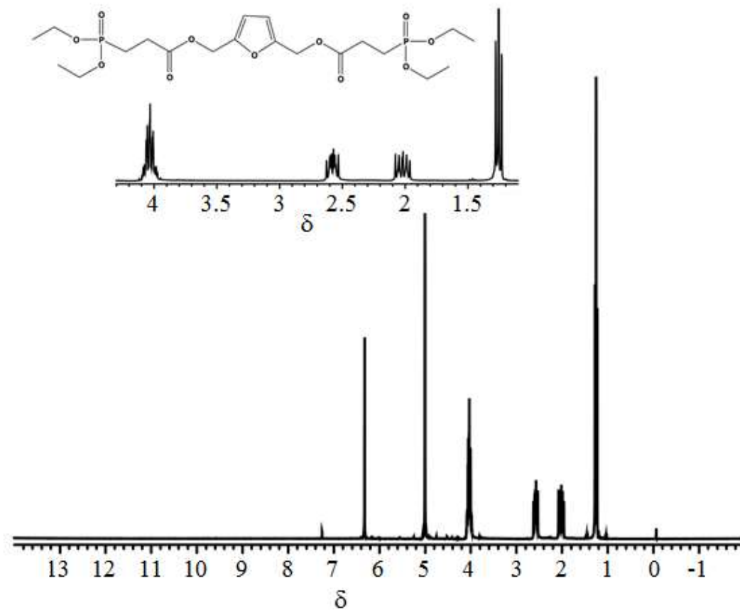
Figure S31. The 1 H NMR Spectrum for Di[(3-diethylphosphonatopropanyl)methyl]furan (DEMF)
