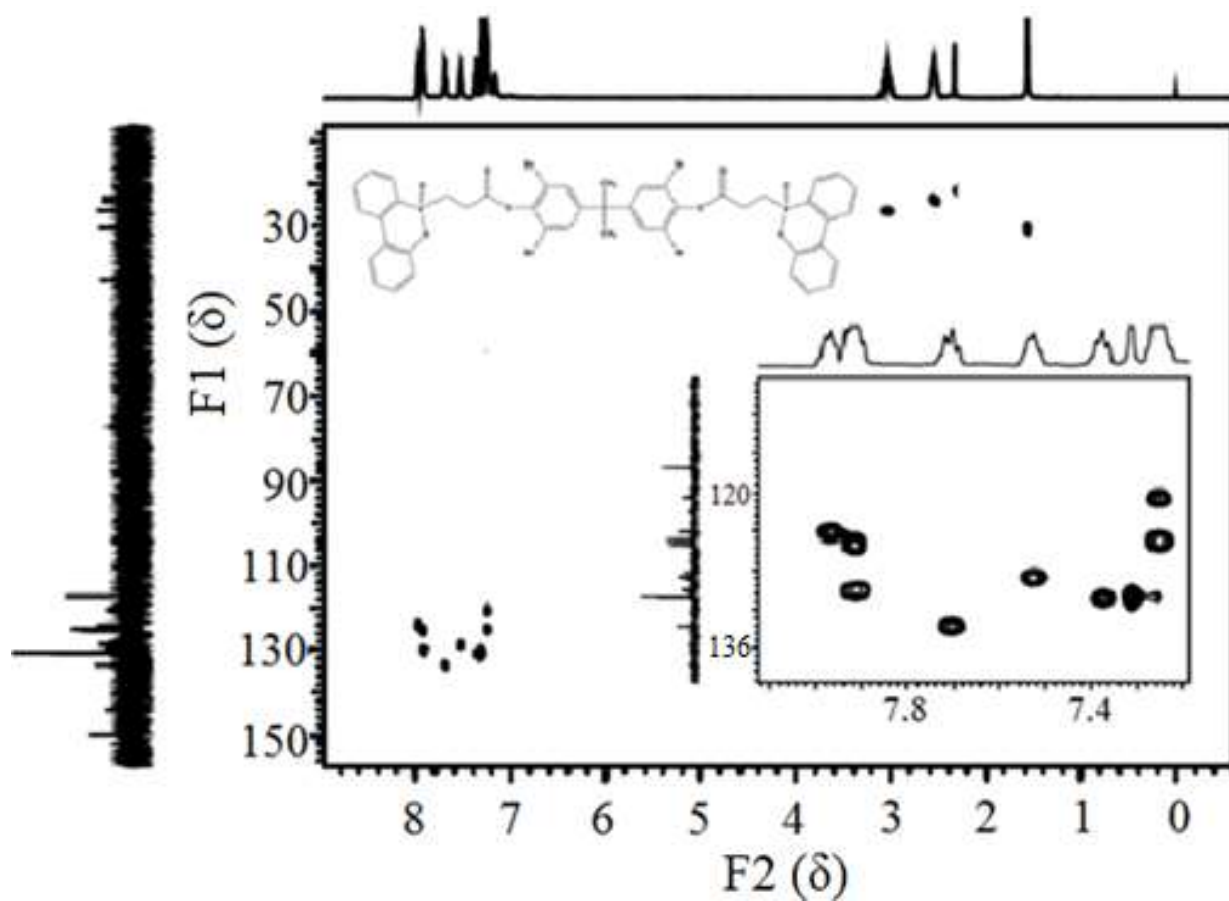
Figure S17. The HSQCAD NMR Spectrum for 2,2-Di[3,5-dibromo-4-(3-dopylpropanoyl)phenyl]propane (DBDPP).
