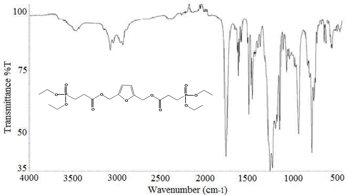
Figure S33. The Infrared Spectrum of Di[(3-diethylphosphonatopropanoyl)methyl]furan (DEMF)
