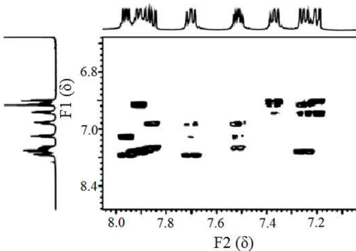
Figure S25. The gCOSY NMR Spectrum for 2,5-Di[(3-dopylpropanoyl)methyl]furan (DDMF)
