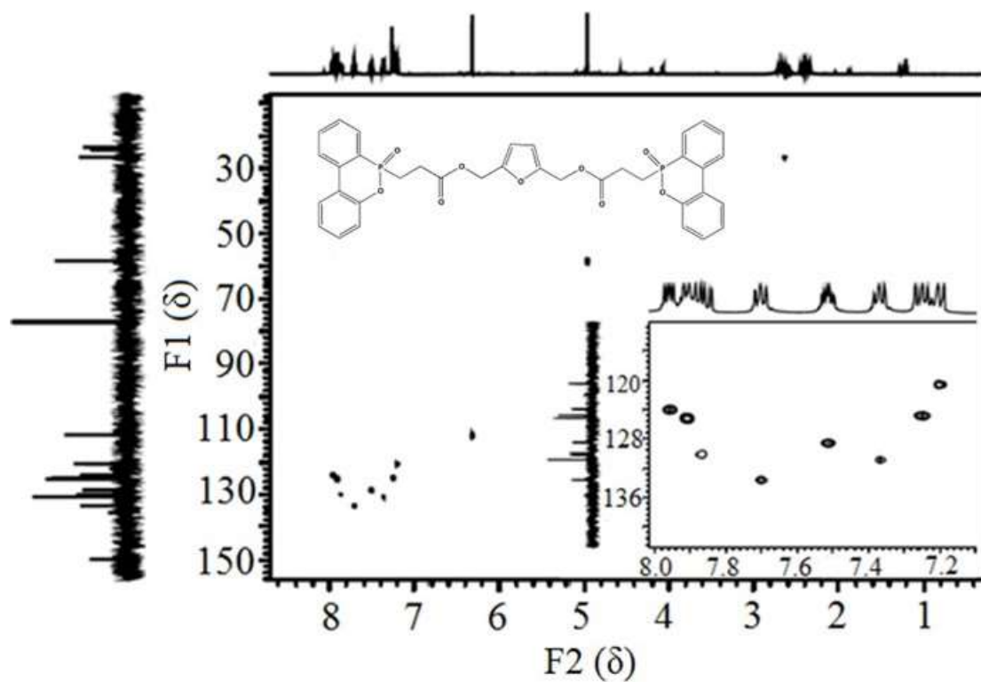
Figure S28. The HSQCDA NMR Spectrum for 2,5-Di[(3-dopylpropanoyl)methyl]furan (DDMF)
