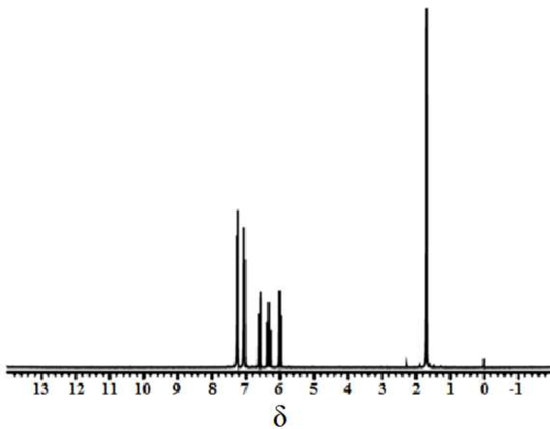
Figure S1. The ^1\text{H} NMR Spectrum for Bisphenol A Diacrylate (BPADA)
