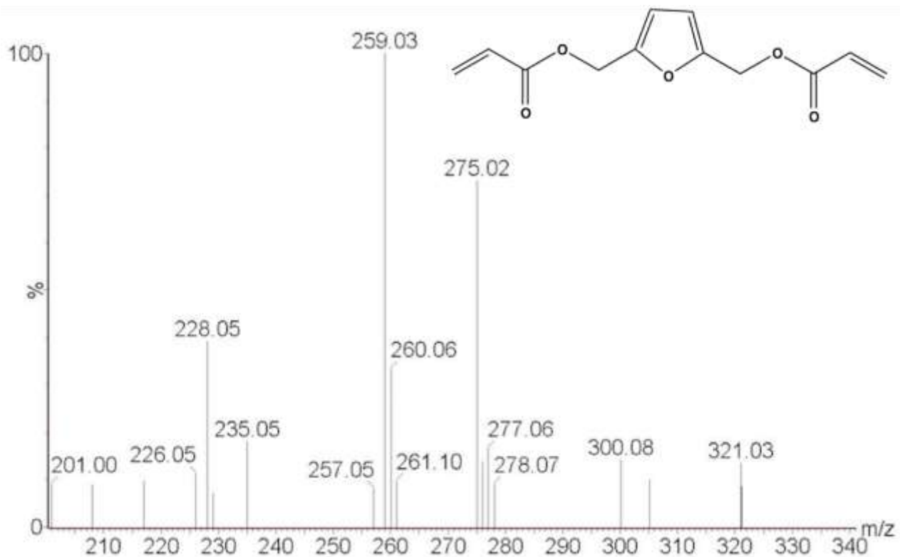
Figure S23. Mass Spectrum for 2,5-bis-(Hydroxymethyl)furan Diacrylate (BHFDA)
