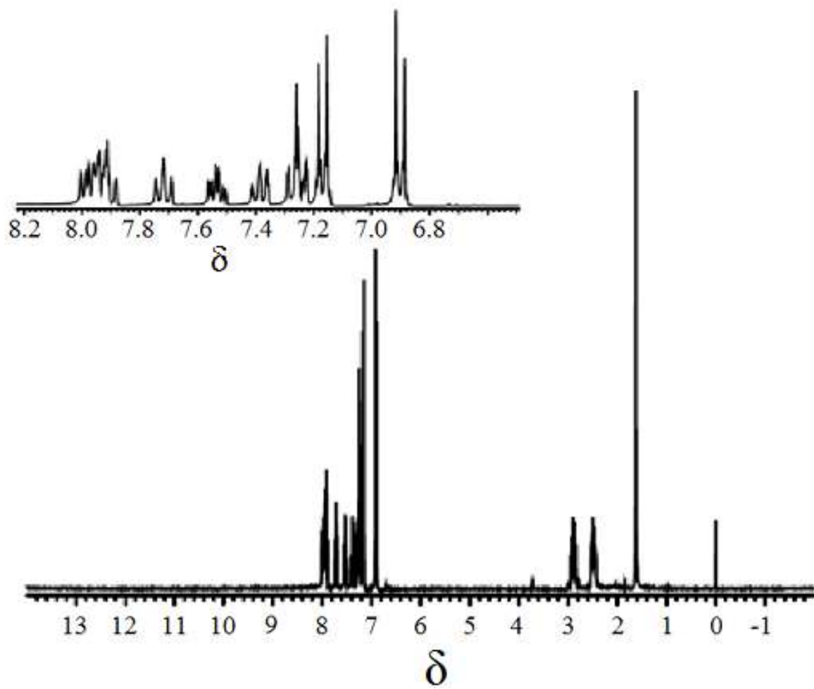
Figure S4. The 1 H NMR Spectrum of 2,2-Di[4-(3-dopylpropanoyl)phenyl]propane (DDPP)
