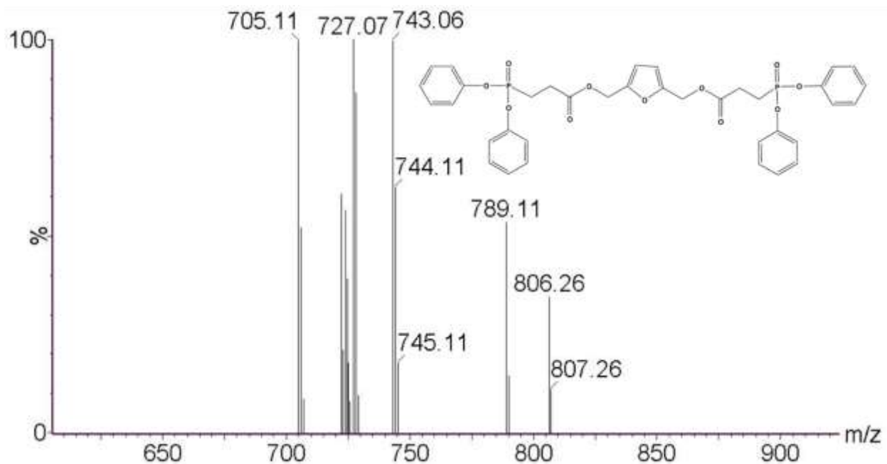
Figure S38. The ESI Mass Spectrum for Di[(3-diphenylphosphonatopropanoyl)methyl]furan (DPMF)
