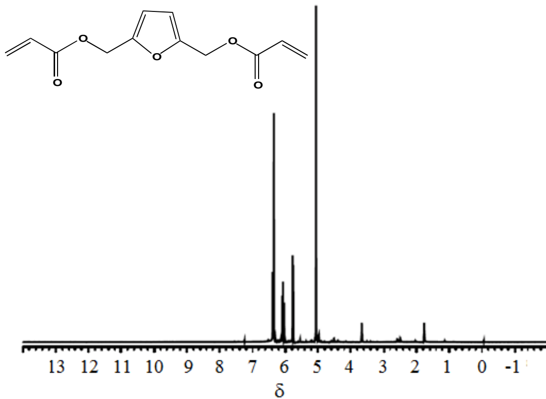
Figure S20. The 1 H NMR Spectrum for 2,5-bis-(Hydroxymethyl)furan Diacrylate (BHFDA)
