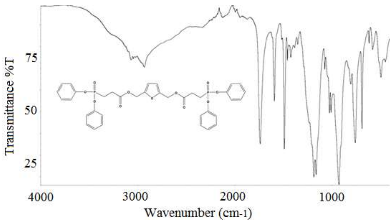
Figure S37. The Infrared Spectrum for Di[(3-diphenylphosphonatopropanoyl)methyl]furan (DPMF)
