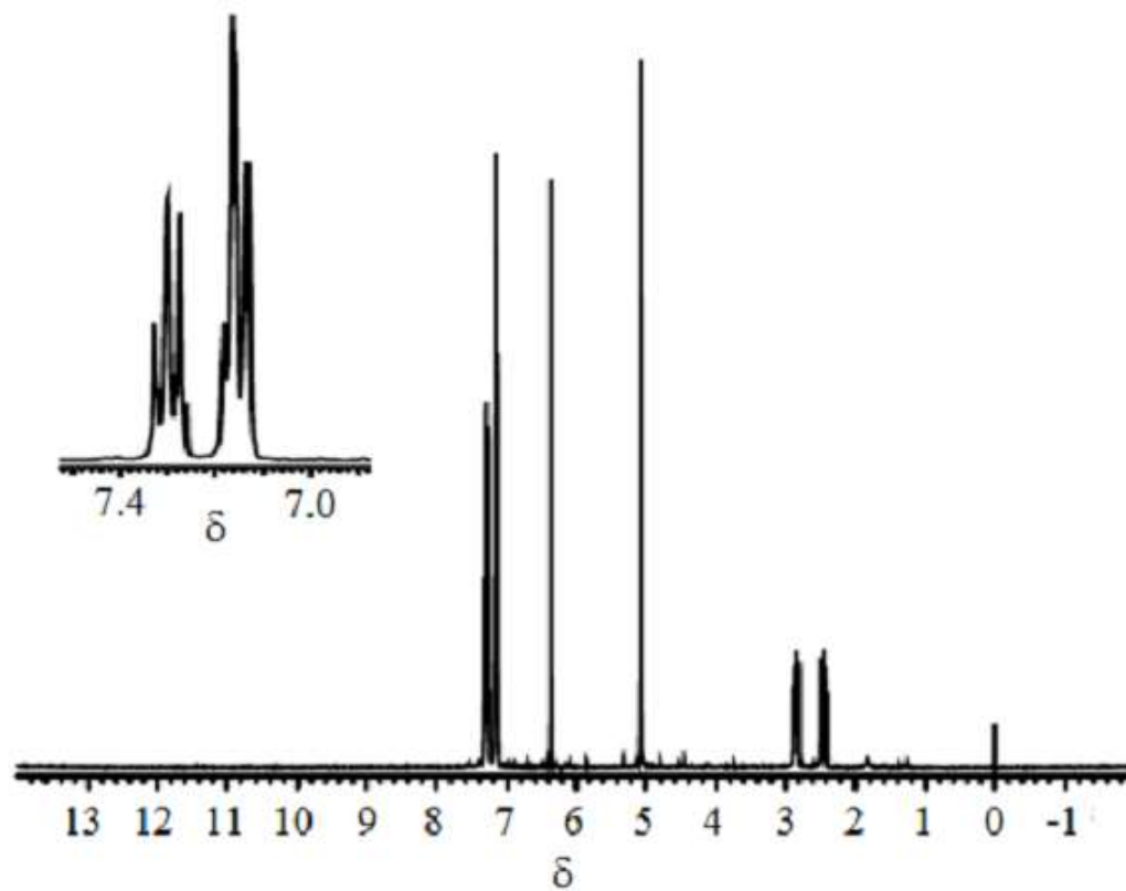
Figure S35. The ^1\text{H} NMR Spectrum for Di[(3-diphenylphosphonatopropanoyl)methyl]furan (DPMF)
