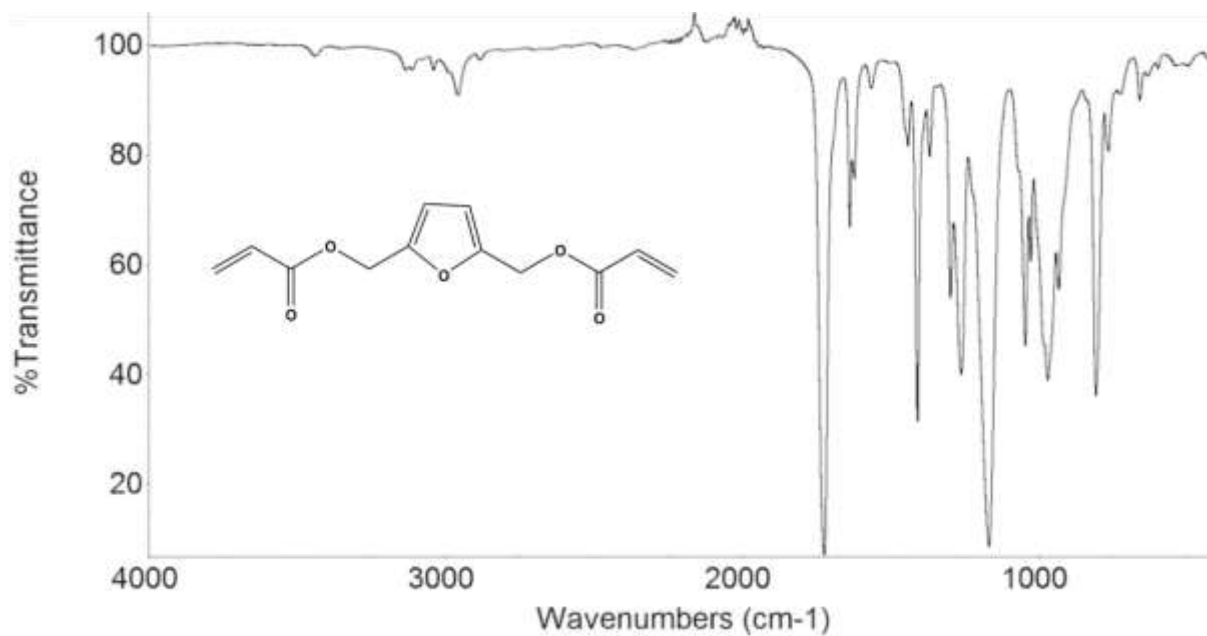
Figure S22. The Infrared Spectrum for 2,5- bis -(Hydroxymethyl)furan Diacrylate (BHFDA)
