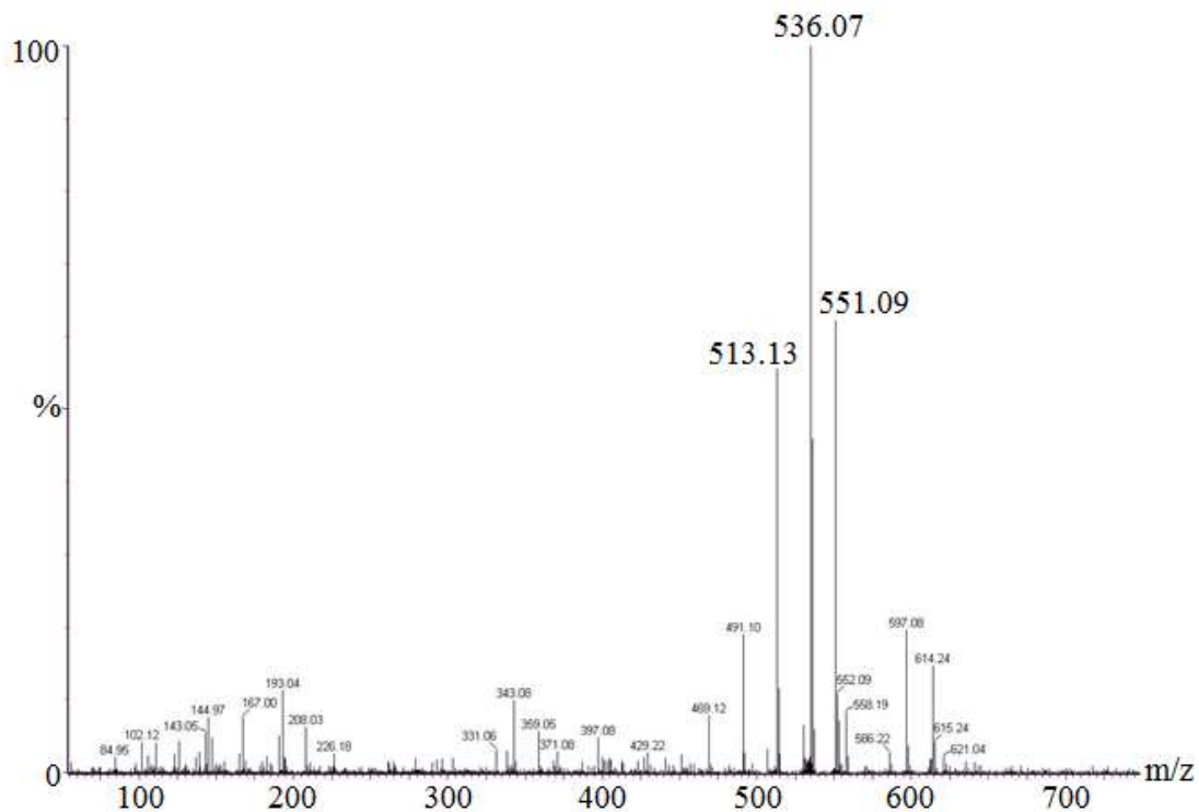
Figure S34. The ESI Mass Spectrum of Di[(3-diethylphosphonatopropanoyl)methyl]furan (DEMF)
