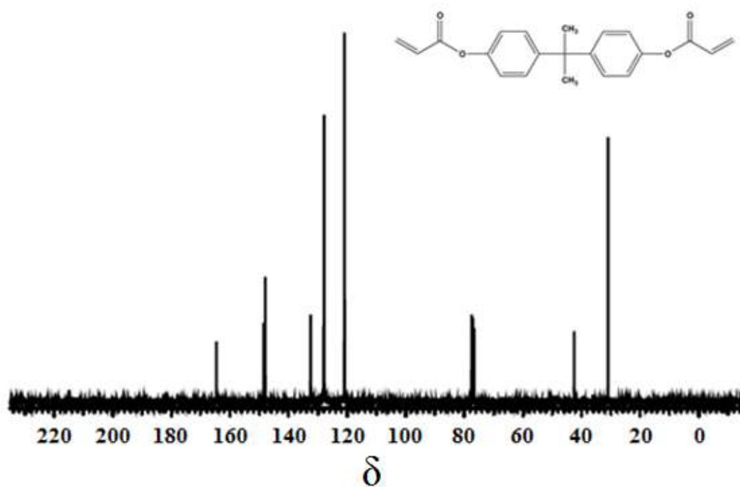
Figure S2. The ^{13}\text{C} NMR Spectrum for Bisphenol A Diacrylate (BPADA)
