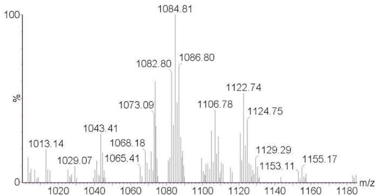
Figure S19. The ESI Mass Spectrum of 2,2-Di[3,5-dibromo-4-(3-dopylpropanoyl)phenyl]propane (DBDPP).
