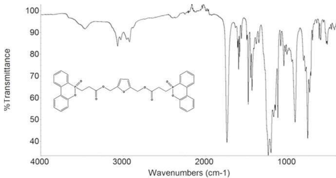
Figure S29. The Infrared Spectrum of 2,5-Di[(3-dopylpropanoyl)methyl]furan (DDMF)
