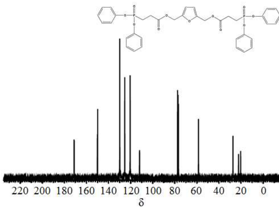
Figure S36. The 13 C NMR Spectrum for Di[(3-diphenylphosphonatopropanoyl)methyl]furan (DPMF)
