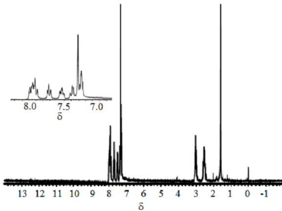
Figure S13. The ^1\text{H} NMR Spectrum 2,2-Di[3,5-dibromo-4-(3-dopylpropanoyl)phenyl]propane (DBDPP)
