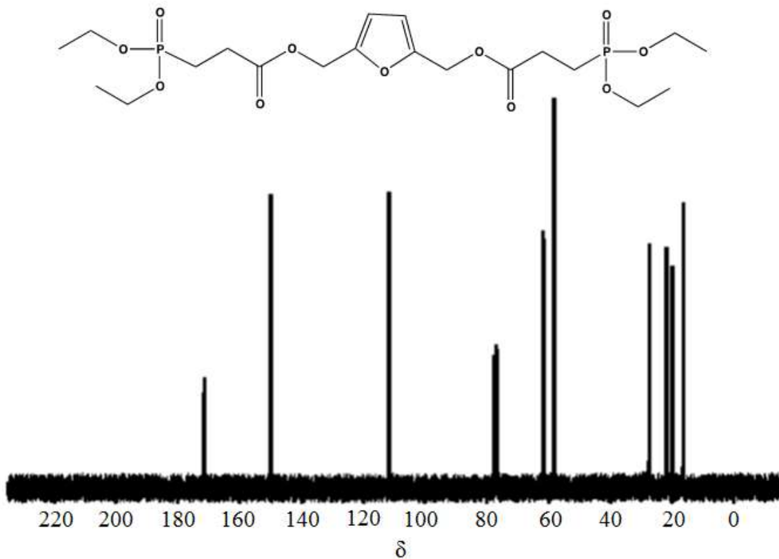
Figure S32. The 13 C NMR Spectrum for Di[(3-diethylphosphonatopropanoyl)methyl]furan (DEMF)
