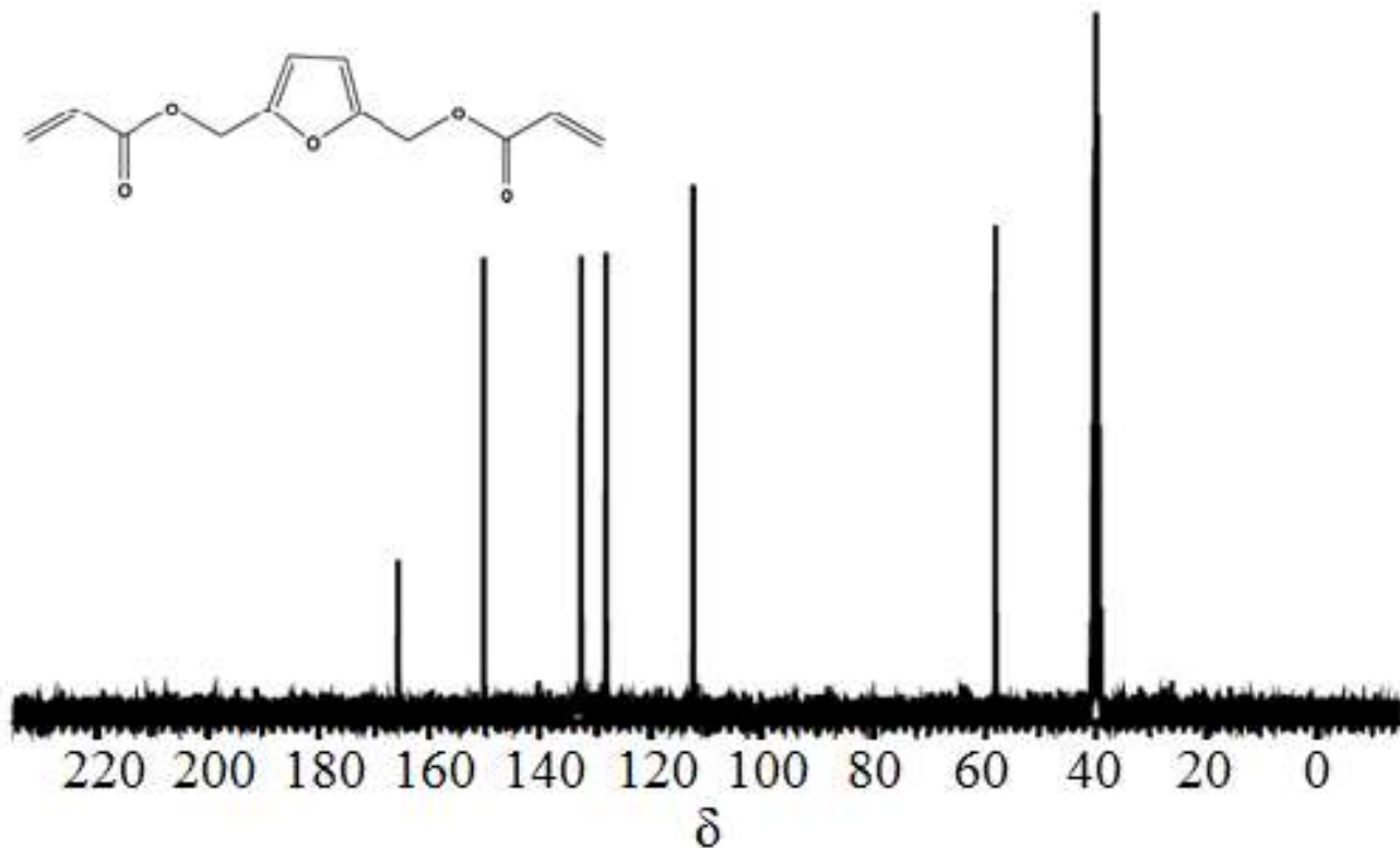
Figure S21. The 13 C NMR Spectrum for 2,5- bis -(Hydroxymethyl)furan Diacrylate (BHFDA)
