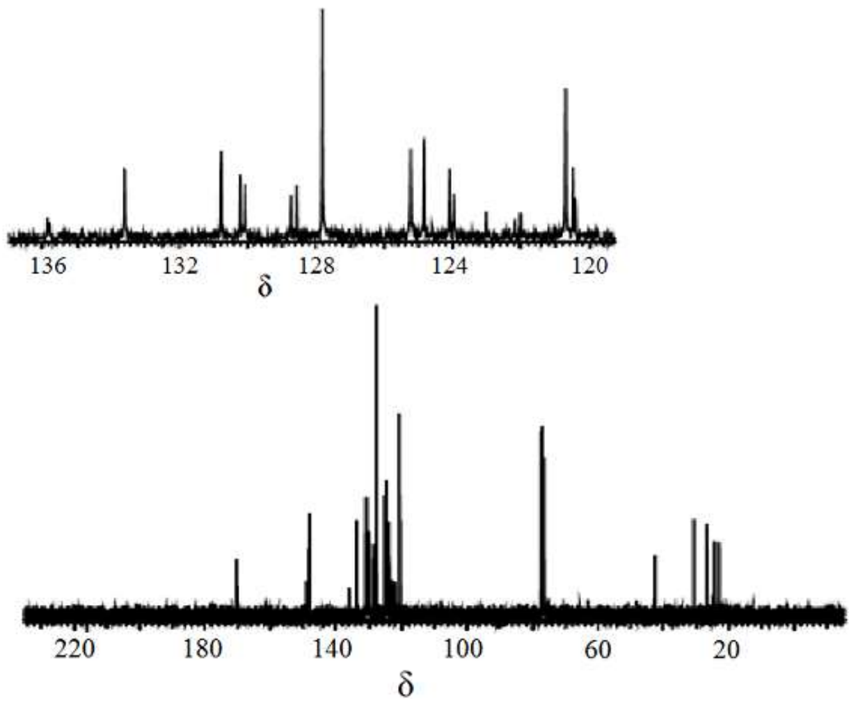
Figure S5. The ^{13}\text{C} NMR Spectrum of 2,2-Di[4-(3-dopylpropanoyl)phenyl]propane (DDPP)
