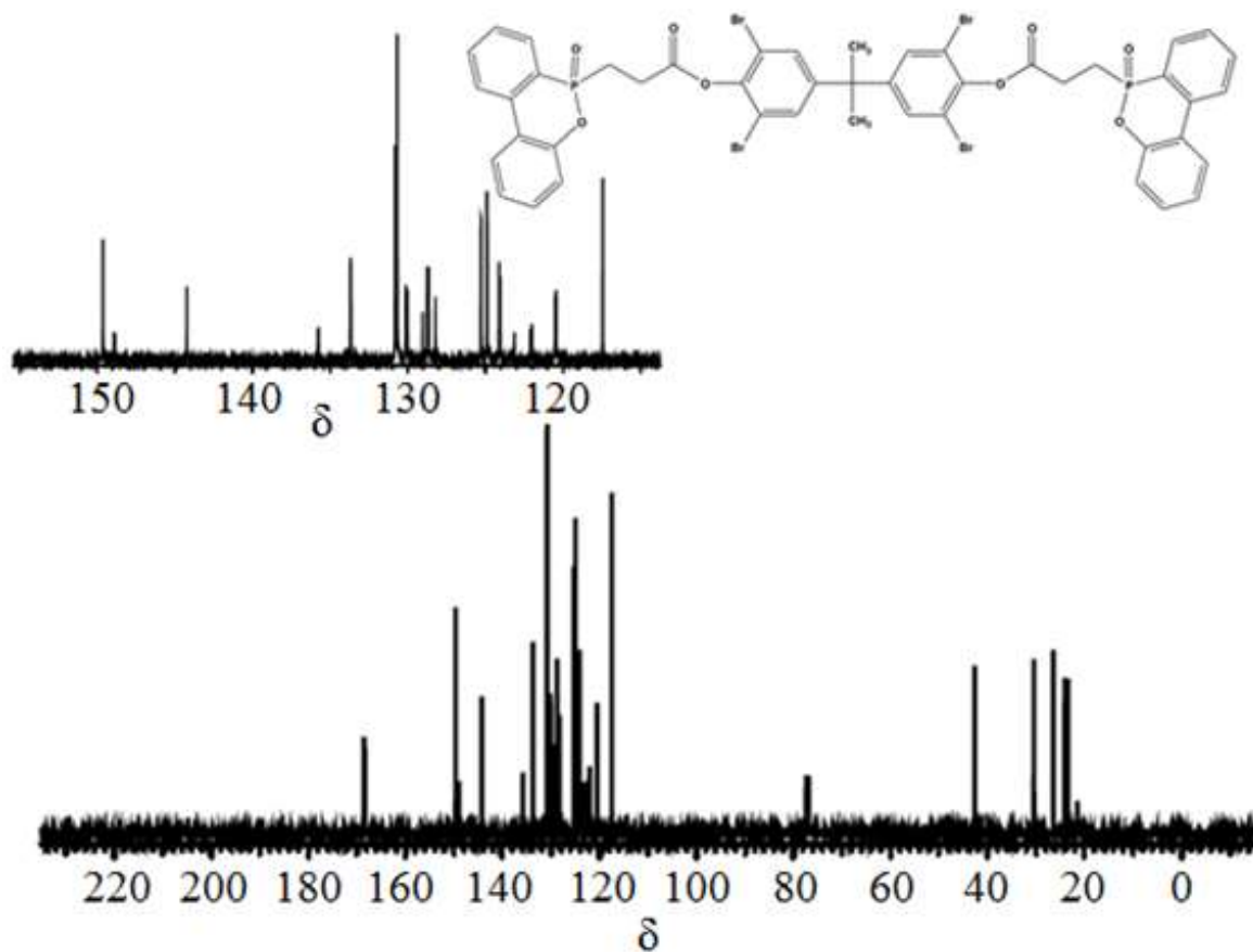
Figure S16. The ^{13}\text{C} NMR Spectrum for 2,2-Di[3,5-dibromo-4-(3-dopylpropanoyl)phenyl]propane (DBDPP).
