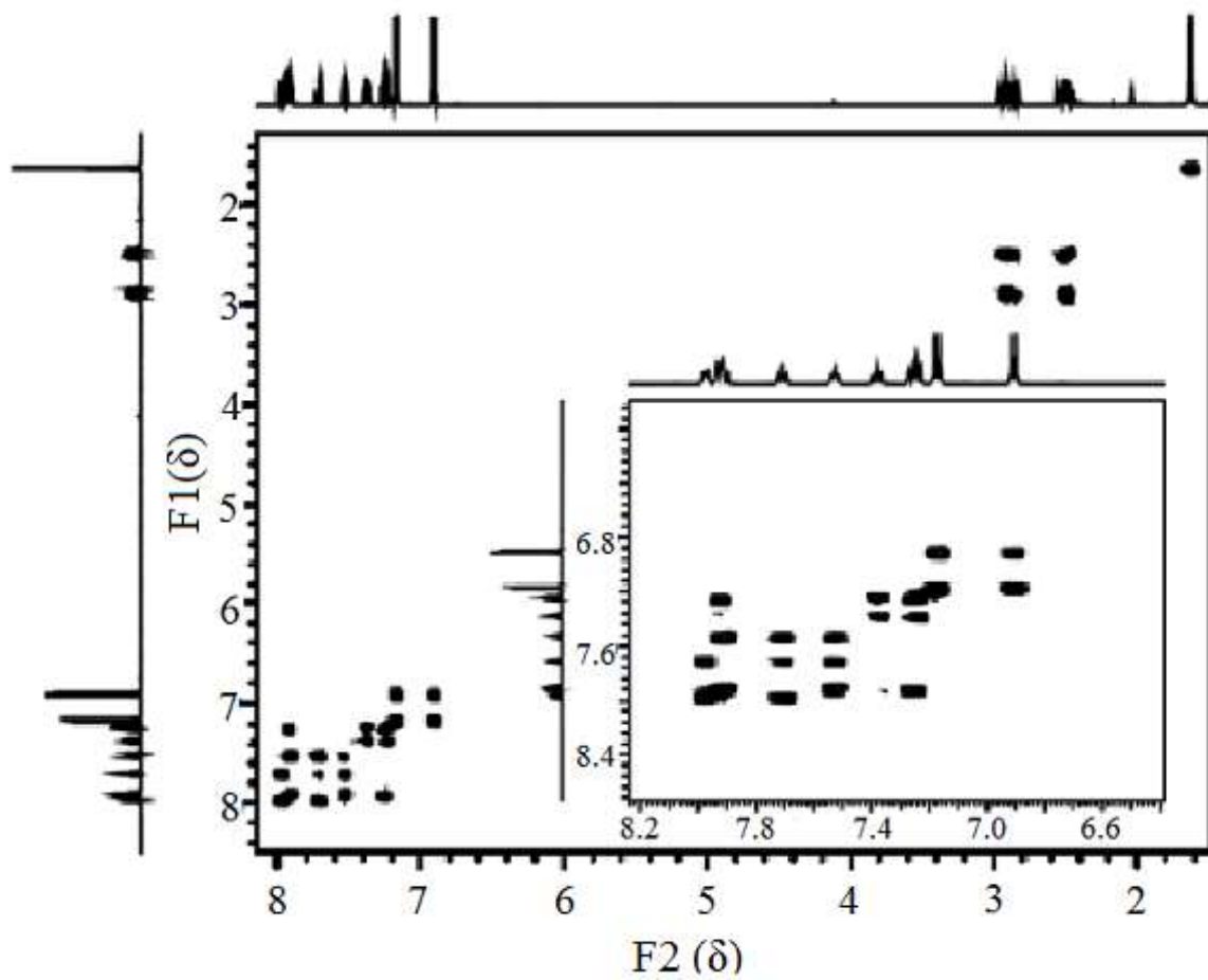
Figure S7. The gCOSY NMR Spectrum of 2,2-Di[4-(3-dopyl)propanoyl]phenyl]propane (DDPP)
