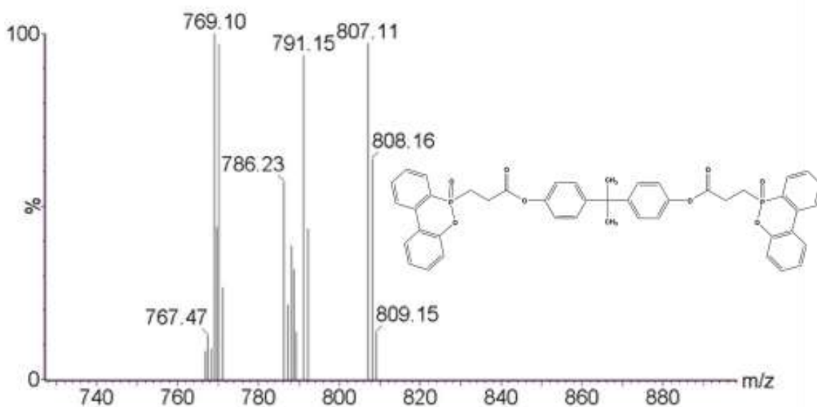
Figure S9. ESI Mass Spectrum of 2,2-Di[4-(3-dopylpropanoyl)phenyl]propane (DDPP)
