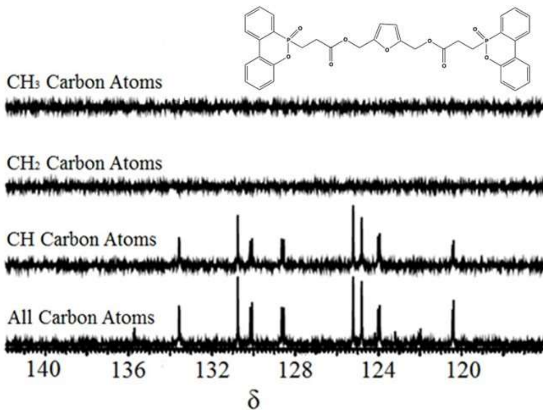
Figure S27. The DEPT NMR Spectrum for 2,5-Di[(3-dopylpropanoyl)methyl]furan (DDMF)
