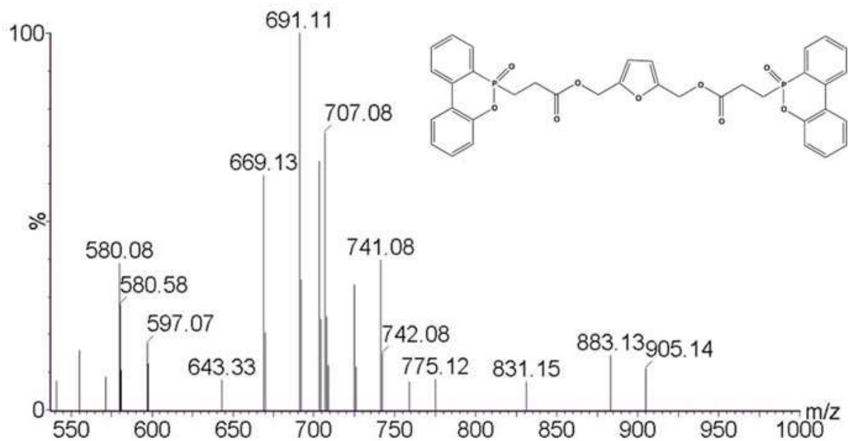
Figure S30. The ESI Mass Spectrum of 2,5-Di[(3-dopylpropanoyl)methyl]furan (DDMF)
