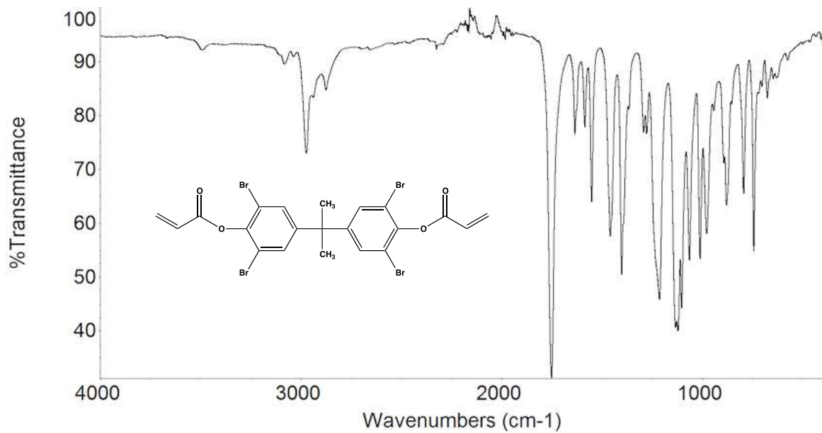
Figure S12. The Infrared Spectrum of of Tetrabromobisphenol A Diacrylate (BBPADA)
