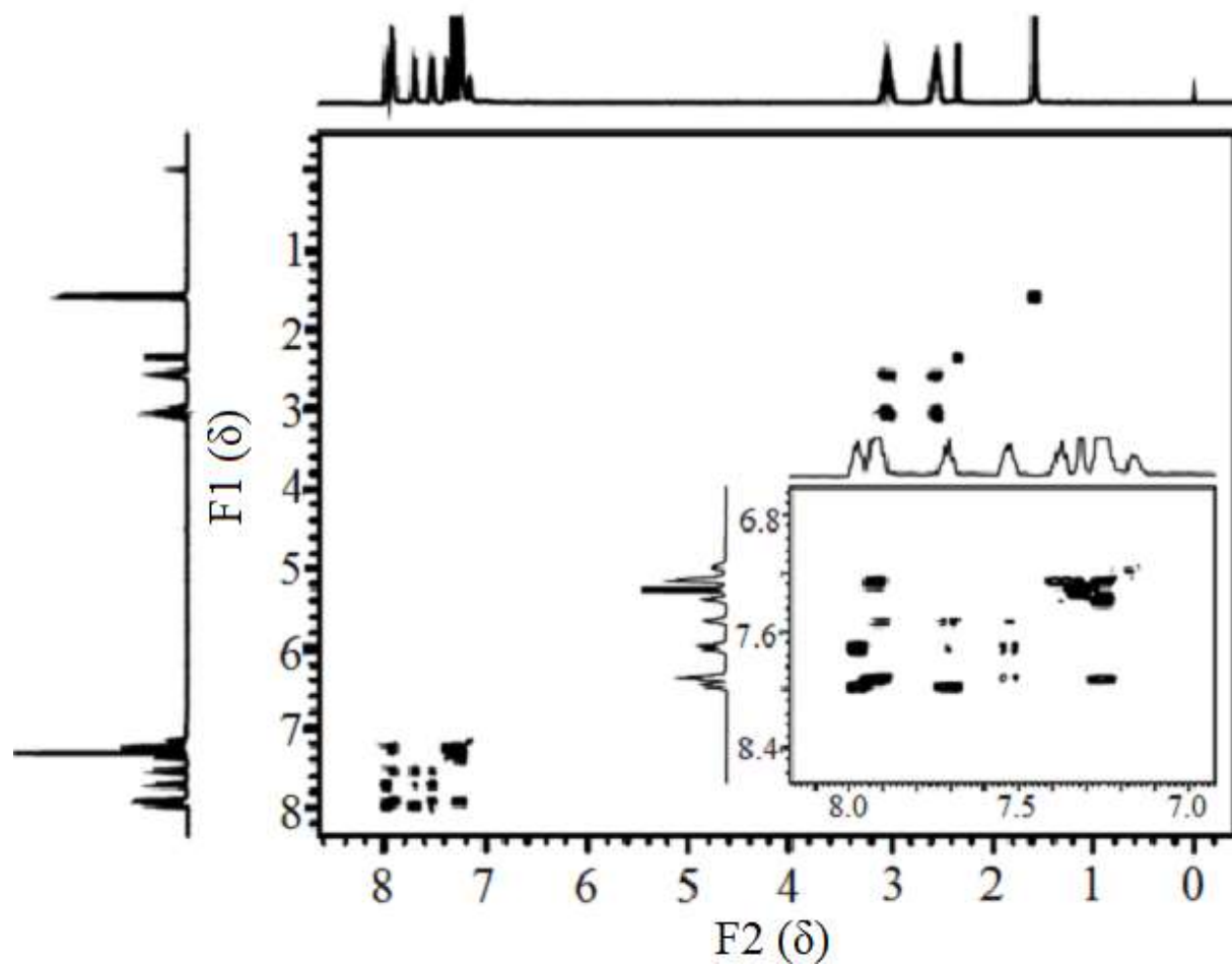
Figure S14. The gCOSY NMR Spectrum for 2,2-Di[3,5-dibromo-4-(3-dopylpropanoyl)phenyl]propane (DBDPP).
