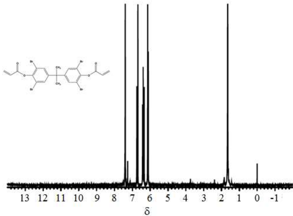
Figure S10. The 1 H NMR Spectrum for Tetrabromobisphenol A Diacrylate (BBPADA)
