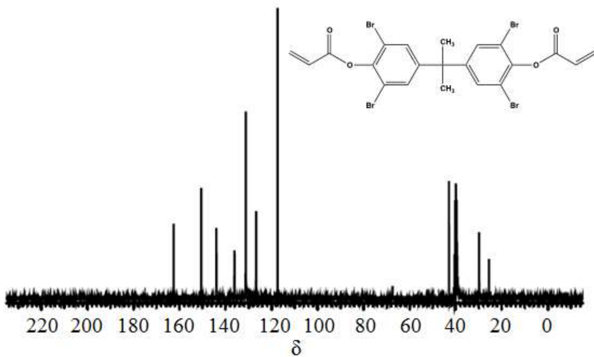
Figure S11. The 13 C NMR Spectrum for Tetrabromobisphenol A Diacrylate (BBPADA)
