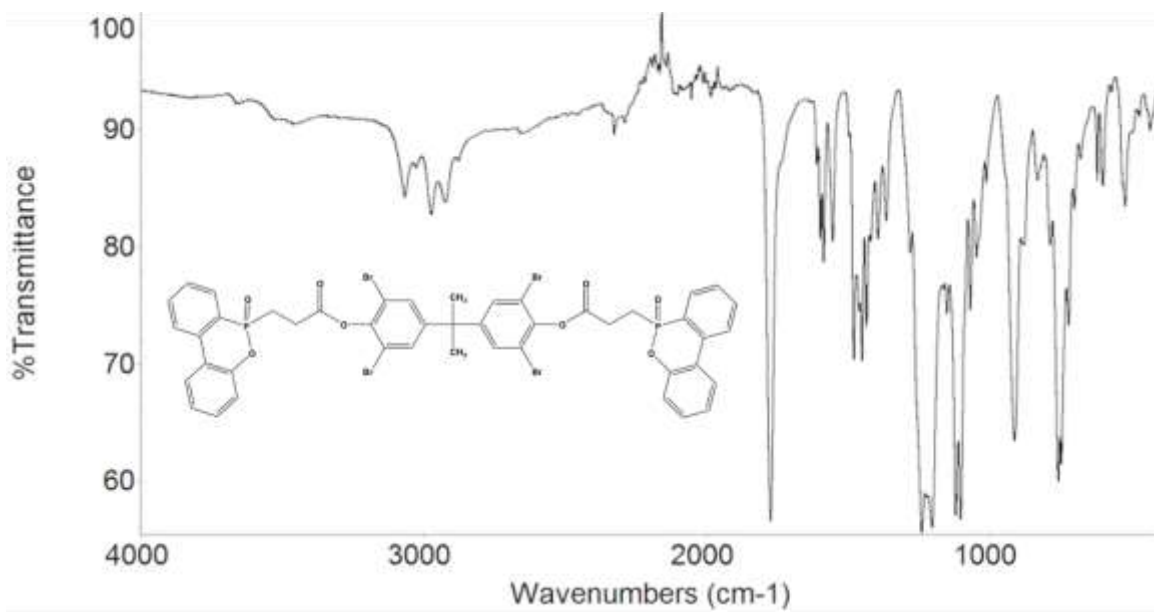
Figure S18. The Infrared Spectrum of 2,2-Di[3,5-dibromo-4-(3-dopylpropanoyl)phenyl]propane (DBDPP).
