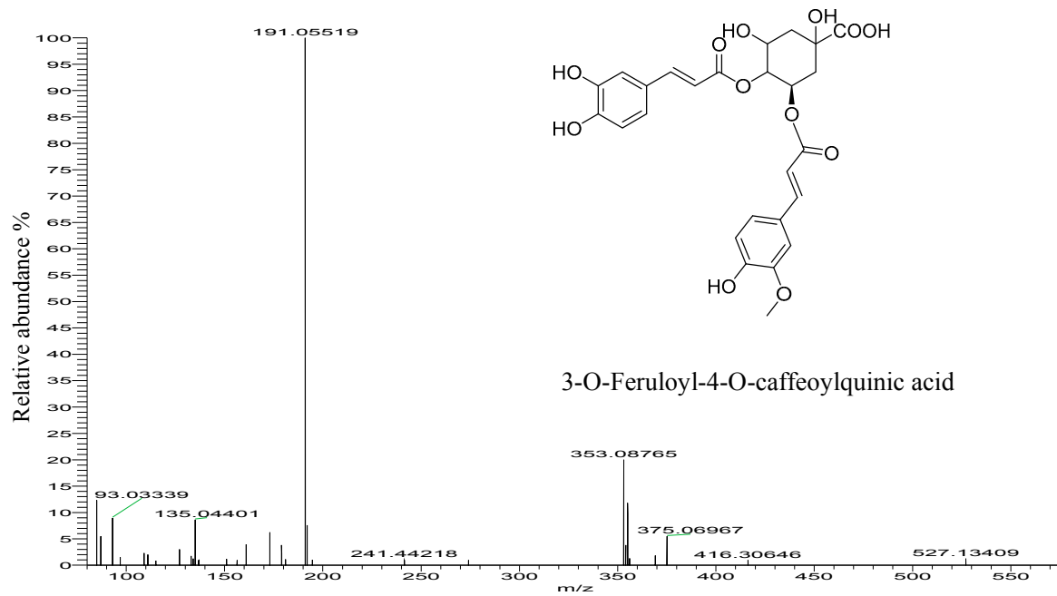
Supplementary Figure S1. MS/MS mass spectra of investigated compounds ( n = 15 ) extracted of coffee silverskin produced by roasting coffee beans ( Coffea arabica L.).
