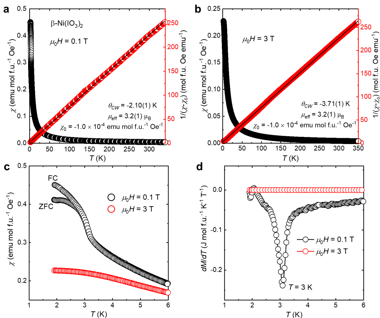
Figure 5. (a,b) (Black) magnetic susceptibility of \beta\text{-Ni}(\text{IO}_3)_2 measured from T = 2\text{ K} – 300\text{ K} at (a) \mu_0 H = 0.1\text{ T} and (b) \mu_0 H = 3\text{ T} . (red) Curie–Weiss fitting of 1/(\chi - \chi_0) against temperature for the paramagnetic phase. (c) Zero-field-cooled (ZFC) and field-cooled (FC) magnetic susceptibilities of \beta\text{-Ni}(\text{IO}_3)_2 as a function of temperature at different magnetic field. (d) First derivative of magnetization with respect to the temperature, dM/dT vs. T for \beta\text{-Ni}(\text{IO}_3)_2 .
