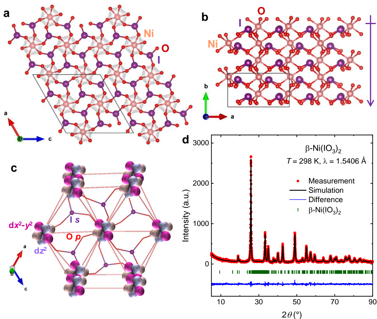
Figure 2. (a,b) Crystal structure of \beta -Ni(IO 3 ) 2 consisting of corner-sharing NiO 6 octahedra and IO 3 trigonal pyramid; the polar symmetry of \beta -Ni(IO 3 ) 2 results from the alignment of (IO 3 ) − local dipole along the b axis. (c) Atomic connectivity and orbital overlap in \beta -Ni(IO 3 ) 2 . (d) Rietveld refinements of XRD data of polycrystalline \beta -Ni(IO 3 ) 2 .
