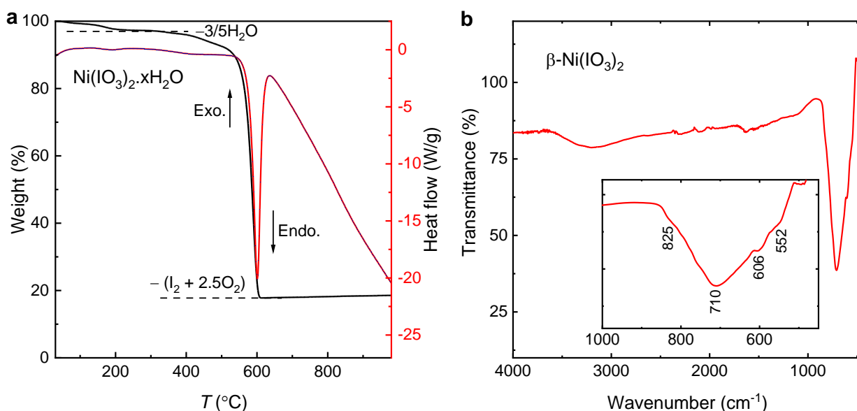
Figure 1. (a) Thermogravimetric analysis (TGA) and differential scanning calorimetry (DSC) of \beta\text{-Ni}(\text{IO}_3)_2/\text{Ni}(\text{IO}_3)_2 \cdot 2\text{H}_2\text{O} showing loss of 3/5\text{H}_2\text{O} of crystallization at T \approx 60\text{--}200\text{ }^\circ\text{C} and a decomposition temperature of 523\text{ }^\circ\text{C} accompanied by the loss of \text{I}_2 and 2.5\text{O}_2 . (b) FTIR of \beta\text{-Ni}(\text{IO}_3)_2 showing four absorption bands corresponding to four fundamental I–O vibrations expected for \text{IO}_3 group in \text{C}_{3v} symmetry \Gamma_{\text{vib}} = 2\text{A}_1 + 2\text{E} .
