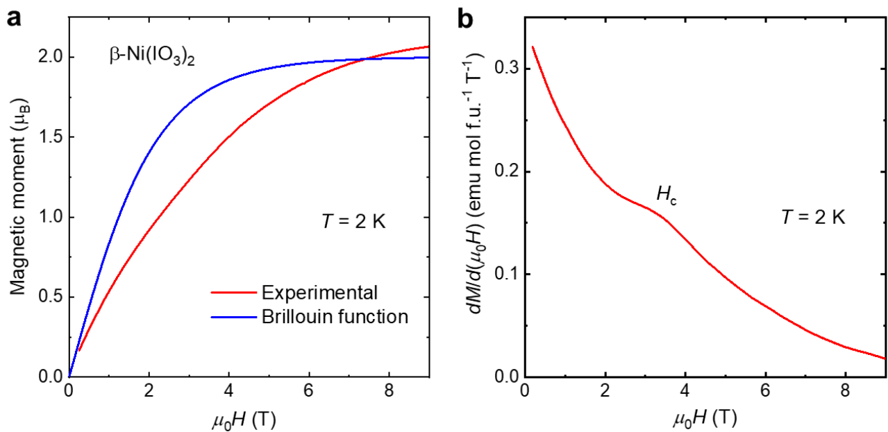
Figure 6. (a) (red) M(H) data of \beta\text{-Ni}(\text{IO}_3)_2 in \mu_B at T = 2\text{ K} , (blue) Brillouin function for J = 1 and T = 2\text{ K} . (b) dM/dH curve for \beta\text{-Ni}(\text{IO}_3)_2 , showing critical field H_c at \sim 3\text{ T} .
