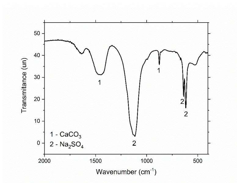
Figure S2. FTIR spectrum for efflorescence on 28 d 5NC pastes.
