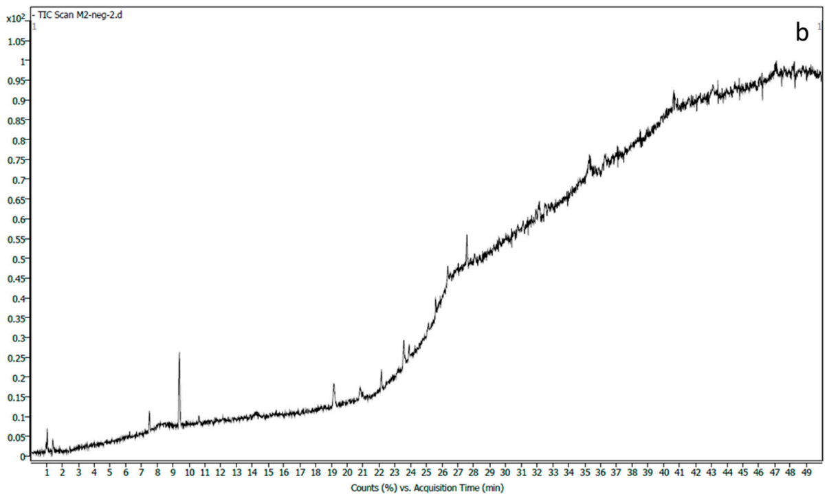
Figure S1. Full LC-MS chromatograms of MT-MAE-W/E (a) and MT-Ma-W/E (b) in negative ion mode of analysis.
