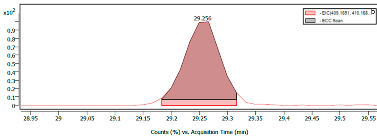
Figure S2. LC-MS chromatograms resending \alpha -mangostin of MT-MAE-W/E (a) and MT-Ma-W/E (b).
