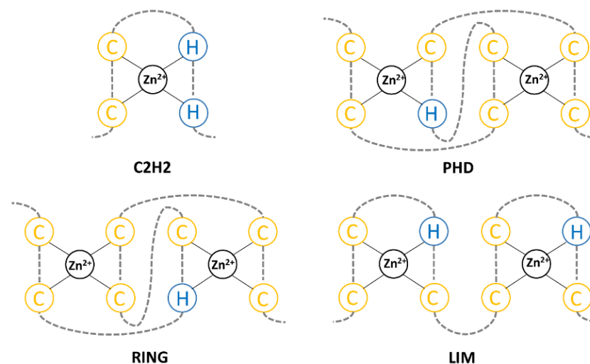
Figure 2. Scheme of C2H2, PHD, RING, and LIM zinc-finger domains.
