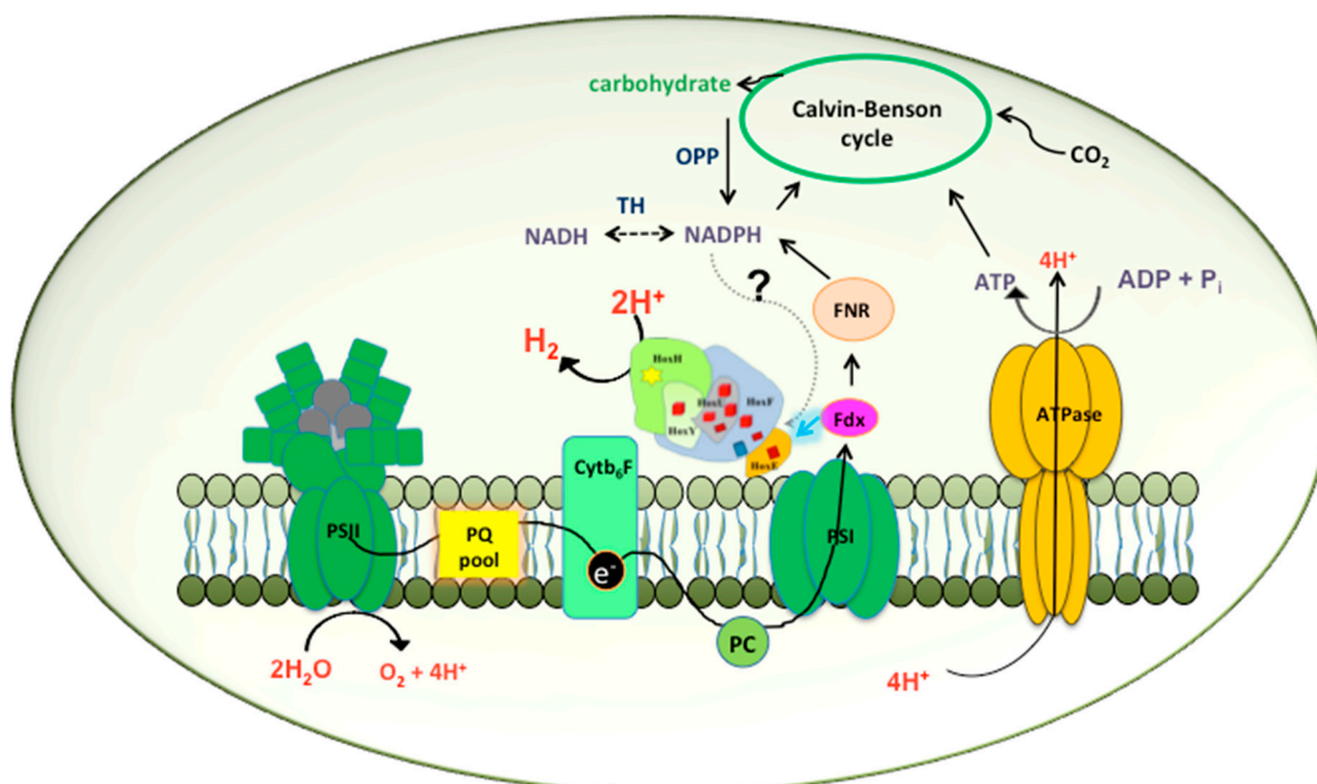
Figure 1. Biochemistry of hydrogen production in Synechocystis PCC 6803 by direct biophotolysis. In this pathway the reducing equivalents are obtained directly from the splitting of water at PSII. The electrons are transferred into the photosynthetic electron transport chain through a series of transport molecules including plastoquinone (PQ), cytochrome b 6 f (Cyt b 6 f) and plastocyanin (PC), and move through photosystem I (PSI) to reduce ferredoxin (Fdx) which goes on to reduce NADP + to NADPH via the enzyme ferredoxin NADP + reductase (FNR). At the same, time the reduced ferredoxin also has the capacity to directly donate the electrons to the Hox hydrogenase indicated by the
