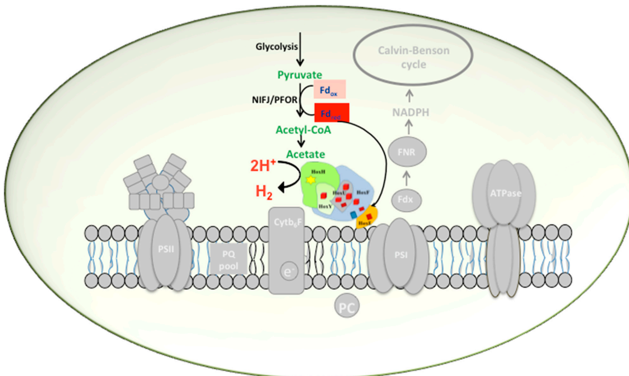
Figure 2. Biochemistry of hydrogen production in Synechocystis PCC 6803 by indirect biophotolysis. In darkness, under anaerobiosis, when the PSII is inactivated, glycogen is catabolized to pyruvate by glycolysis. Pyruvate is further oxidized to acetyl CoA during which ferredoxin is reduced by pyruvate formate oxidoreductase (PFOR). Reduced ferredoxin has the capacity to directly donate electrons to the Hox hydrogenase.
