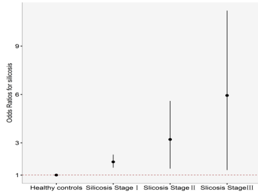
Figure S1 The relationships between HMGB-1 and the stage of silicosis. Model adjusted for age (continuous), BMI (continuous), smoking status (no, yes), drinking status (no, yes), passive smoker (no, yes).
